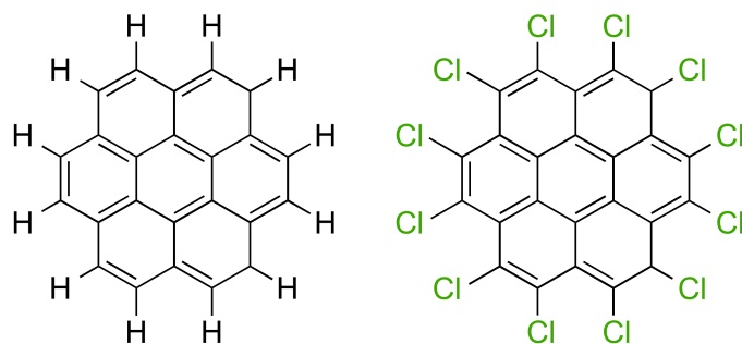
Figure 9.1: Molecular structures of coronene ( C_{24}H_{12} ) on the left and perchlorocoronene ( C_{24}Cl_{12} ) on the right.
