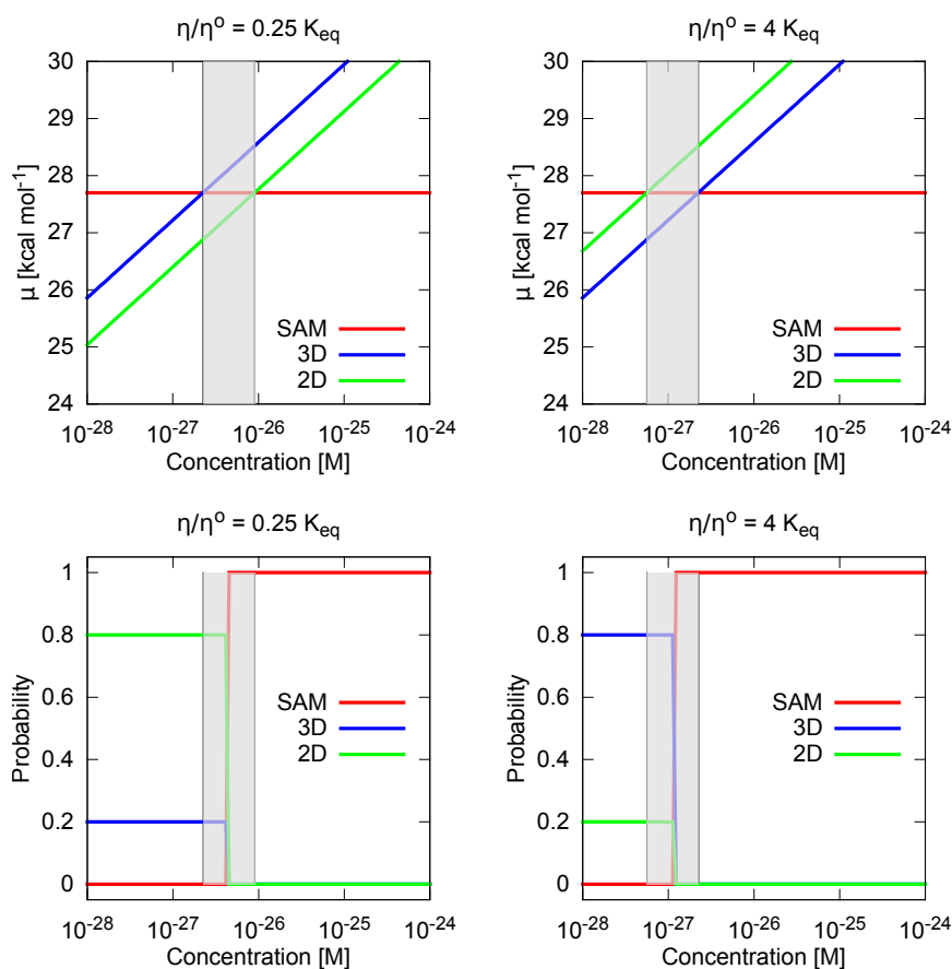
Figure 10.6: Chemical potential (top row) and equilibrium probabilities (bottom row) of A_{2D} , A_{3D} and the SAM as a function of the initial concentration. Two examples are depicted: \eta < K_{eq} (left) and \eta > K_{eq} (right). These examples refer to the adsorption equilibrium and self-assembly of trimesic acid (TMA) into the chickenwire (CHK) architecture. The chemical potentials are: \mu_{3D}^{\circ} = 64.0 \text{ kcal mol}^{-1} , \mu_{2D}^{\circ} = 56.8 \text{ kcal mol}^{-1} (calculated using Eq. 10.2 and 10.3) and \mu_{uc} = 27.7 \text{ kcal mol}^{-1} as calculated in chapter 5. The non-physical concentrations are due to the leaking of a proper treatment of the solvent effects.
