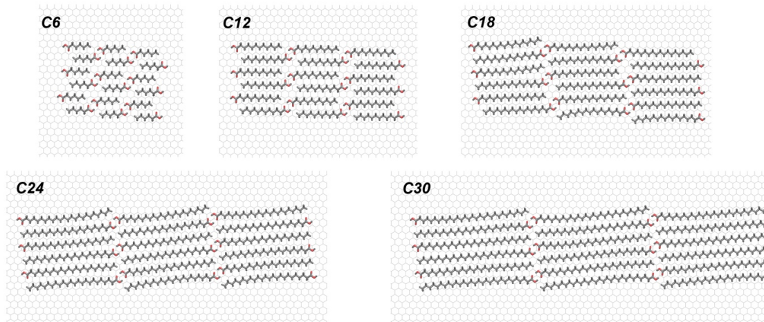
Figure 7.6: Molecular models for the five carboxylic acids.
