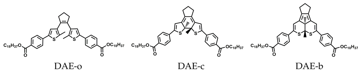
Figure 8.1: Chemical structure of the three form of the investigated diarylethene. From the left: the open (DAE-o), closed (DAE-c), and byproduct (DAE-b).
