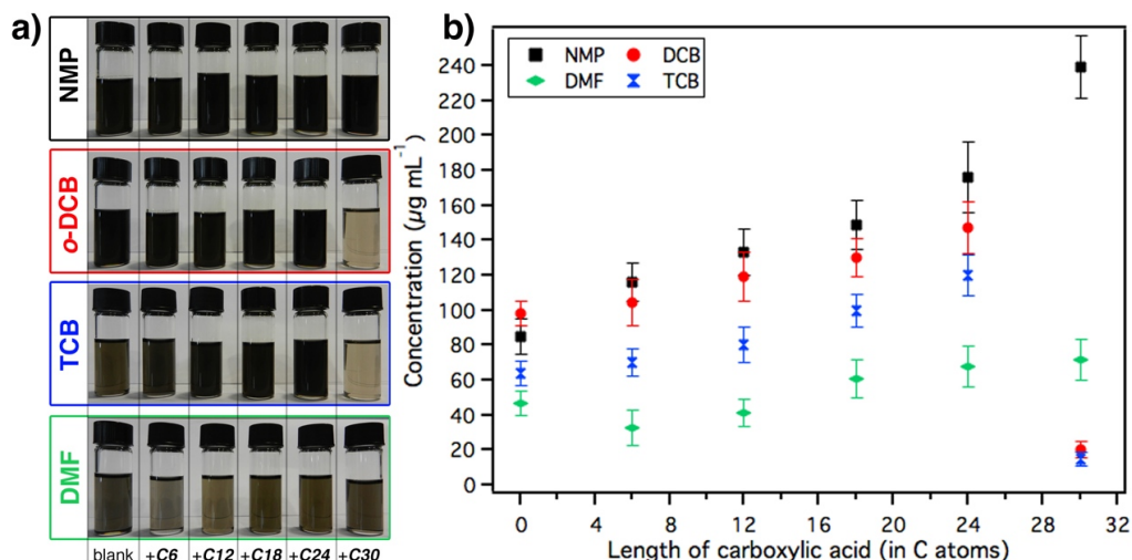
Figure 7.4: a) Photographs of the graphene dispersion obtained by LPE of graphite flakes in the four studied solvents and in the present of the five fatty acids. b) Concentration of the graphene dispersion; the error bars correspond to the standard deviation from 15 independent experiments.
