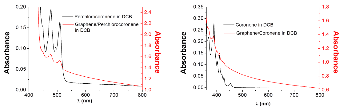
Figure 9.8: Comparison between the adsorbance spectra of the graphene dispersion obtained by the use of a surfactant (red curve), and the absorbance of the surfactants alone (black curve). The plot on the left refers to perchlorocoronene, on the right coronene.
