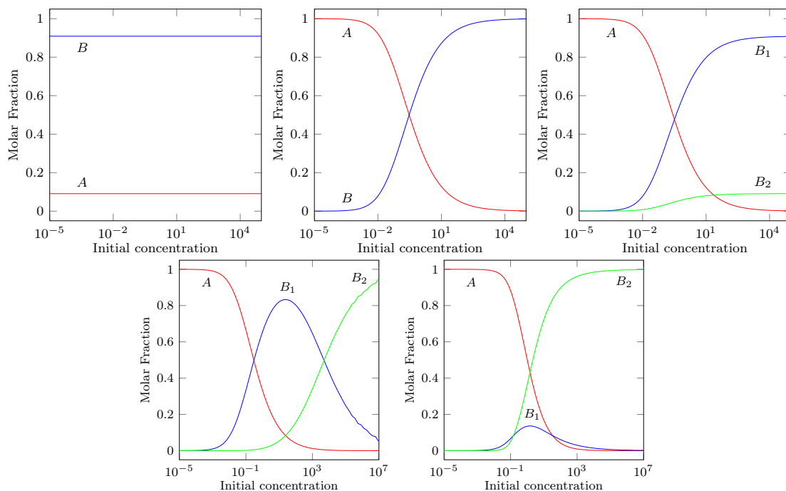
Figure 3.1: Molar fractions as a function of the initial concentration of A for different kind of equilibria.
