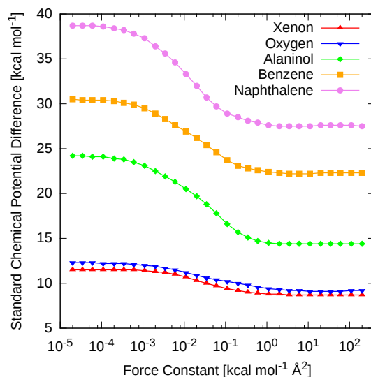
Figure 10.5: Standard chemical potential differences for the five studied systems as a function of the restraining force constant in the confinement simulations. All curves correctly converge for forces higher than 10 \text{ kcal mol}^{-1} \text{ \AA}^{-2} .
