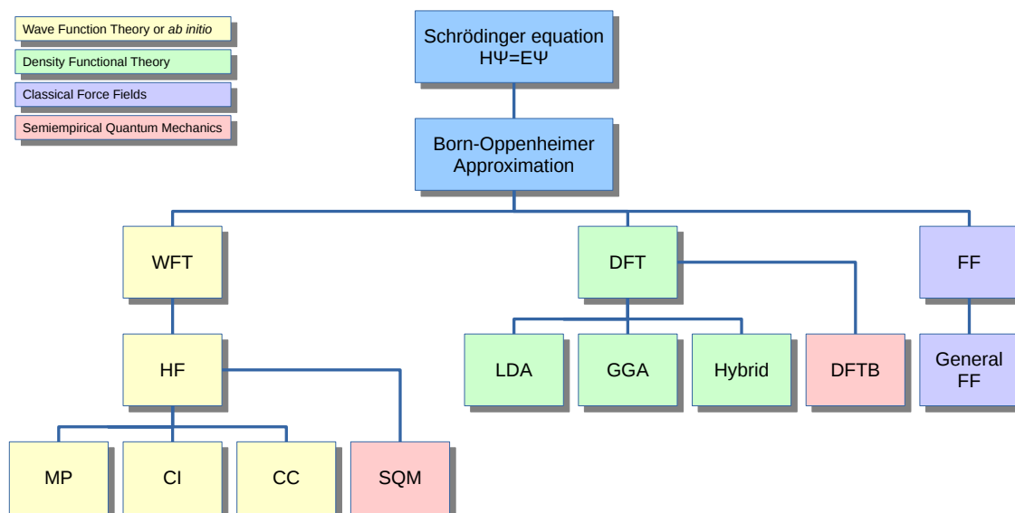
Figure 2.1: Overview of the computational methods briefly presented in this Chapter. The common root is the Schrödinger equation followed by the Born-Oppenheimer approximation. For this, three class of methods can be generated. First, the Wave Function Theory (WFT), which includes Hartree-Fock (HF), and the correlation-corrected Moller-Plesset (MP), Configuration Interaction (CI), and Coupled Cluster (CC). Second the Density Functional Theory (DFT) in its formulations: Local Density Approximation (LDA), Generalized Gradient Approximation (GGA), and Hybrid DFT. Third, the empirical Force Fields (FF), and their generalized extension. Last, the Semiempirical Quantum Mechanics (SQM) obtained from HF, and also from DFT (DFTB, not discussed in this work).
