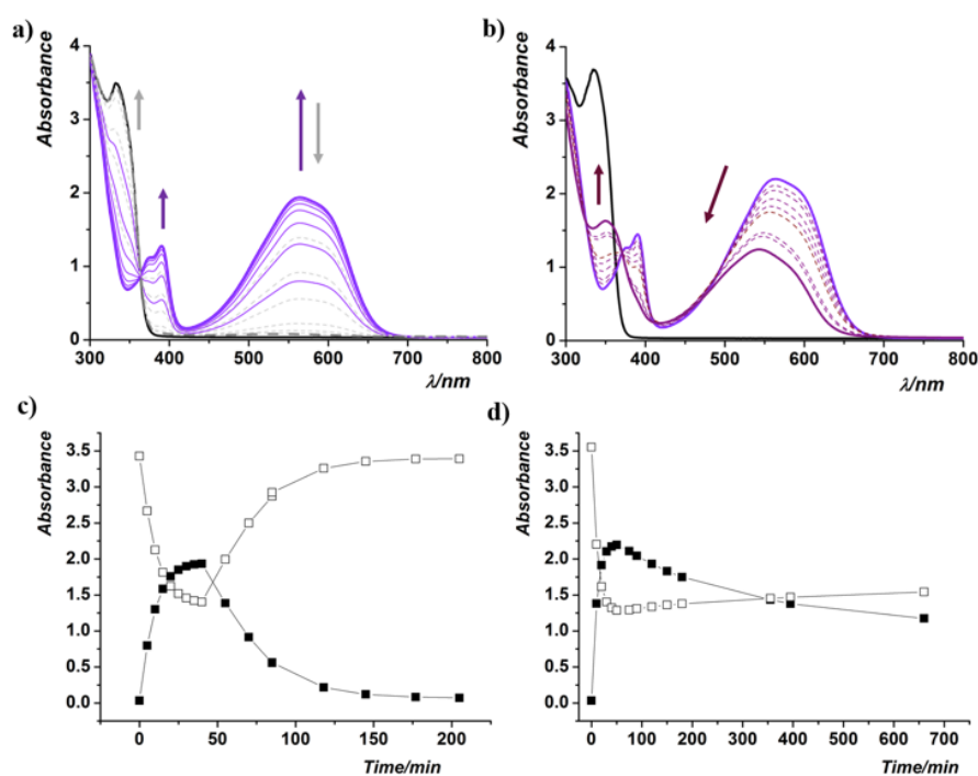
Figure 8.3: Photochromic behavior of DAE in solution followed by UV/Vis absorption spectroscopy. In a) reversible isomerization of the DAE-o (solid black) to the DAE-c (solid violet) by UV light, and back to the DAE-o (dashed black) by visible light. In b) irreversible conversion by UV light of the DAE-o (solid black) to the DAE-c (solid violet) and then to the DAE-b (solid pink). In c) and d) absorption changes at 330 nm and 560 nm (white and black squares, respectively) as a function of the irradiation time in the a) and b) studies.
