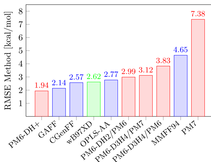
Figure 6.4: Root Mean Square Error (RMSE) of the tested computational methods relative to the experimental TPD data. All values are reported in \text{kcal mol}^{-1} . SQM are in red, force field in blue and DFT in green. Methods are ranked by RMSE.
