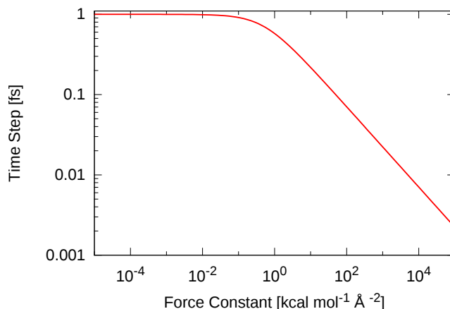
Figure E.1: Time step as a function of the force constant of the applied harmonic restrain.
