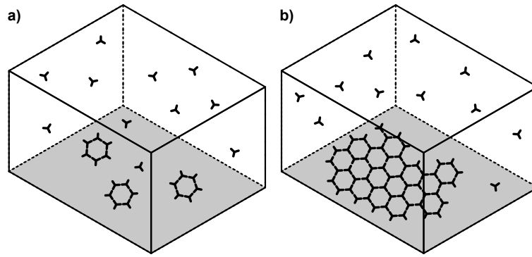
Figure 5.1: Schematic representation of the self-assembly at surfaces process. In a) the free molecules in solution are in equilibrium with finite-size object physisorbed at the solid-liquid interface. In b) the monomer in solution are in equilibrium with an extended periodic structure.
