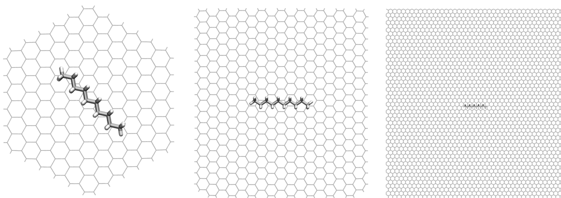
Figure 6.1: Models for the graphite substrate used in this work. On the left, the 216 hexagonal model used for the SQM and DFT methods. On the center, the 610 carbon atoms model used for the CGenFF force field. On the right, the 103 \times 110 Å periodic graphene layer used for the GAFF and OPLS-AA force fields. The model used for the MMFF94 force field is similar to this last, but with double size ( 206 \times 216 Å). As reference, the biggest molecule used in this work (decane) is represented at the center of each model.
