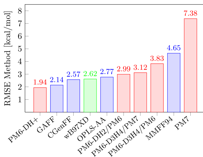
Figure 6.4: Root Mean Square Error (RMSE) of the tested computational methods relative to the experimental TPD data. All values are reported in kcal mol -1 . SQM are in red, force field in blue and DFT in green. Methods are ranked by RMSE.
