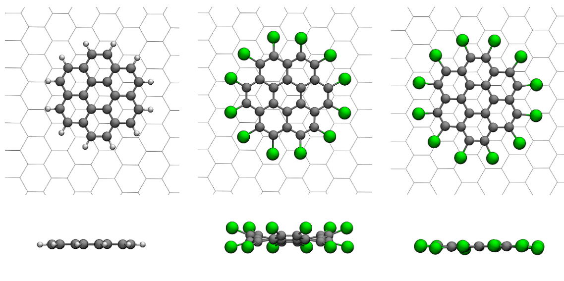
Figure 9.2: Top and side views of the optimized structures when adsorbed on graphene of coronene (left) and perchlorocoronene (center and right). For coronene only one structure is shown, that corresponds to the geometry obtained by both the CGenFF force field and the OM6-DH+ semiempirical method. For the perchlorocoronene the structures optimized at the two levels of theory are significantly different with the force field (center) producing a very distorted structure, while in the semiempirical (right) it is much more planar.
