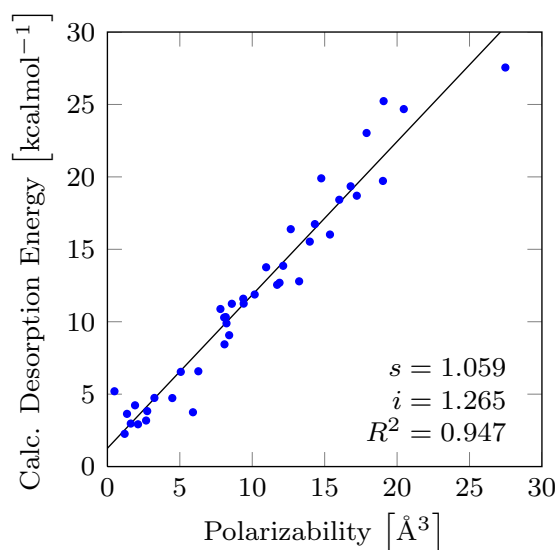
Figure 6.8: Correlation plot between the polarizability of a molecule and its desorption energy from graphene both calculated using the PM6-DH+ semiempirical method.
