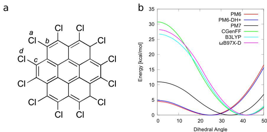
Figure 9.3: a) Chemical structure of perchlorocoronene. The four labeled atoms form the pseudo-dihedral used to evaluate the planarization cost; six of these dihedrals are present. b) Adiabatic energy profiles for the planarization of perchlorocoronene. In the minimum energy the molecule is not planar but presents a pseudo-dihedral angle of about 41^\circ when modeled with the reference DFT. When the pseudo-dihedral angle is forced to zero, the molecule is fully planar and the energy value represents the cost of planarization.
