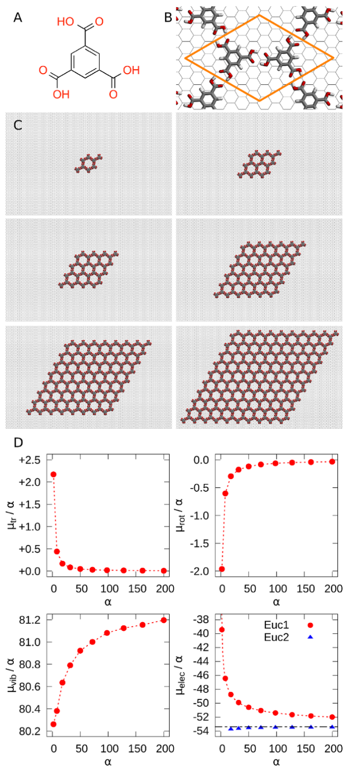
Figure 5.2: A) Chemical structure of trimesic acid (TMA, benzene-1,3,5-tricarboxylic). B) Unit cell of TMA in the chickenwire architecture. C) Six example supramolecules used to evaluate the limit of the chemical potential at increasing \alpha (8, 18, 32, 72, 128, and 200). D) Translational, rotational, vibrational and electronic contributions to the total chemical potential for supramolecule formed by \alpha TMA molecules when normalized by \alpha . All chemical potentials are reported in \text{kcal mol}^{-1} .
