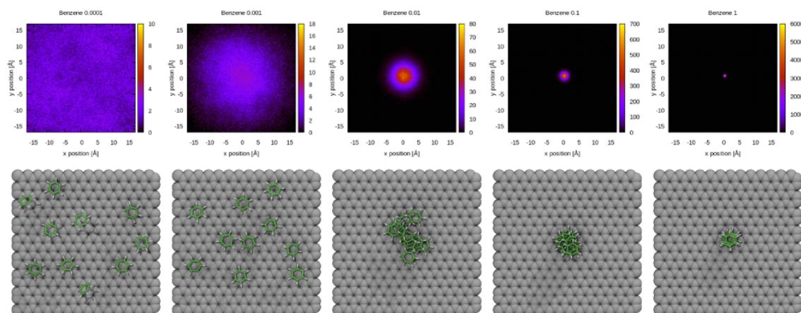
Figure 10.4: Top row: projection of the position of the center of mass of benzene on the graphene surface along the confinement simulations. Bottom row: ten superimposed frames from the confinement dynamics at each force constant. At low restraining force constants the whole surface is explored, while at higher forces the available surface is gradually confined.
