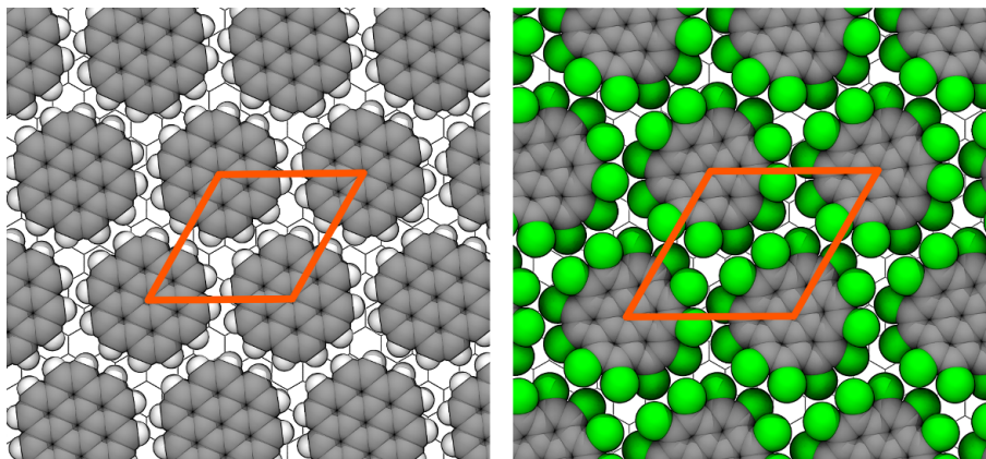
Figure 9.7: SAMs modeled for coronene (left) and perchlorocoronene (right) on graphene. Both architectures adopt a hexagonal unit cell of size of 11.32 Å and 12.89 Å, respectively, and an unit cell area of 110.88 Å 2 and 143.81 Å 2 .
