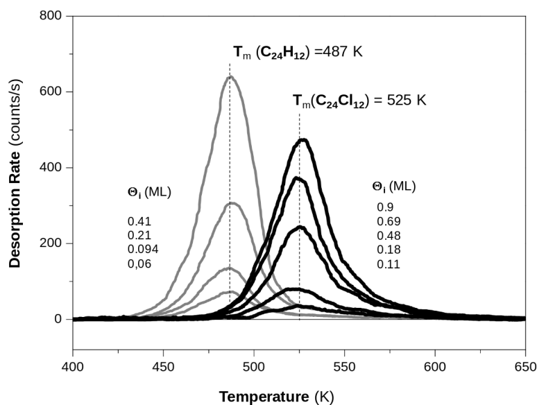
Figure 9.5: TPD spectra obtained at constant heating rate \beta = 2.5 \text{ Ks}^{-1} for several C_{24}H_{12} and C_{24}Cl_{12} samples at different submonolayer initial coverage \Theta_0 . The increase in the desorption temperature T_m from 487 K to 525 K indicates that perchlorination raises the binding energy.
