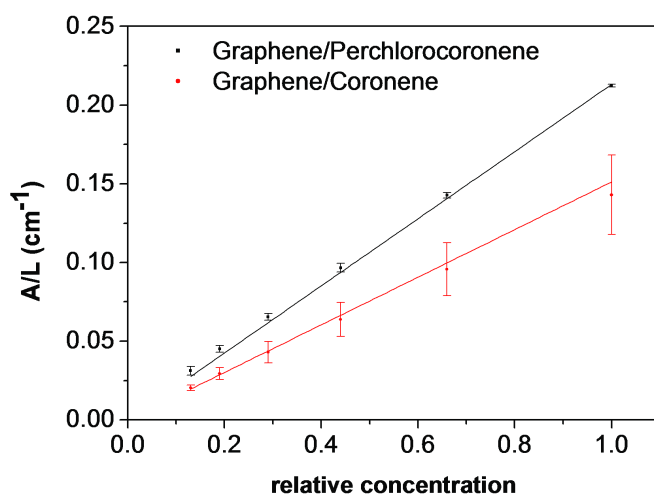
Figure 9.9: Absorbance at 660 nm upon dilution of the graphene dispersions obtained by coronene (red) and perchlorocoronene (black). From the slope of the linear interpolation, the concentration of graphene is determined.
