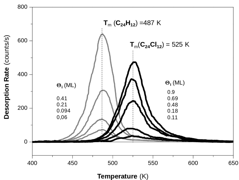
Figure 9.5: TPD spectra obtained at constant heating rate \beta = 2.5 \text{ K s}^{-1} for several \text{C}_{24}\text{H}_{12} and \text{C}_{24}\text{Cl}_{12} samples at different submonolayer initial coverage \Theta_0 . The increase in the desorption temperature T_m from 487 K to 525 K indicates that perchlorination raises the binding energy.
