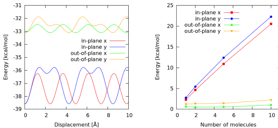
Figure 8.8: Left) Energy profiles obtained by displacing a C18 alkyl chain on a graphene surface along the x and y directions when adsorbed in the in-plane and out-of-plane zig-zag conformations. Right) Height of the energy barriers involved in the displaced in the x and y direction of a cluster of 1, 2, 5, and 10 molecules adsorbed in a in-plane and out-of-plane zig-zag conformation.
