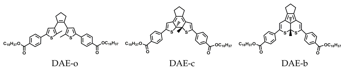
Figure 8.1: Chemical structure of the three form of the investigated diarylethene. From the left: the open (DAE-o), closed (DAE-c), and byproduct (DAE-b).
