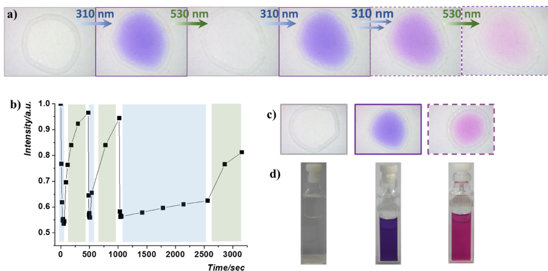
Figure 8.2: a) Bright-field images of a DAE drop on a quartz substrate during two UV/Visible irradiation cycles, with the formation of the DAE-b upon prolonged UV irradiation. b) Normalized intensity of the green RGB channel of the DAE drop during the photoconversion cycles in a). c) Bright-field images of DAE-o, DAE-c, DAE-b drops. d) Photos of DAE-o, DAE-c, DAE-b solutions in 2 mm quartz cuvettes.
