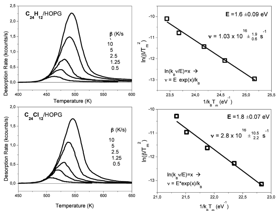
Figure 9.6: On the left, R(t) profiles at different heating rate \beta and, on the right, the linear plot obtained by graphing \ln(\beta/T_m^2) versus 1/k_B T_m . The top row refers to coronene with at initial coverage of 0.75 ML. The lower row refers to perchlorocoronene.
