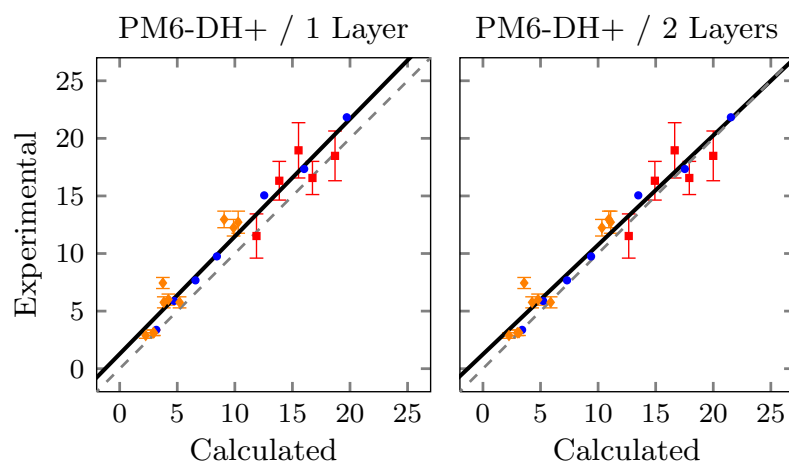
Figure 6.6: Correlation between the experimental and the calculated desorption energies evaluated using the PM6-DH+ semiempirical method using one (left) or two (right) graphene layers to model the graphite substrate.
