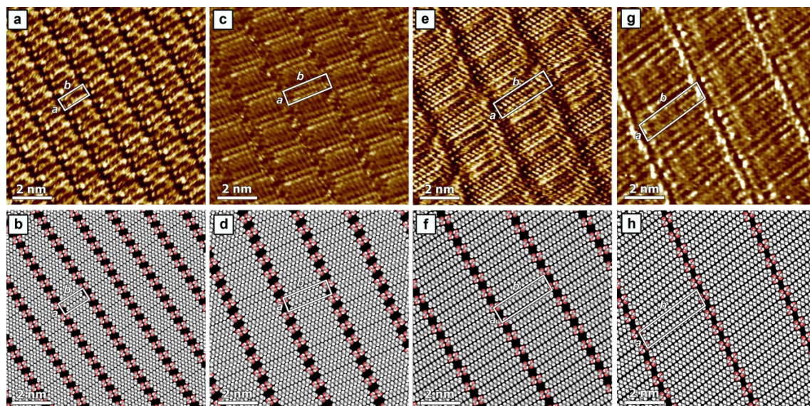
Figure 7.3: STM images (top row) and molecular models (bottom row) of the SAMs formed by the four molecules from C12 (left), to C30 (right). The shorted C6 does not show ordered SAMs.
