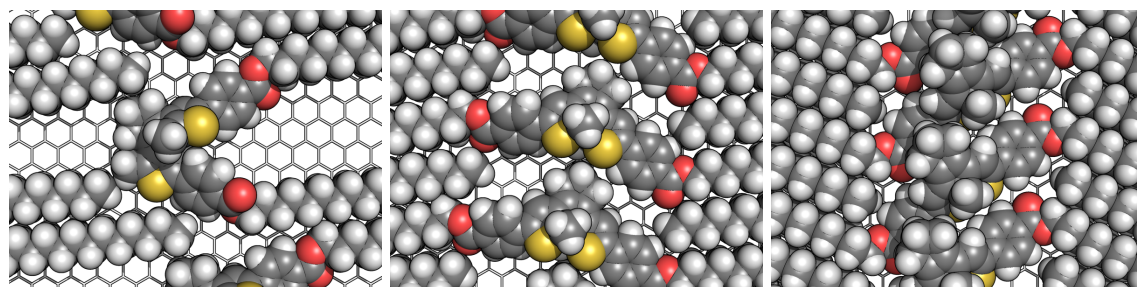
Figure 8.6: Magnification of the molecular models generated for the DAE-o (left), DAE-c (center), and DAE-b (right). Note how the alkyl chains are parallel in the DAE-o and antiparallel in the DAE-c and DAE-b, how the DAE-b is more dense than the DAE-c thanks to the different alkyl chain conformations, and the overlap of the cores of the molecules which is present only in the DAE-b.
