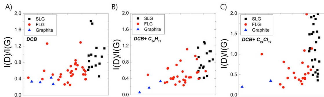
Figure 9.12: I(D)/I(G) ratio analysis of graphene dispersions in a) pure solvent (o-DCB), b) coronene, and c) perchlorocoronene.
