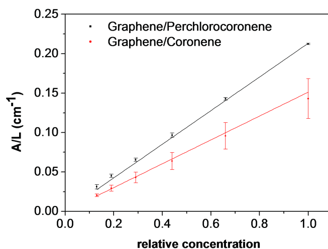
Figure 9.9: Absorbance at 660 nm upon dilution of the graphene dispersions obtained by coronene (red) and perchlorocoronene (black). From the slope of the linear interpolation, the concentration of graphene is determined.
