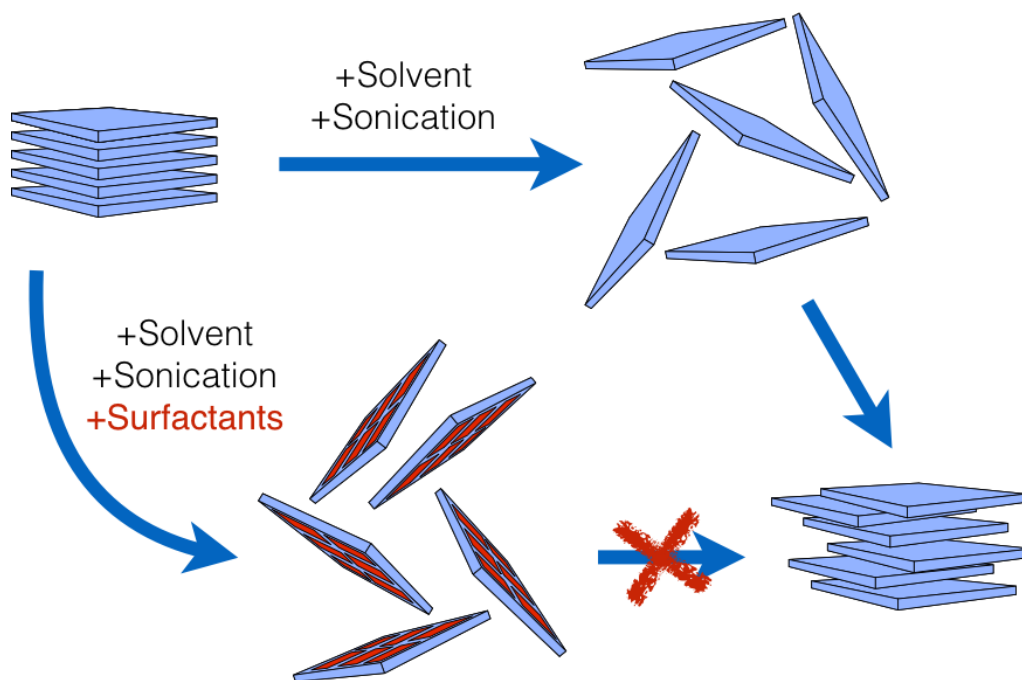
Figure 7.1: Schematic representation of the liquid-phase exfoliation by sonication in the absence (top) and presence (bottom) of dispersion stabilizing agents.
