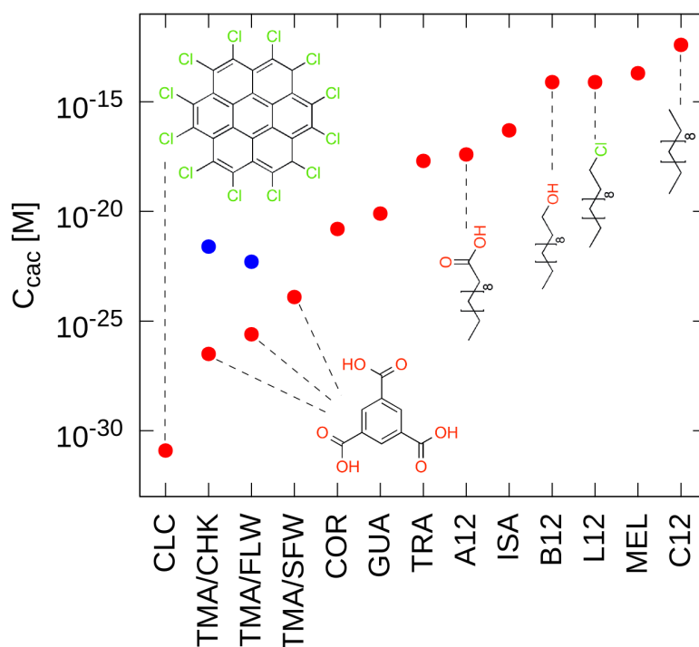
Figure 5.6: Critical aggregation concentration for the thirteen studied self-assembled architectures. For TMA, both the hydrogen bond uncorrected (blue) and corrected (red) values are reported.
