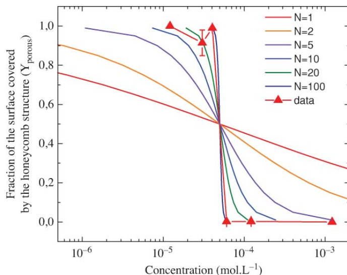
Figure 4.2: Surface coverage as a function of the concentration. The red points are the experimental values, while the different curves are the predicted surface coverages with different values for the domain size parameter N . Reproduced with permission from ref. 163 (Copyright 2011 AIP Publishing LLC).
