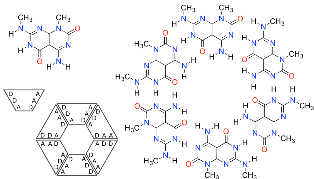
Figure 3.2: Chemical structures of the monomer and hexamer studied in this section. The monomer show two complementary hydrogen pattern (AAD and DDA) on the two sides of the molecule, allowing the self-assembly in the hexamer.
