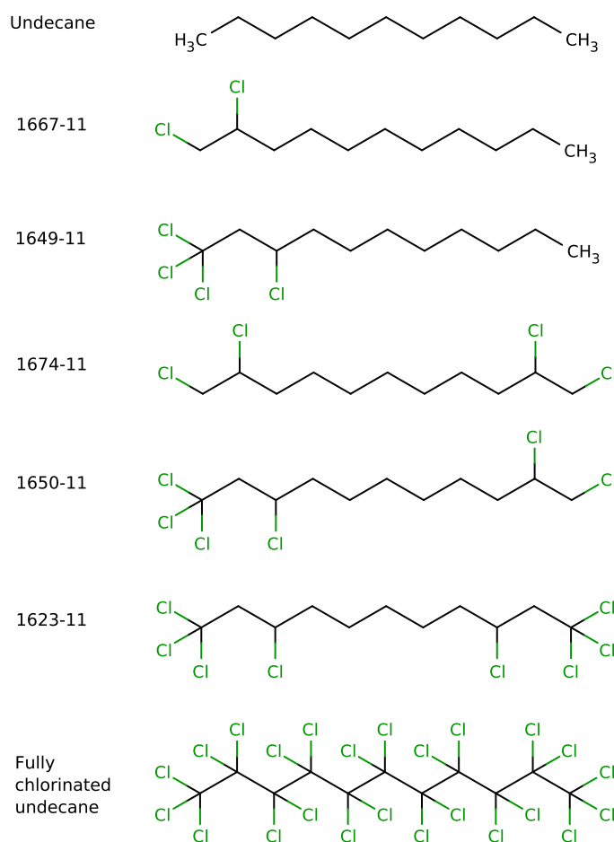
Figure 6.10: Molecular structured of the commercially available partially chlorinated undecane molecules studied in this work.
