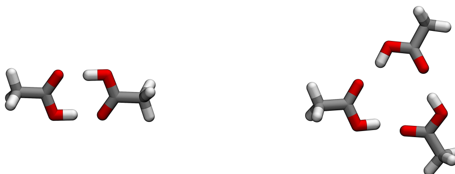
Sketch representations of the linear (left) and trigonal (right) hydrogen bond patterns of carboxylic acid self-assembly.
