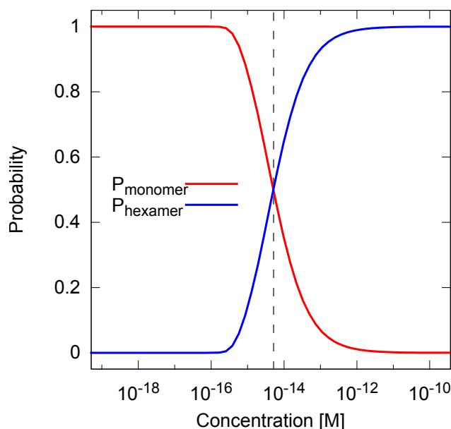
Figure 3.4: Molar fraction of the monomer and hexamer as a function of the initial concentration of monomers. The dashed gray line indicates the C_{A,\frac{1}{2}} , which delimits the domains of dominance of the monomer (at low concentrations) and of the hexamer (at high concentrations).
