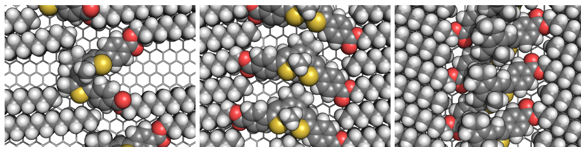
Figure 8.6: Magnification of the molecular models generated for the DAE-o (left), DAE-c (center), and DAE-b (right). Note how the alkyl chains are parallel in the DAE-o and antiparallel in the DAE-c and DAE-b, how the DAE-b is more dense than the DAE-c thanks to the different alkyl chain conformations, and the overlap of the cores of the molecules which is present only in the DAE-b.
