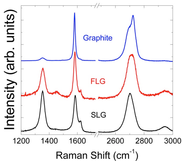
Figure 9.11: Typical Raman spectra obtained for graphene of different thickness produced by liquid phase exfoliation.
