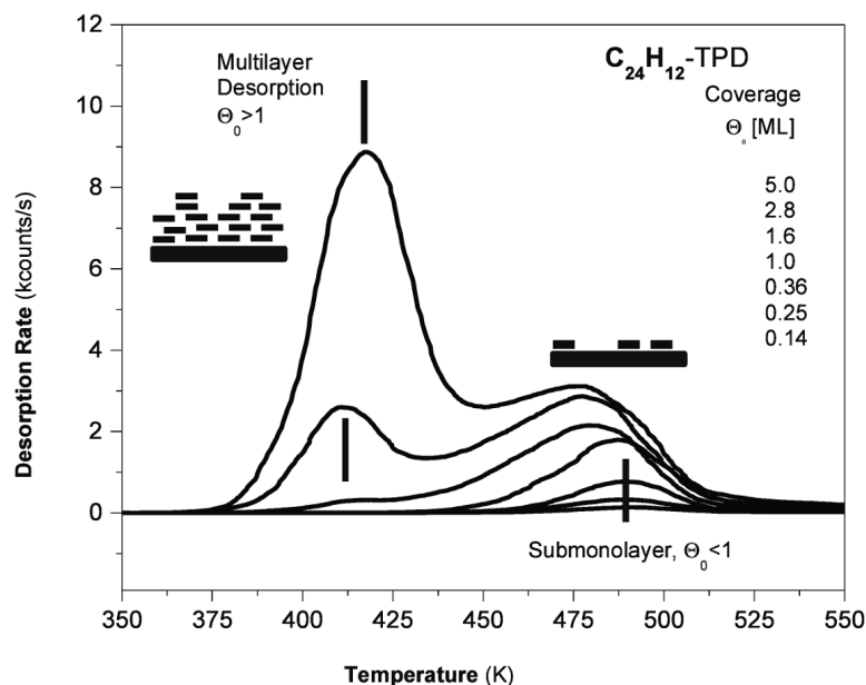
Figure 9.4: TPD spectra for the desorption of coronene obtained at different initial coverage \Theta_0 . The thermal desorption proceeds via two distinguishable peaks. The first at T_B \simeq 410 K reveals the sublimation of the multilayers. The second, peaked at T_S \simeq 480 K, represents desorption from the monolayer, where the molecule-surface interaction raises the binding energy by about 70 K.
