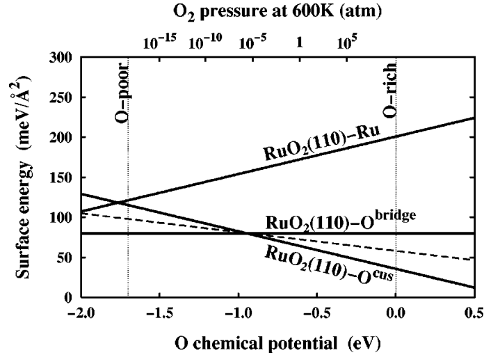
Figure 4.1: Example graph showing how the surface free energy changes as a function of the oxygen chemical potential for three different terminations of a \text{RuO}_2 (110) surface. Reproduce with permission from ref. 152.
