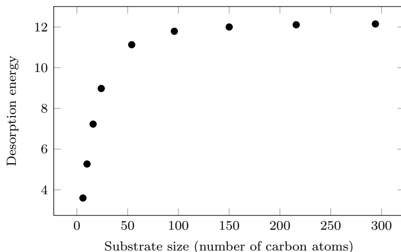
Figure 6.2: Desorption energy for benzene as a function of the size (measured as number of carbon atoms) of the graphene substrate calculated using the PM6-DH+ semiempirical method. The desorption energy essentially converges after 150 carbon atoms, while the used model contains 216 atoms.
