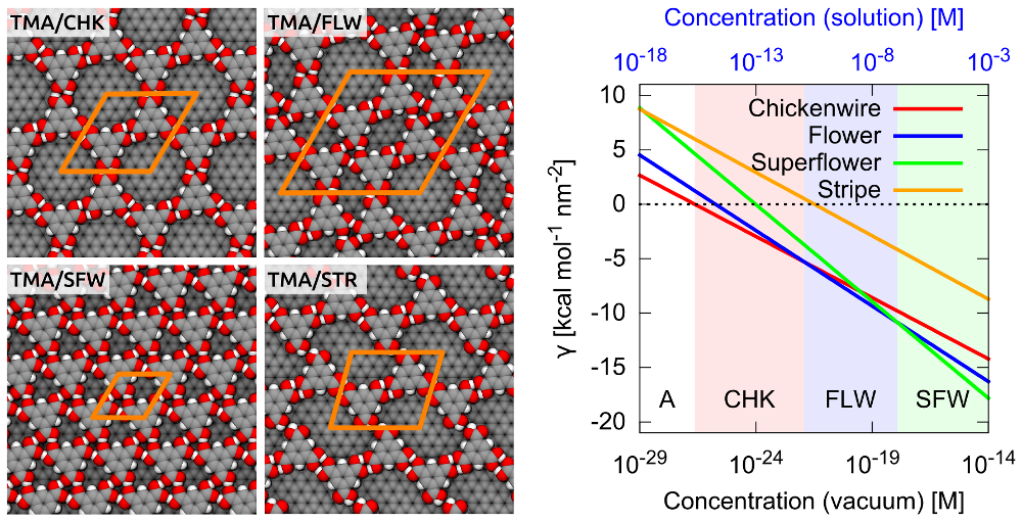
Figure 5.4: Surface free energy excess \gamma as a function of the monomer concentration for trimesic acid (TMA) self-assembly in the three different experimentally observed architectures – chickenwire (CHK), flower (FLW), and superflower (SFW) – and the hypothetical stripe (STR) architecture. The concentration dependency is evident, showing how at low concentration the disassembled state A is the favored, while at higher concentration the three assemblies CHK, FLW, and SFW are visible in order. The value of \gamma for the STR architecture is at all concentrations higher than the one of the others, indicating that architecture is never visible. The lower x axis (in black) indicates the concentration in vacuum, while the upper x axis (in blue) includes an approximation of the effect of the solvent (see Appendix B).
