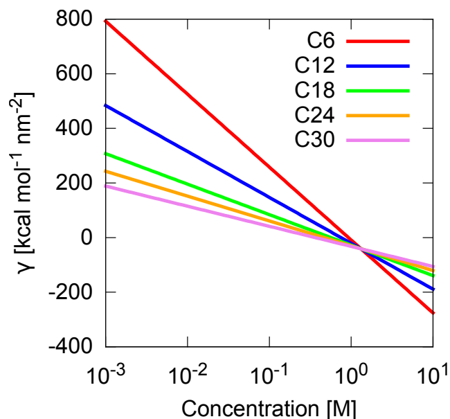
Figure 7.8: Effect of the concentration of the molecules in solution to the stability of the self-assembled monolayers. Since the stability of the shortest molecules is more strongly influenced by the entropy cost to self-assembly, due to higher number of molecules to constrain on the surface, \gamma changes more steeply, allowing an inversion of the stability ranking at high concentrations.
