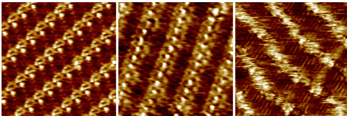
Figure 8.4: Height STM images obtained for the self-assembled monolayer of the DAE-o (left), DAE-c (center), and DAE-b (right) at the HOPG/1-phenyloctane interface.
