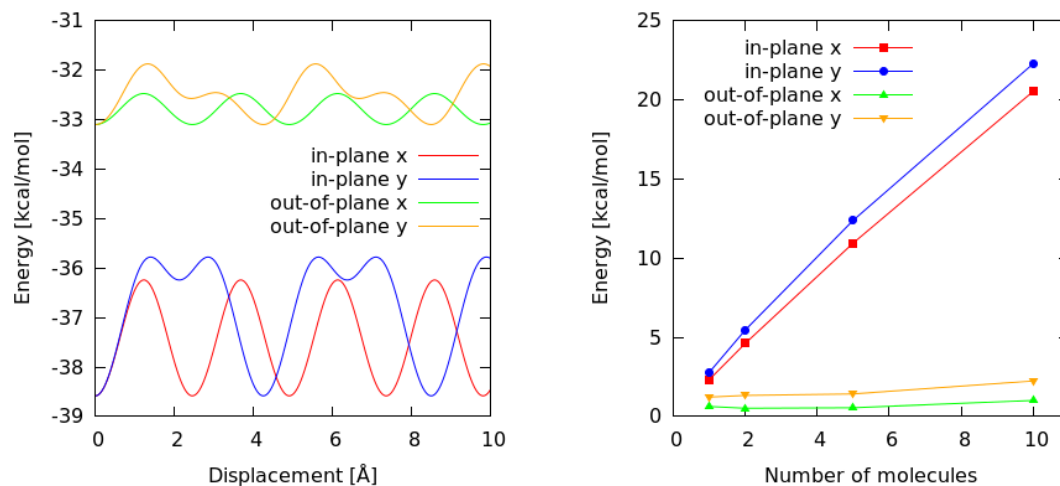
Figure 8.8: Left) Energy profiles obtained by displacing a C18 alkyl chain on a graphene surface along the x and y directions when adsorbed in the in-plane and out-of-plane zig-zag conformations. Right) Height of the energy barriers involved in the displaced in the x and y direction of a cluster of 1, 2, 5, and 10 molecules adsorbed in a in-plane and out-of-plane zig-zag conformation.
