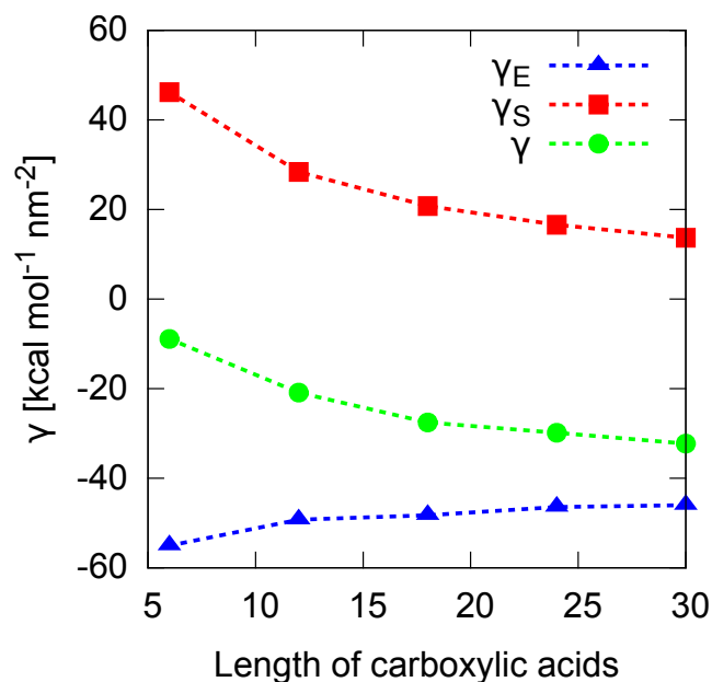
Figure 7.7: Surface free energy decomposed in energetic and entropic contributions evaluated for the five SAMs from C6 to C30.
