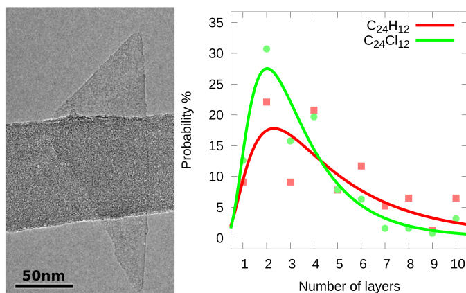
Figure 9.10: On the left, HR-TEM image of an exfoliated graphene bilayer. On the right, statistical analysis on the number of layers for the exfoliated graphene dispersion in the presence of coronene (red) or perchlorocoronene (green).
