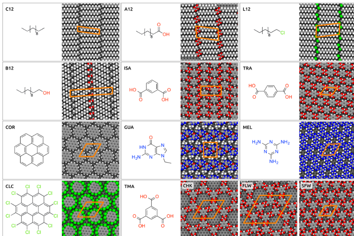
Figure 5.3: Modeled self-assembled monolayers and their chemical structures.
