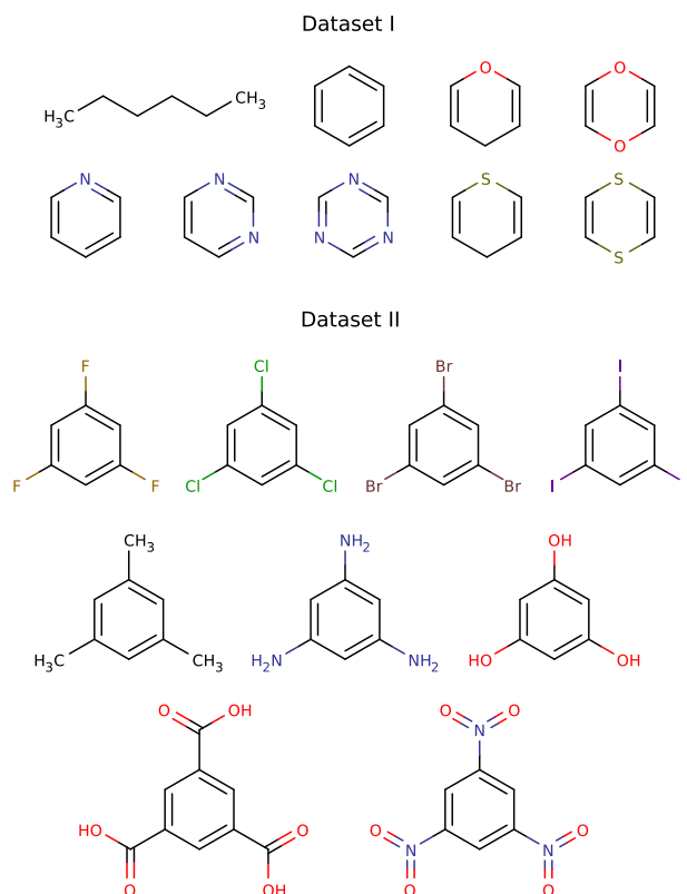
Figure 6.7: Molecular structures of the two data sets used to explore the effect of chemical functionalization on the desorption energy from graphene. In the first set, a benzene scaffold is modified by in-ring substitution with heteroatoms; in the second set, the benzene is 1,3,5 tri-substituted by different polarizable, electron donating, or electron withdrawing groups.
