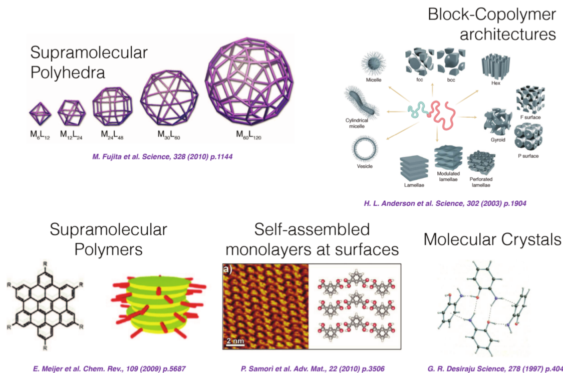
Figure 1.1: Examples of finite and infinite-size molecular self-assembly. Adapted with permission from ref. 6 (copyright 2010 American Association for the Advancement of Science), ref. 7 (copyright 2003 American Association for the Advancement of Science), ref. 11 (copyright 2009 American Chemical Society), ref. 12 (copyright 2004 American Chemical Society), and ref. 10 (copyright 1997 American Association for the Advancement of Science).
