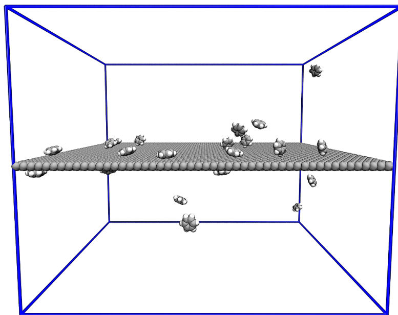
Figure 10.2: Typical simulation box used in the equilibrium sampling simulations. The graphene layer defines the xy plane, while the z dimension is changed systematically to simulate different values of the \eta parameter. Due to the periodic boundary conditions, the molecules can diffuse through the z dimension and adsorb on the graphene layer on both sides.
