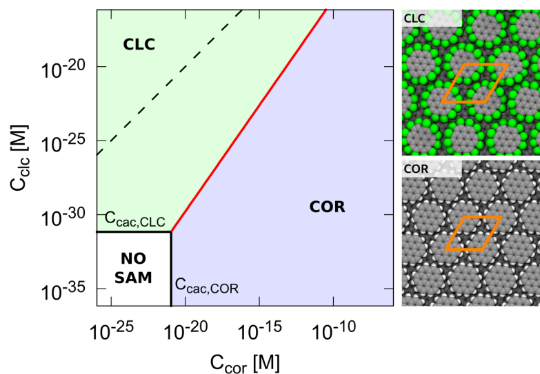
Figure 5.5: Phase diagram for the competitive self-assembly of coronene/perchlorocoronene mixtures. The two black solid lines indicate the critical aggregation concentrations, below which no self-assembly occurs. The red line represents the boundary where \gamma_{\text{COR}} = \gamma_{\text{CLC}} , which implies equal probability to observe one or the other SAM. Below the red line the preferred SAM is the one formed by coronene; over it, the preferred is perchlorocoronene. The dashed line indicate the locus where the concentration of coronene and perchlorocoronene are equal.
