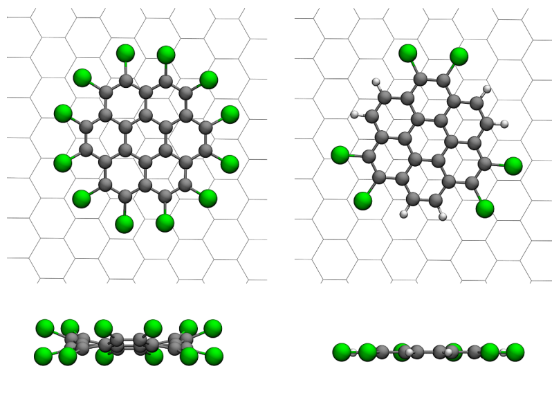
Figure 9.13: Comparison of the geometries of perchlorocoronene (left) and the 1,2,5,6,9,10-hexachlorocoronene (right). While the chlorine atoms are highly out of plane in the former due to the high steric repulsions, the second is completely flat.
