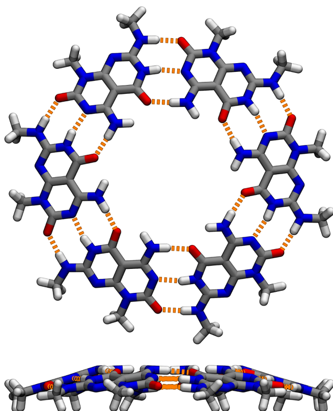
Figure 3.3: Top and side view of the optimized model of the hexamer. In the side view the curvature is evident as all monomers are not flat on the surface, but are slightly tilted upwards by about 20^\circ .
