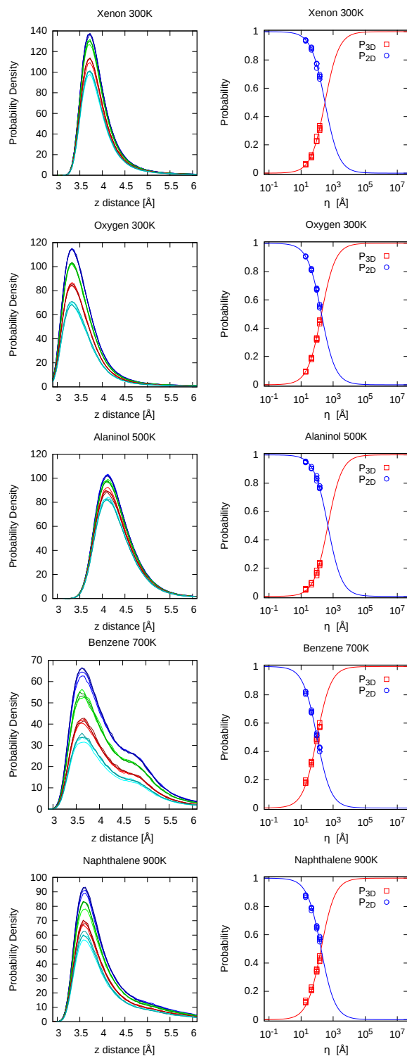
Figure 10.3: Equilibrium sampling results for the five studied systems. Left: probability density as a function of the distance from the surface; the blue, green, red and cyan curves indicate the value of \eta (19, 44, 94, 144 Å). Right: probability of the desorbed and adsorbed states as a function of the extension parameter \eta . Each of the four points corresponds to the superimposition of the four simulations at constant \eta value.
