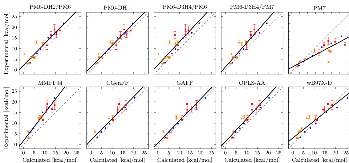
Figure 6.3: Correlation plots between the calculated and the experimental desorption energies. Five semiempirical methods (PM6-DH2/PM6, PM6-DH+, PM6-D3H4/PM6, PM6-D3H4/PM7 and PM7), four force fields (MMFF94, CGenFF, GAFF and OPLS-AA), and one DFT functional ( \omega B97XD/6-31G(d)) are reported. The color of the dots represents the class of the molecule: blue alkanes, red aromatic compounds, and orange small molecules and solvents. The error bars represent the experimental uncertainties in the TPD data. The dashed gray line indicates the ideal fit, compared to the real linear fit (solid black line).
