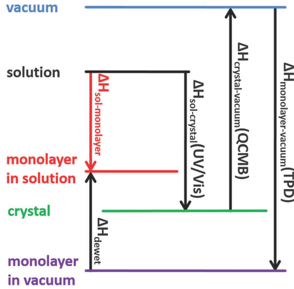
Figure 4.3: Born-Haber thermodynamic cycle used to access the enthalpic driving force for self-assembly at surfaces. Reproduced with permission from ref. 171.
