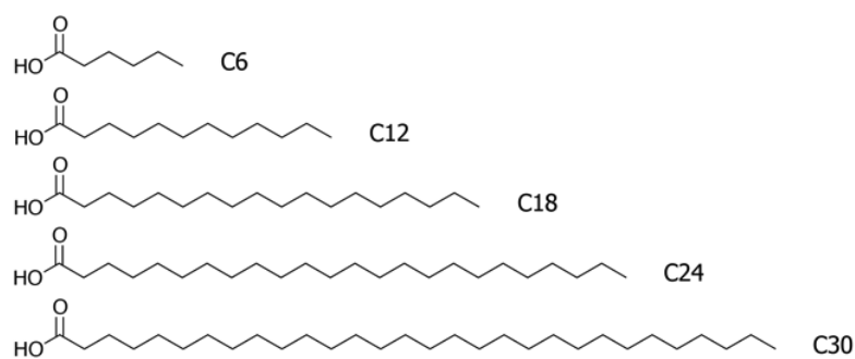
Figure 7.2: Chemical structure of the fatty acids studied, from hexane (C6) to triacontane (C30).
