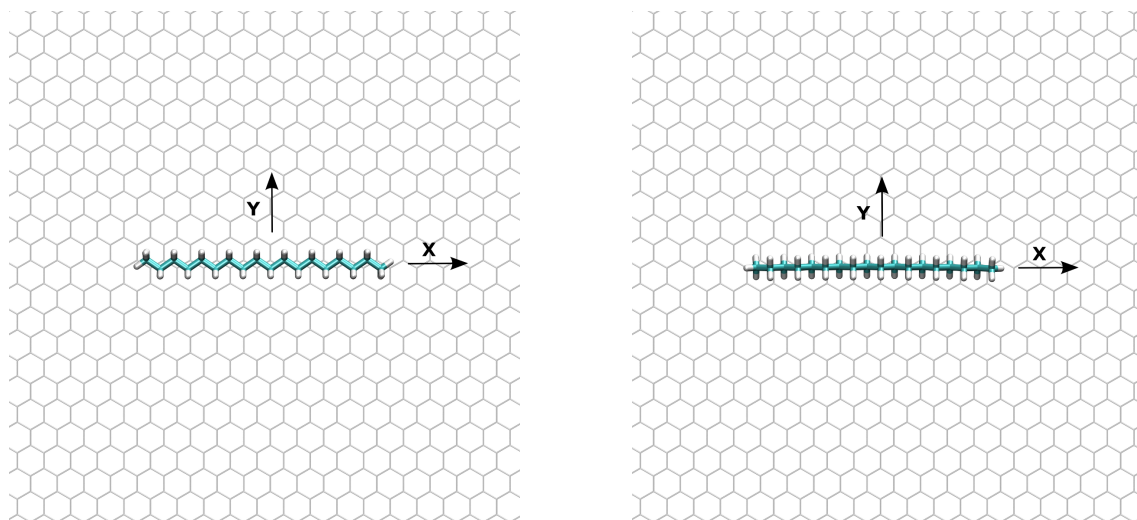
Figure 8.7: Minimized in-plane and out-of-plane conformation of octadecyl chain on graphene. The arrows show the direction of the displacements used to build the energy profiles and evaluate the energy barriers.
