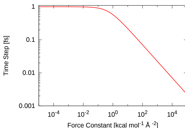
Figure E.1: Time step as a function of the force constant of the applied harmonic restrain.
