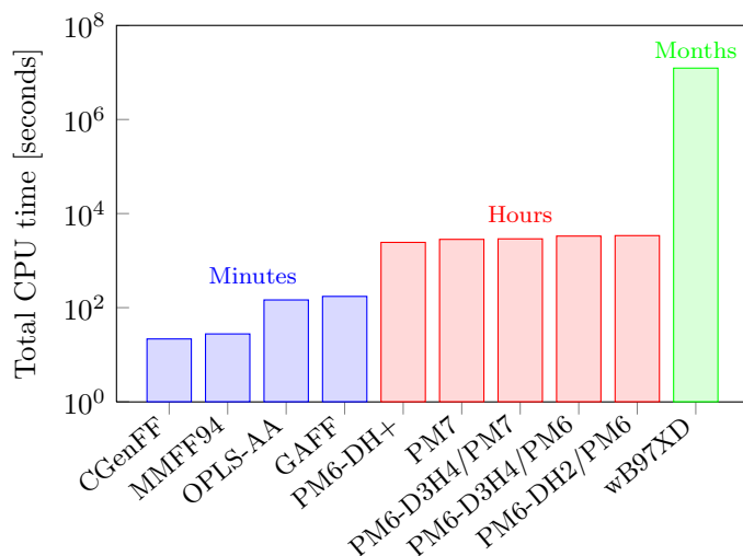
Figure 6.5: Average CPU time needed to calculate the desorption energy of one molecule using the different computational methods here benchmarked. This corresponds to the time on a single processor: SQM and DFT calculation are actually run in parallel decreasing significantly the user time.
