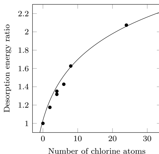
Figure 6.11: Relative desorption energies of the PCA with respect to undecane plotted as a function of the number of chlorine atoms present in the molecule. As main feature, the increase in the desorption energy is not linear with the chlorine content.
