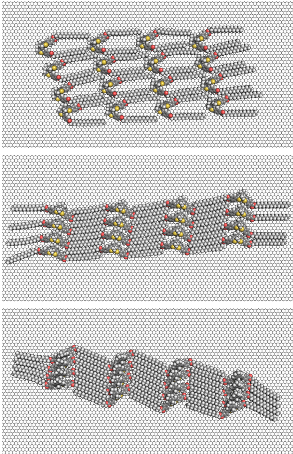
Figure 8.5: Optimized models of the 4 \times 4 cells self-assembled architectures for the open (top), closed (center), and byproduct (bottom) isomers of DAE.
