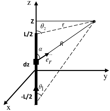
Figure VI.5: Portion de fil
