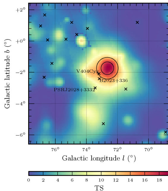
Figure 3. 12 h residual TS map on MJD 57199.25 (0.1–2 GeV, 0^\circ 1 pixel ^{-1} ). 3FGL sources are marked as black crosses. 68 and 95 per cent confidence regions on the best-fitting position are represented.
