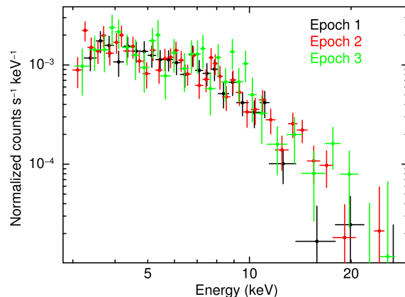
Figure 7. NuSTAR FPMA spectra for three epochs of observations. Black, red, and green points correspond to epochs 1, 2, and 3, respectively.
