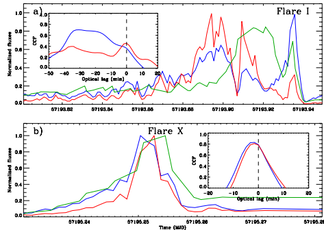
Fig. 2. V-band (green), 3–13 keV (red), and 20–40 keV (blue) LCs around flares I a) and X b). The insets show the cross-correlation functions of the 3–13 keV (red) and 20–40 keV (blue) vs. the optical LCs over the same time intervals as the LCs. The dashed vertical lines represent the 0 lag level.
