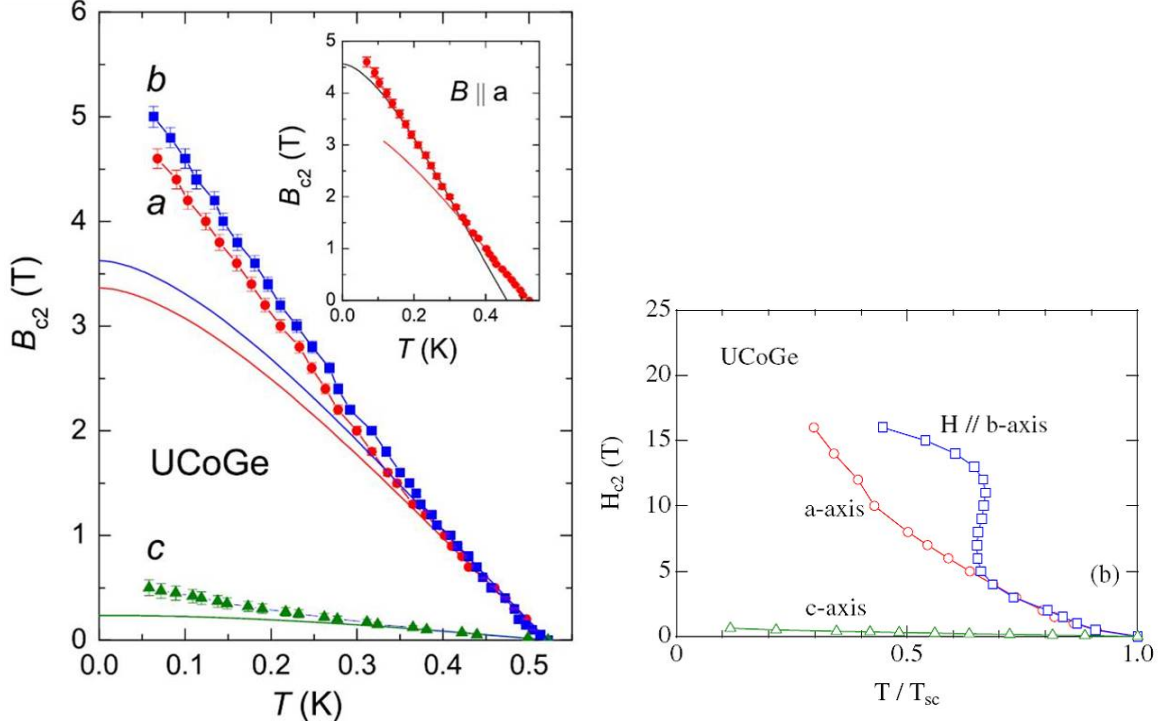
Figure 3.4 Critical field of UCoGe along the three crystallographic directions [87, 12].
