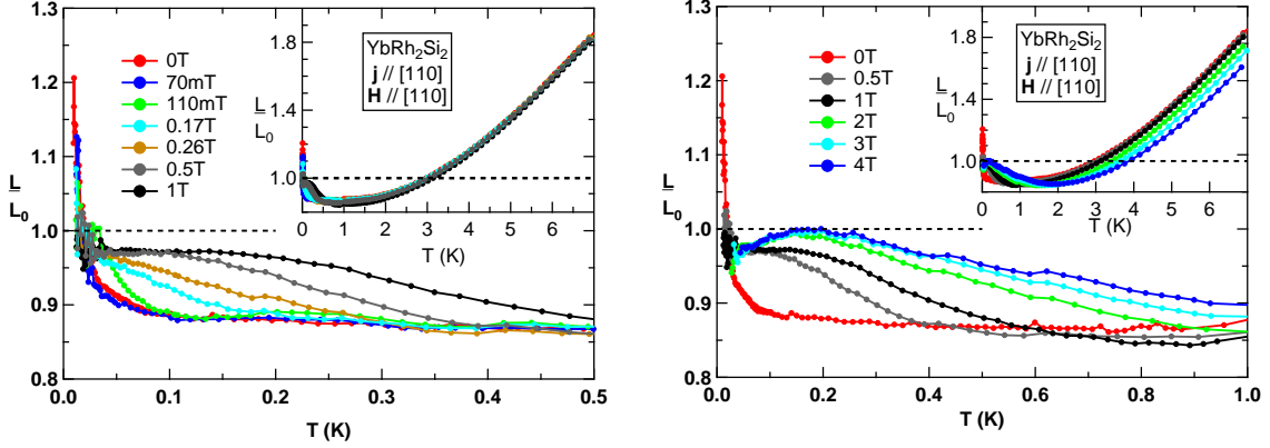
Figure 5.12 Lorenz ratio below 1\text{T} (left panel) and up to 4\text{T} (right panel) below 1\text{K} . In insets are displayed the Lorenz ratios in the whole temperature range.
