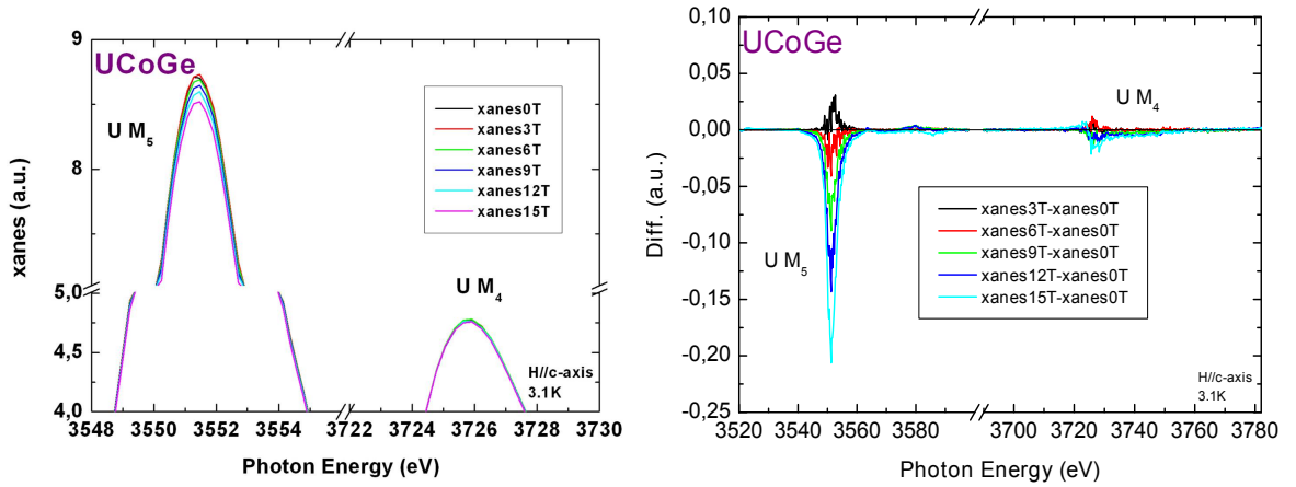
Figure 3.21 Left panel: XANES at various fields of M_5 - and M_4 -edges, only close to the maximum, at 3K, \mathbf{H}/\mathbf{c} . Right panel: difference between the XANES measured under field with the one at 0T.
