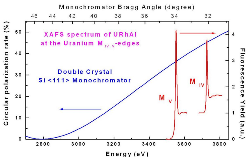
Figure 2.10 Polarization transfer by the monochromator at the U M -edges. Courtesy of F. Wilhelm and A. Rogalev.
