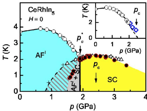
Figure 3.8 Phase diagram of \text{CeRhIn}_5 under pressure [109]. The round points ( \bullet ) are the transition measured by specific heat, the triangles ( \Delta ) by susceptibility and the crosses ( + ) by resistivity. In the magnetic phase, the superconducting temperature differs according to the probe, whereas it is similar in the non magnetic phase.
