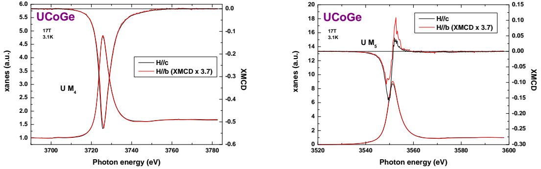
Figure 3.26 Comparison of XANES and XMCD of the uranium at 3K, 17T between the configurations \mathbf{H}/\mathbf{b} and \mathbf{H}/\mathbf{c} for the M_4 -edge (left panel) and the M_5 -edge (right panel). A multiplying factor has been applied on the XMCD signal when \mathbf{H}/\mathbf{b} .
