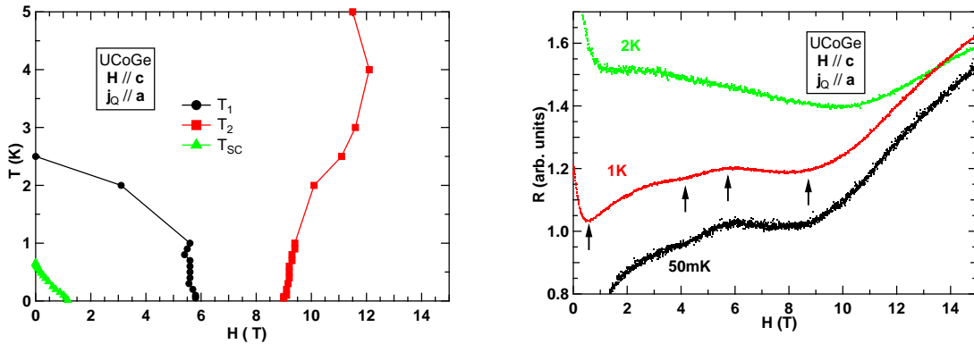
Figure 3.25 Left panel: temperature and field dependence of the resistive anomalies. The superconducting temperature has also been plotted (green triangles). Right panel: zoom on the magnetoresistivity at 50mK (in black), 1K (in red) and 2K (in green). The arrows show the different anomalies visible.
