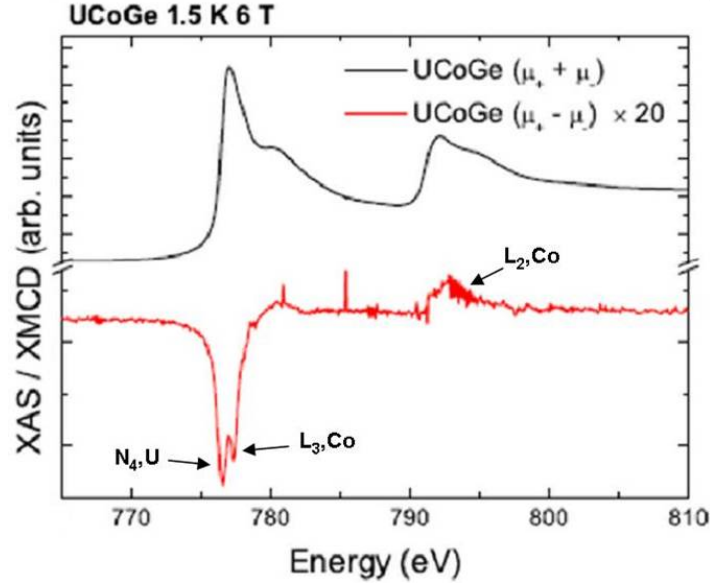
Figure 3.27 XMCD measurements at low energy. The L_3 -edge and the L_2 -edge of the cobalt has been measured, but the proximity of the N_4 -edge of the uranium to the L_3 edge makes the results difficult to interpret.
