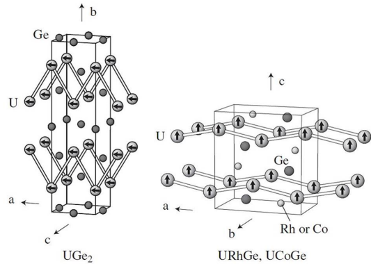
Figure 1.11 Crystallographic structure of \text{UGe}_2 , \text{URhGe} and \text{UCoGe} . The arrows represent the direction of the magnetic moments. From [8].
