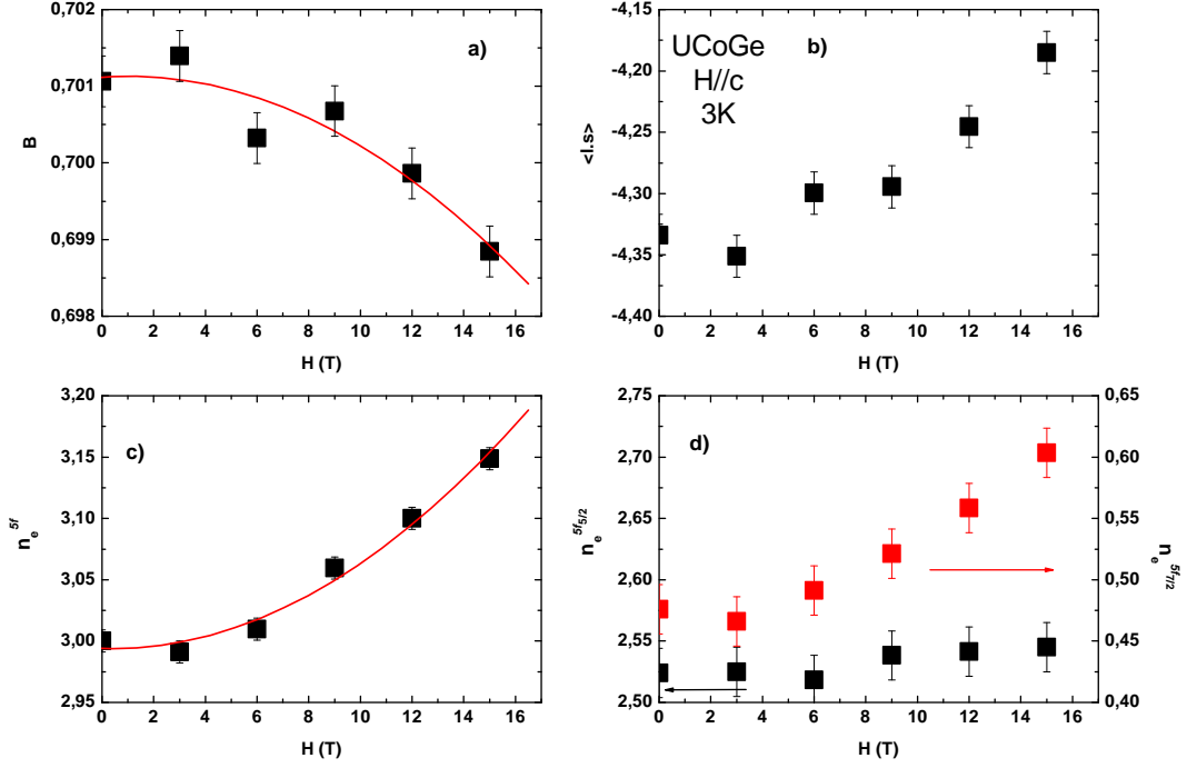
Figure 3.22 Evolution with the field of the branching ratio (panel a ), \langle l.s \rangle (panel b ), the total number of 5f electrons (panel c ) and in the 5f_{5/2} and 5f_{7/2} shells (panel d ).
