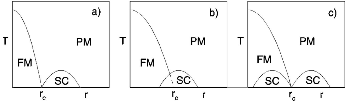
Figure 1.6 Different scenarios when existence of superconductivity close to a magnetic instability. Panel (a): SC exists only out of the FM phase, like Fe under pressure [193, 184]. The superconductivity exists in both phases, with the vanishing of T_{sc} at the QCP (Panel (c)) or not (Panel (b), case of UCoGe). The panel (c) has been predicted by Fay and Appel [46], and is similar to UGe 2 , but no superconductivity has been detected in the PM phase up to now. The parameter r represents the "distance" to the QCP. From [179].
