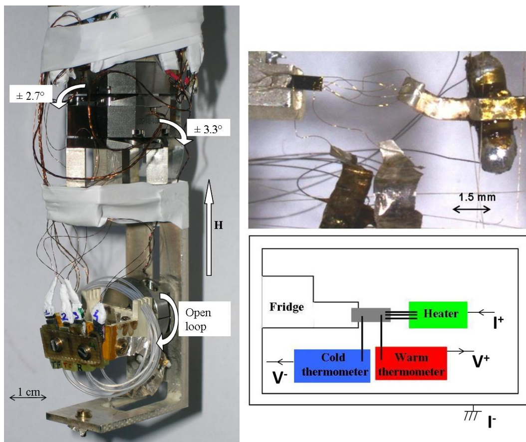
Figure 2.6 On the left: the whole stage with the two goniometers, the rotator and the sample holder. On the right, a zoom of the thermal conductivity setup: regular two-thermometer one-heater setup for the thermal conductivity measurements (photo on the top and sketch on the bottom).
