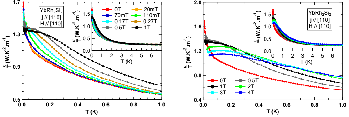
Figure 5.11 Thermal conductivity of \text{YbRh}_2\text{Si}_2 below 1\text{K} and 1\text{T} (left panel) and above 1\text{T} (right panel). In insets are shown the same quantities in the whole temperature range.
