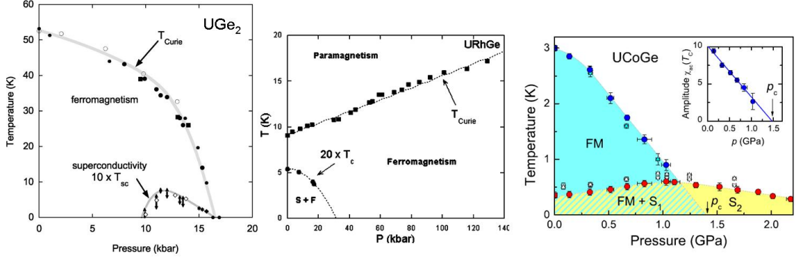
Figure 1.14 ( P - T ) phase diagram of UGe_2 [85], URhGe [68] and UCoGe [194, 72].
