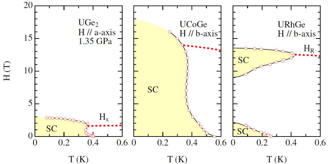
Figure 1.13 Critical fields of UGe 2 [191], UCoGe [12] and URhGe [119] along one particular direction. From [11].
