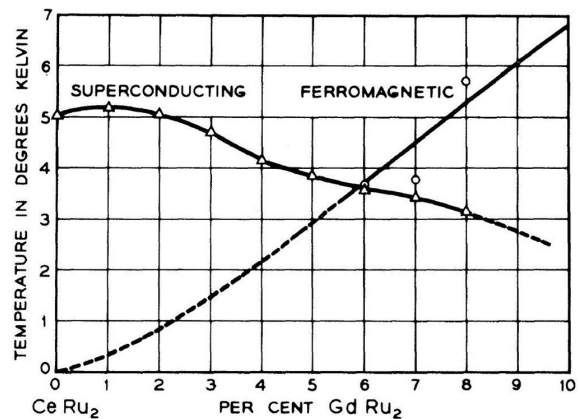
Figure 1.7 Superconducting phase diagram of the Gd-doped CeRu 2 [133].
