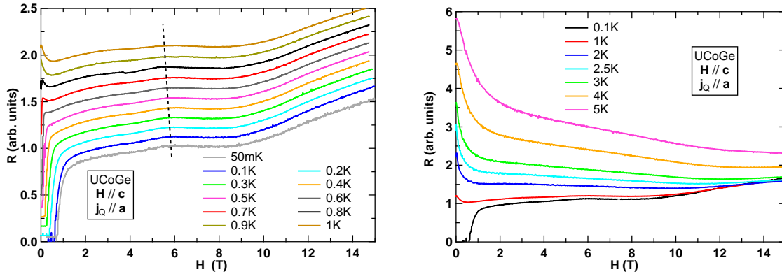
Figure 3.24 Magnetoresistivity of UCoGe below 1K (left panel) and above (right panel) in the configuration H // c and j_Q // a .
