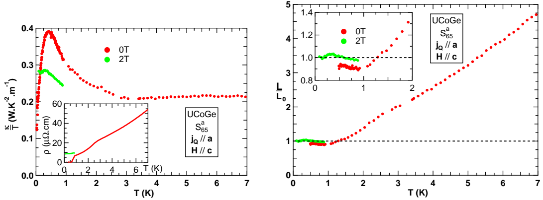
Figure 4.8 On the left, the thermal conductivity and the resistivity (in inset) of sample S_{65}^a with the field along the \mathbf{c} -axis. On the right is displayed the Lorenz ratio with a zoom of the low temperature part in inset.
