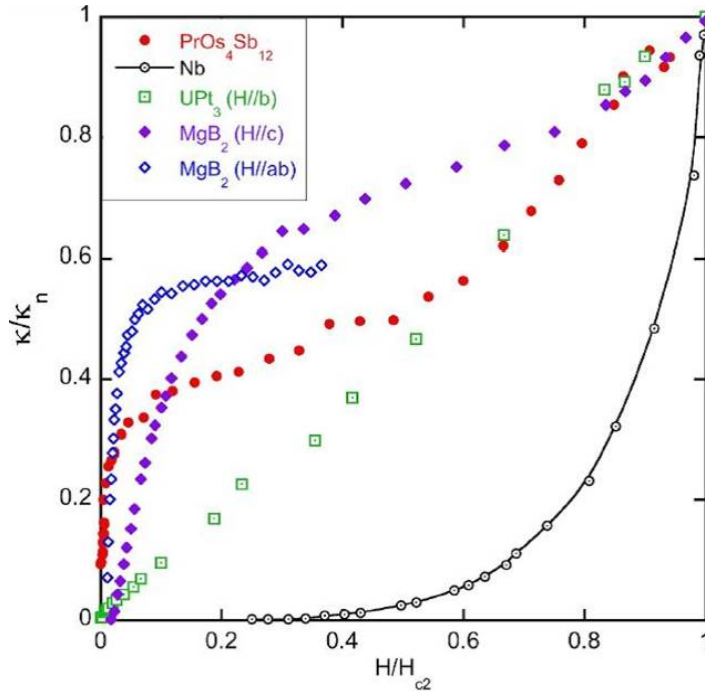
Figure 2.4 Magnetic field dependence of the normalized residual thermal conductivity of some compounds. Nb shows an exponential behavior whereas UPt 3 is almost linear. MgB 2 and PrOs 4 Sb 12 are multigap superconductors. From [189].
