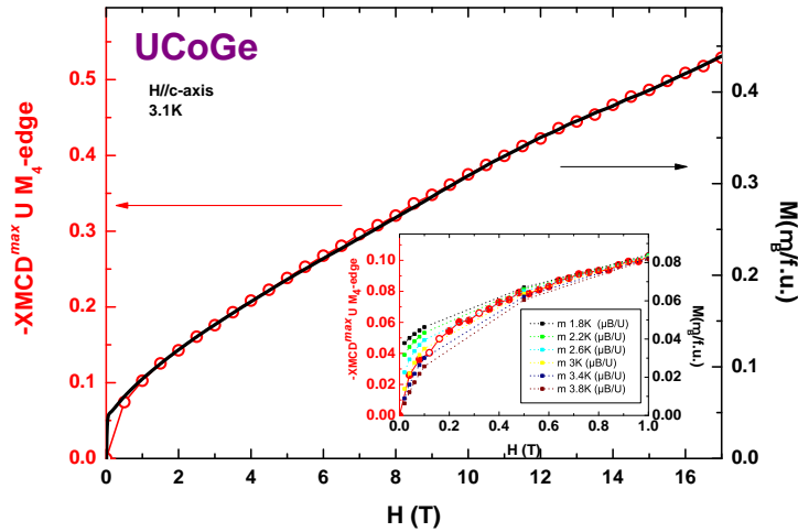
Figure 3.17 XMCD of the U M_4 -edge at 3K between 0T and 17T, \mathbf{H}/\mathbf{c} , with the comparison with the macroscopic magnetization (right axis). In inset is shown the low field measurements, which enables to determine the temperature of the sample.
