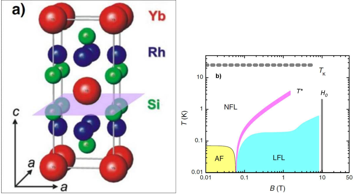
Figure 5.1 Panel a) the tetragonal structure of \text{YbRh}_2\text{Si}_2 (from [239]). Panel b) the low field phase diagram of \text{YbRh}_2\text{Si}_2 , with \mathbf{H} \perp \mathbf{c} . AF is the antiferromagnetic phase and LFL the paramagnetic phase with a Fermi liquid behavior. T^* is a crossover between the two regimes corresponding to the nature of the QCP (Kondo breakdown or Lifshitz transition), T_K is the coherence temperature and a topological transition is suspected to occur at H_0 [170]. Note that in the configuration \mathbf{H} // \mathbf{c} , a similar phase diagram is found. From [63].
