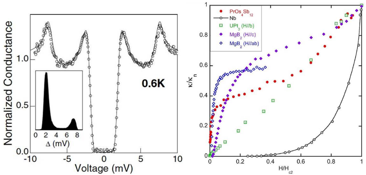
Figure 1.5 STM spectroscopy in the multigap superconductor MgB_2 [129] (left panel) and thermal conductivity measurements in the multigap superconductors MgB_2 and PrOs_4Sb_{12} , and in the one band Nb (conventional SC) and UPt_3 (unconventional SC) [189] (right panel).
