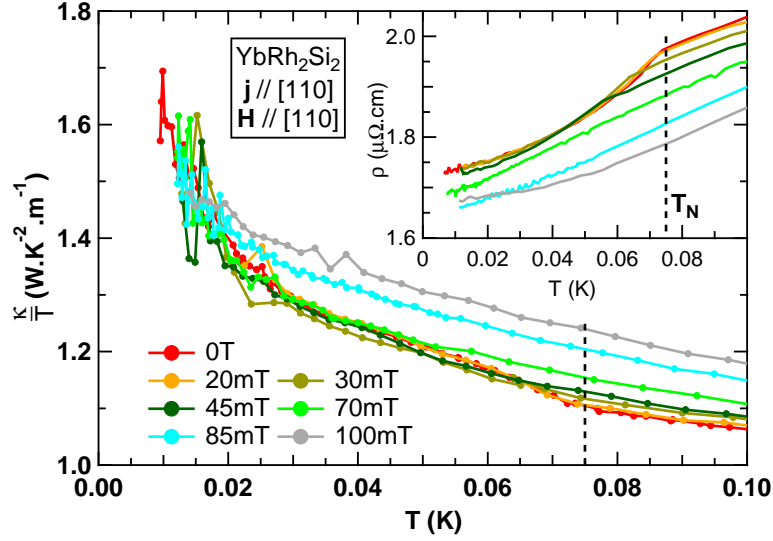
Figure 5.6 Thermal conductivity and electrical resistivity (in inset) of \text{YbRh}_2\text{Si}_2 below 0.1K and below 0.1T. The vertical dashed lines represent the Néel temperature at zero field.
