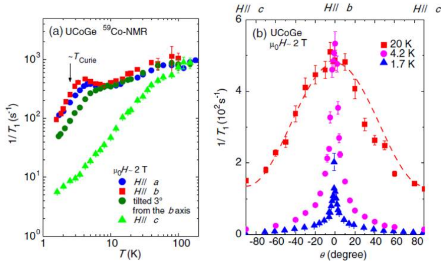
Figure 4.16 Panel (a): Evolution of 1/T_1 by NMR measurements. At 2T, the ratio 1/T_1 does not depend on the field direction when applied along the a and the b -axis, but is strongly suppressed when applied along the c -axis, indicating the longitudinal character of the magnetic fluctuations. The suppression starts has high temperatures, approximately 80K. Panel (b): Angle dependence of the relaxation rate of the magnetic fluctuations at several temperatures. At 20K (in red), the angle evolution is regular, as seen by the expected sinusoidal behavior (dashed line). At lower temperatures, a sharp maximum lies when \mathbf{H} is close to the b -axis, indicating that the fluctuations are suppressed by the component along the c -axis of the magnetic field. From [74].
