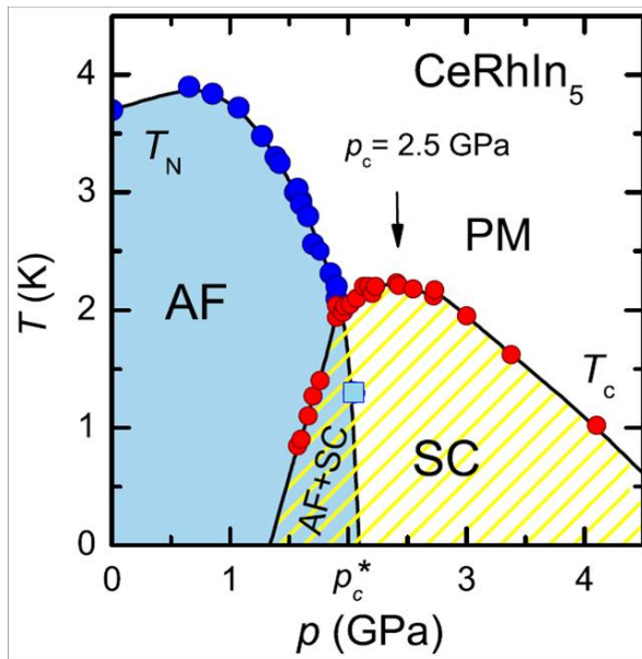
Figure 2 Typical phase diagram of a heavy fermion, represented by \text{CeRhIn}_5 [108]. AF, PM and SC are the antiferromagnetic, the paramagnetic and the superconducting states respectively. T_N and T_c are the Néel and the superconducting temperatures respectively. p_c and p_c^* are the critical pressures corresponding to the maximum of the superconducting temperature and to the pressure where T_N \rightarrow 0\text{K} respectively.
