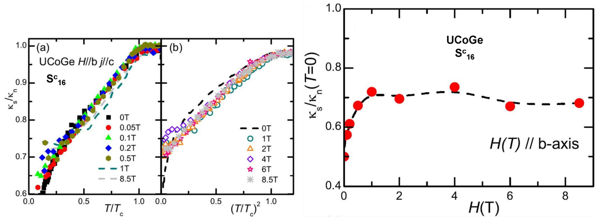
Figure 4.24 \kappa_{sc}/\kappa_N versus T/T_{sc} (on the left) and versus (T/T_{sc})^2 (in the middle) and versus H (on the right) of sample S_{16}^c when \mathbf{H}/\mathbf{b} . From [83].
