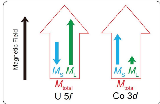
Figure 3.28 Schematic sketch of the direction of the Co and U moments in UCoGe, similar to UCoAl [214]. The arrows are not in scale.
