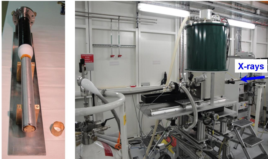
Figure 2.7 Probe (left) and the fridge with the X-rays line (right) used at the ID12 line at ESRF. Courtesy of F. Wilhelm and A. Rogalev.
