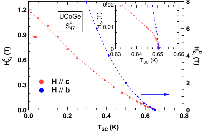
Figure 3.13 Critical field of sample S_{47}^c measured by resistivity with \mathbf{H}//\mathbf{c} and \mathbf{H}//\mathbf{b} . In inset: zoom of the very low field part. A small step is visible in the critical field at low field when \mathbf{H}//\mathbf{c} whereas it is strictly linear when \mathbf{H}//\mathbf{b} . The dashed lines are guides to the eyes.
