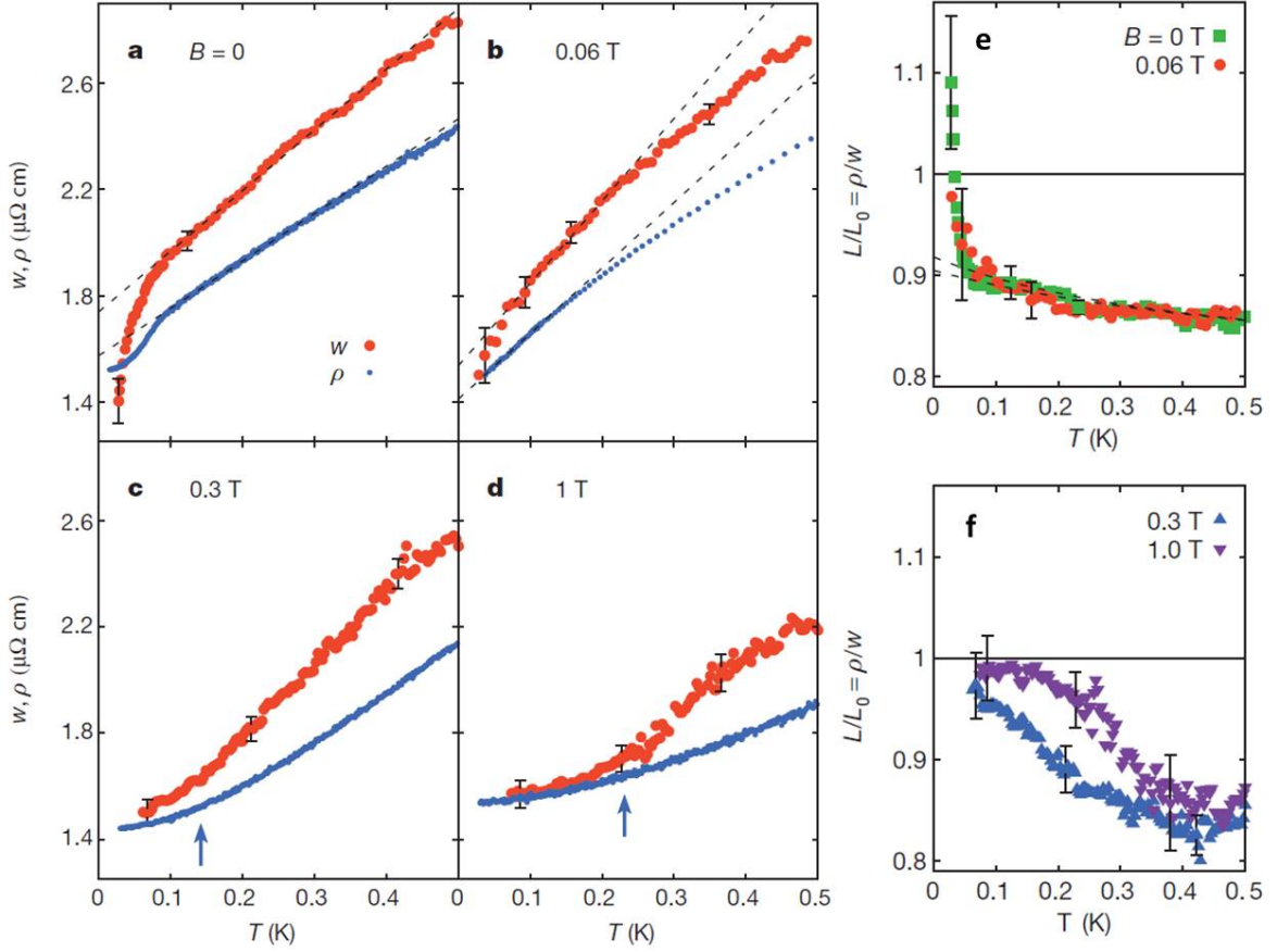
Figure 5.3 Thermal ( w_{th} ) and electrical ( \rho ) resistivities, measured by Pfau et al. [165], below H_c at 0\text{T} (panel a), close to the QCP at 60\text{mT} (panel b) and above H_c ( 0.3\text{T} (panel c) and 1\text{T} (panel d)). The Lorenz ratios at 0\text{T} and 60\text{mT} are displayed panel e, and at 0.3\text{T} and 1\text{T} panel f.
