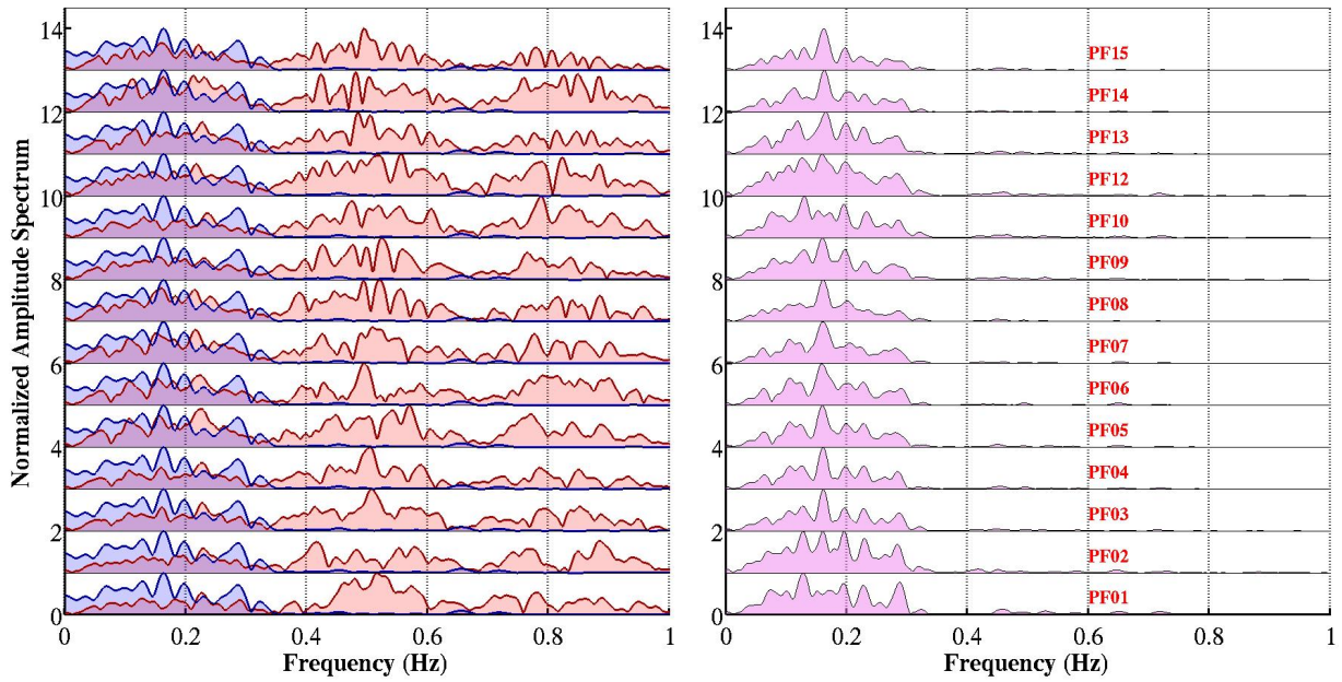
Figure 6.27: Amplitude spectra of the vertical component of the 2012 April 02 event. The left panel shows the normalized amplitude spectrum of the source wavelet for the event |\bar{W}(\omega)| (blue shaded area) and the normalized amplitude spectra of point source Green's function |G(\mathbf{x}_r, \omega)| (red shaded area) for the transect stations on the French side. The right panel shows the normalized amplitude spectra of the corresponding synthetic seismograms |\tilde{U}(\mathbf{x}_r, \omega)| (violet shaded area).
