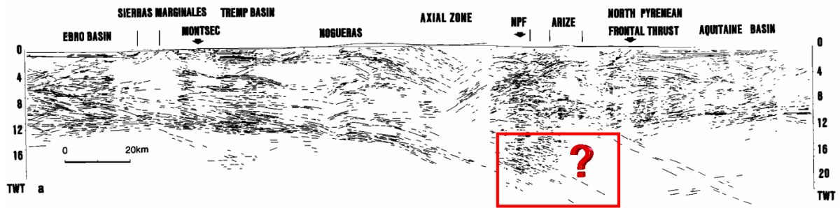
(a) Unmigrated reflection data from ECORS-Pyrenees profile.
