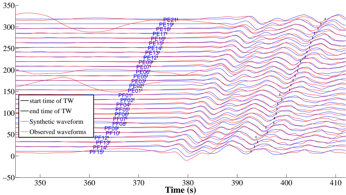
(a) Vertical components of observed and synthetic waveforms
