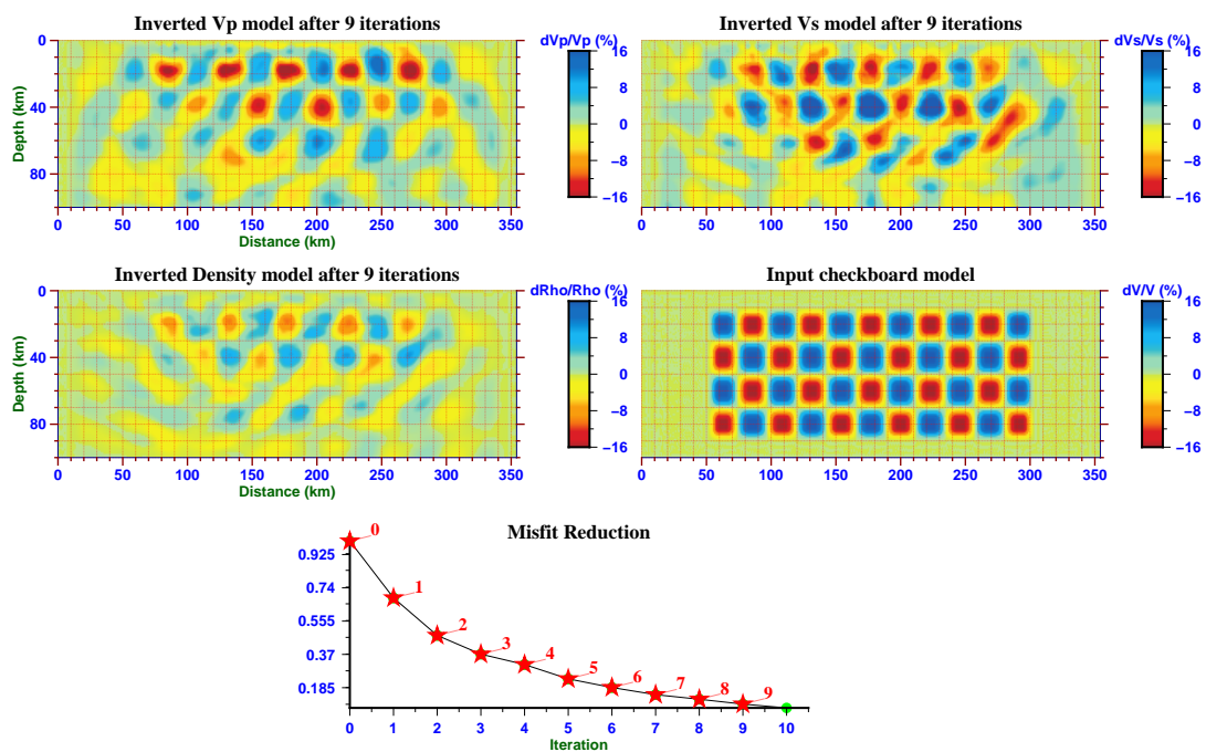
(a) Inverted velocity and density models using a uniform corner frequency filter on all the available three component waveforms.
