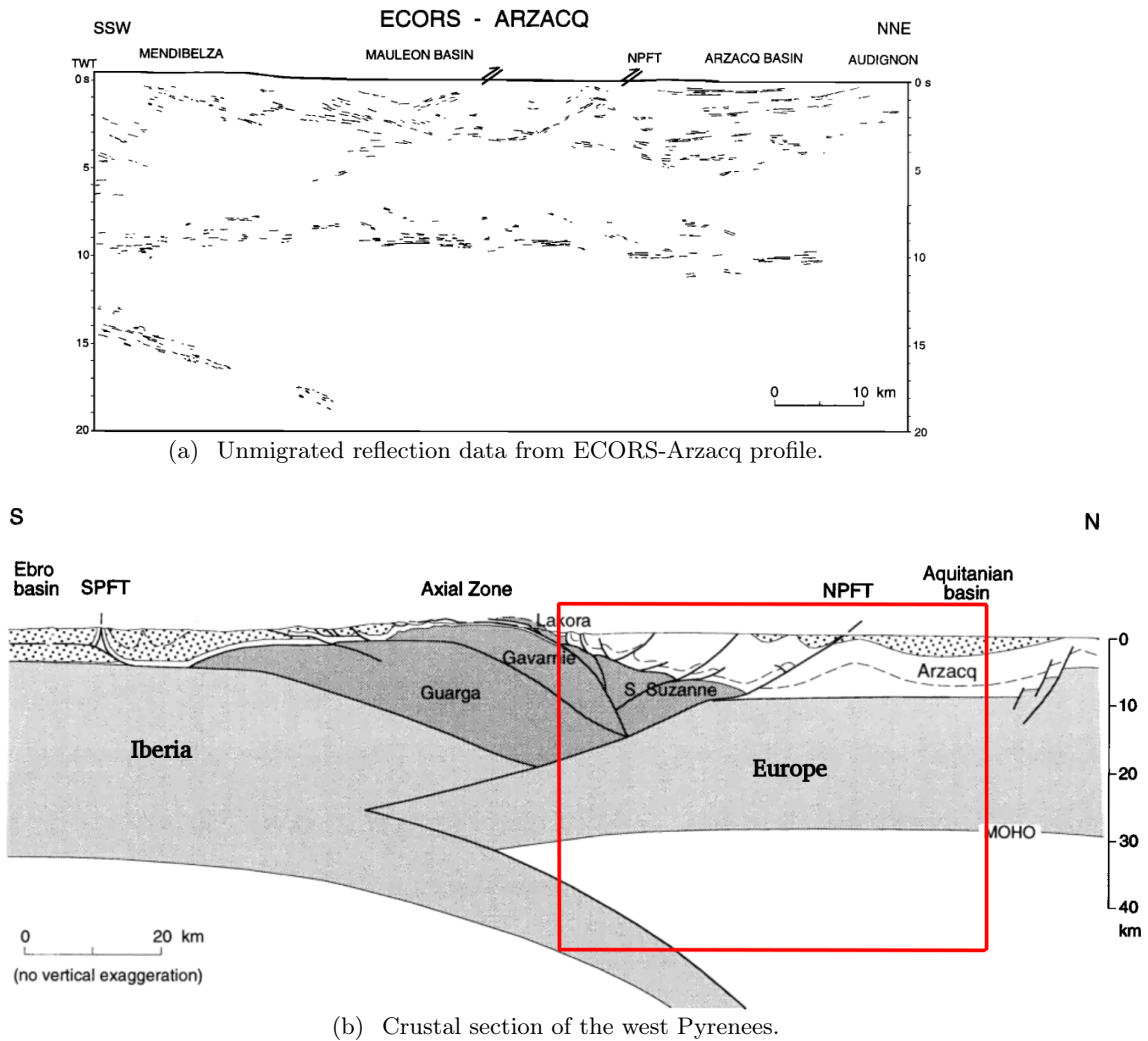
Figure 1.5: Reflection data and interpretation of the ECORS-Arzacq profile (from Teixell, 1998). (a) Line drawing of the unmigrated ECORS-Arzacq vertical reflection profile, from the published data given by Daignières et al. (1994). The evident subhorizontal reflections at 9 to 10 s two-way time along the entire profile are identified as the European Moho. The dipping reflections at 14 to 18 s TWT in the southern part of the profile display the underthrusting of the Iberian lower crust. (b) Teixell's crustal section of the western Pyrenees. The cross-section shows the stacked tectonic wedges at different crustal levels, formed by deep indentation of the Iberian crust by the European crust. The structures of the crustal root and the European crust are imaged by the ECORS-Arzacq profile shown with the red frame. The dotted pattern indicates Tertiary rocks. The dashed line in the northern Pyrenees displays the top of Jurassic.
