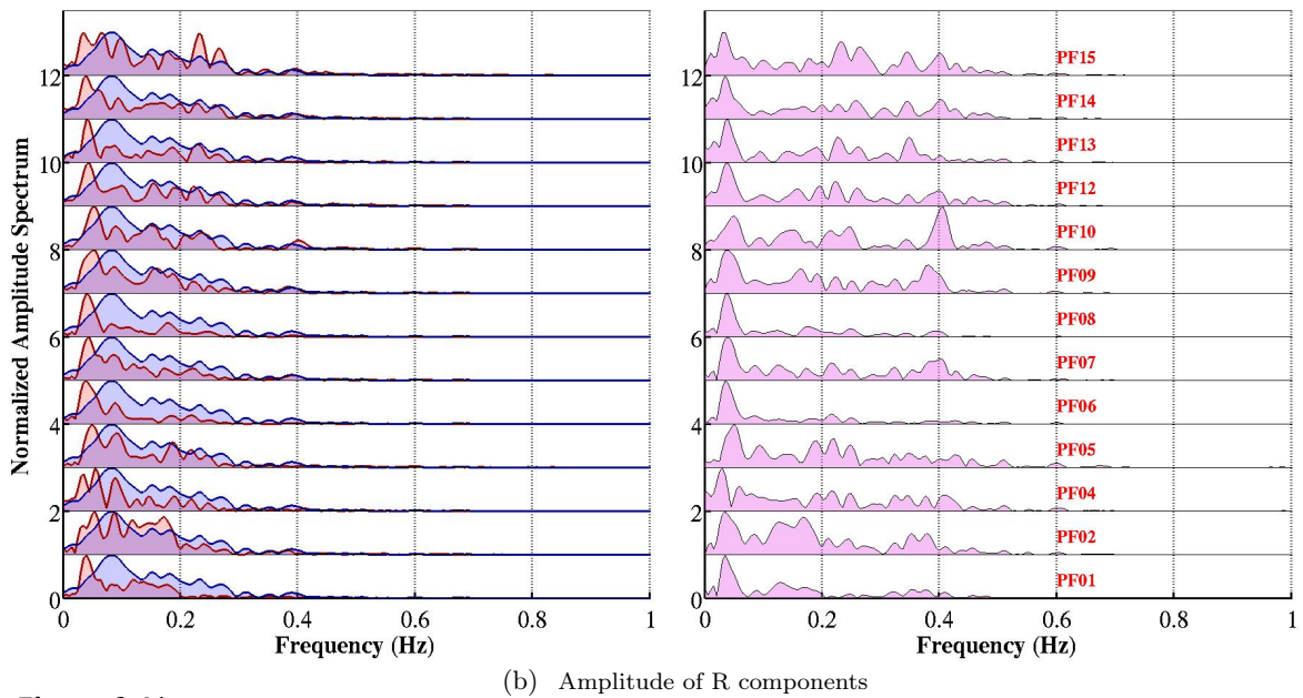
Figure 6.41: Amplitude spectra of the vertical component (a) and the radial component (b). Left panel: Normalized amplitude spectra of the May 24 source wavelet |\bar{W}(\omega)| (blue shaded area) and data traces |D(\mathbf{x}_r, \omega)| (red shaded area) of some transect station. Right panel: Normalized amplitude spectra of the deconvolved data traces |\tilde{d}(\mathbf{x}_r, \omega)| (violet shaded area).
