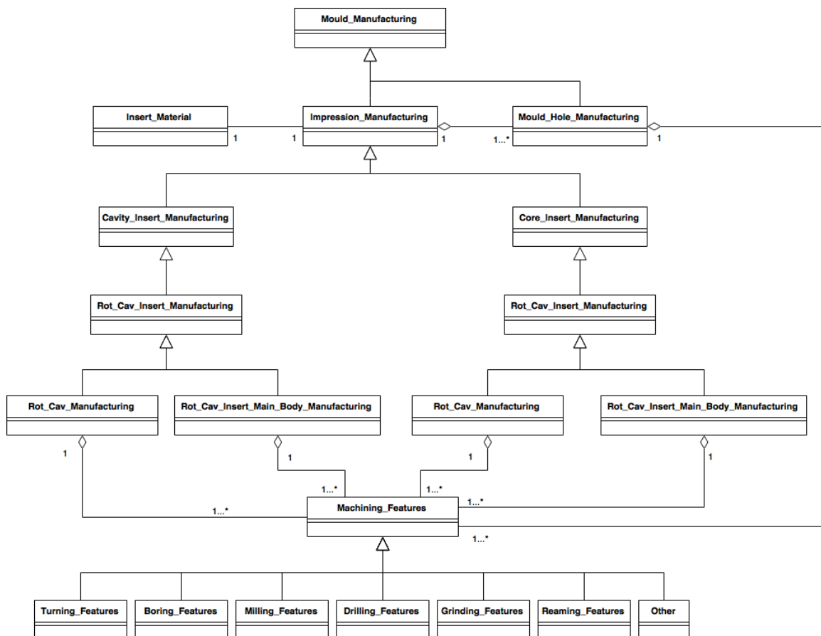
Figure 51 Mould manufacturing data structure.
