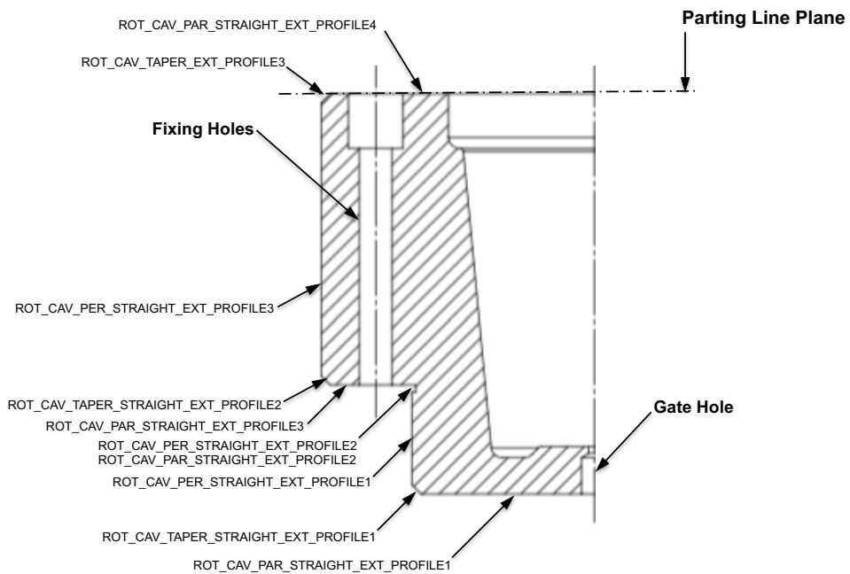
Figure 47 Cavity insert main body geometry information.
