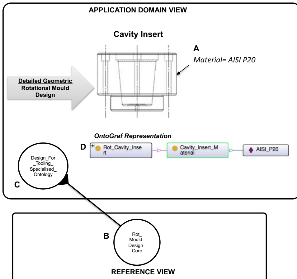
Figure 62 Simple Instantiation Approach.
