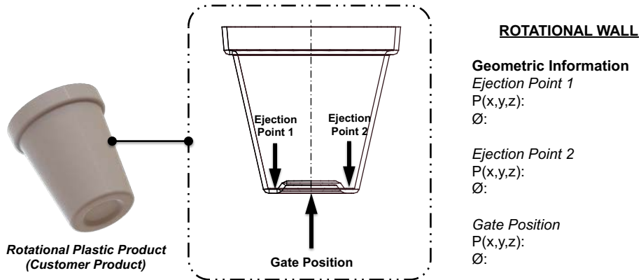
Figure 31 Gate and Ejection Features in Plastic Injected Products.
