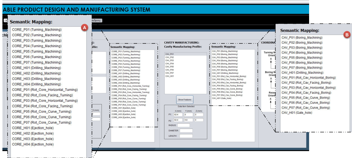
Figure 147 Detailing of the Design for Machining semantic mapping visualisation in the IPDMS
