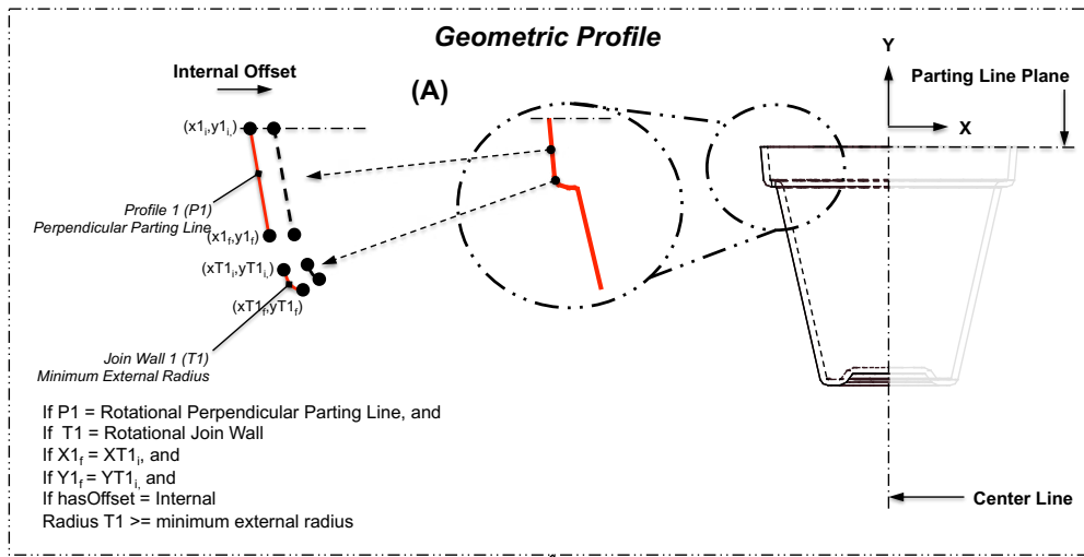
Figure 77 Semantic rule for the relationships between Fillet Feature and Rotational Joint Wall for the minimum external radius.
