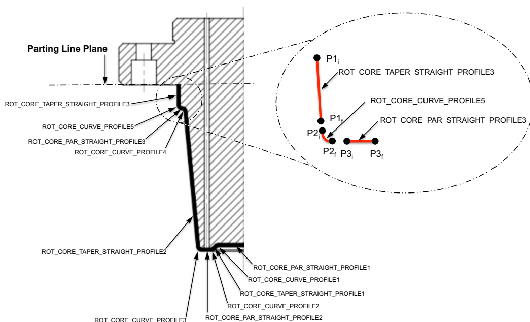
Figure 41 Core insert geometry information.
