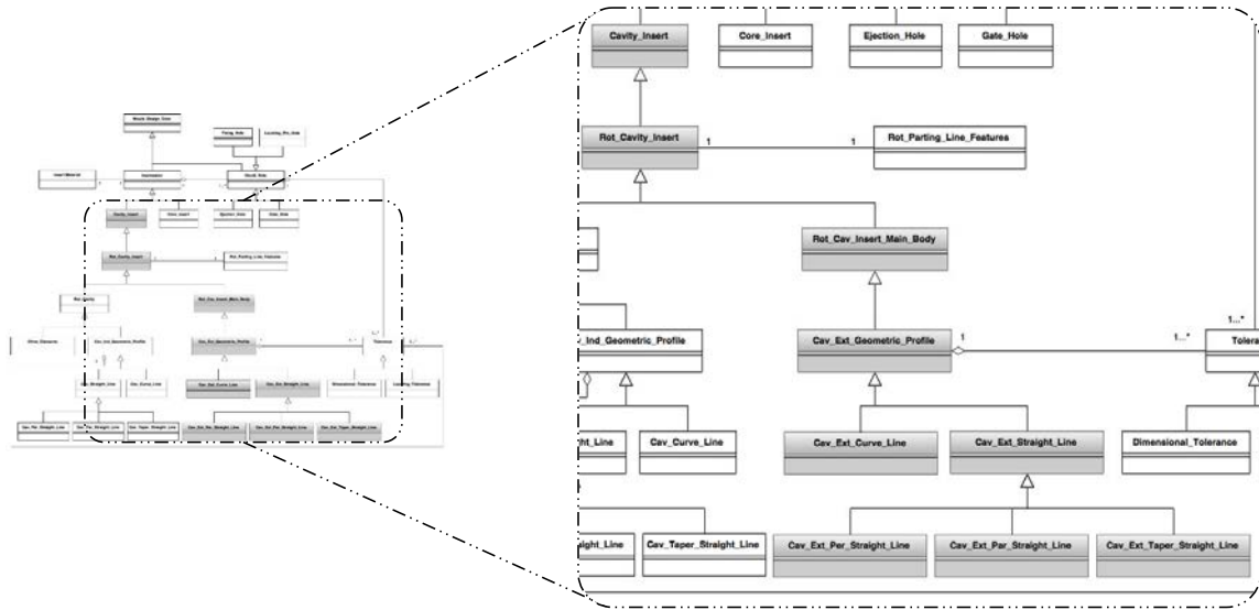
Figure 46 Detail of cavity insert geometric information in the data structure.
