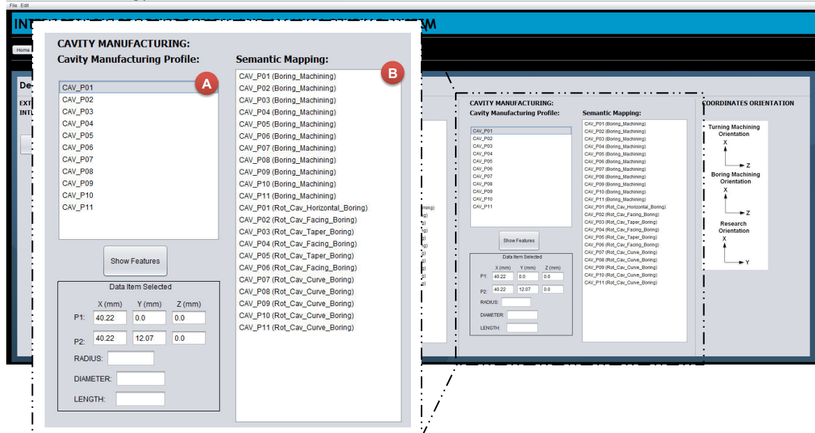
Figure 162 Results of the Rotational Cavity translation (Rotational Cavity Manufacturing).
