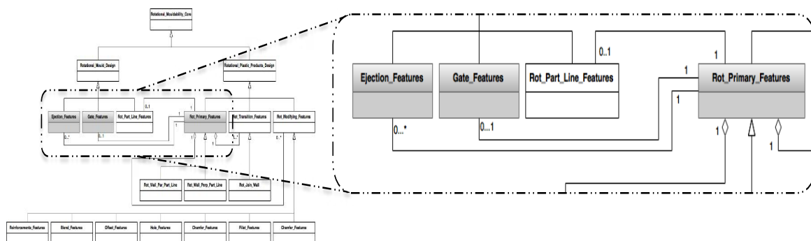
Figure 30 Relationships between rotational primary features and gate features and primary features and ejection features.
