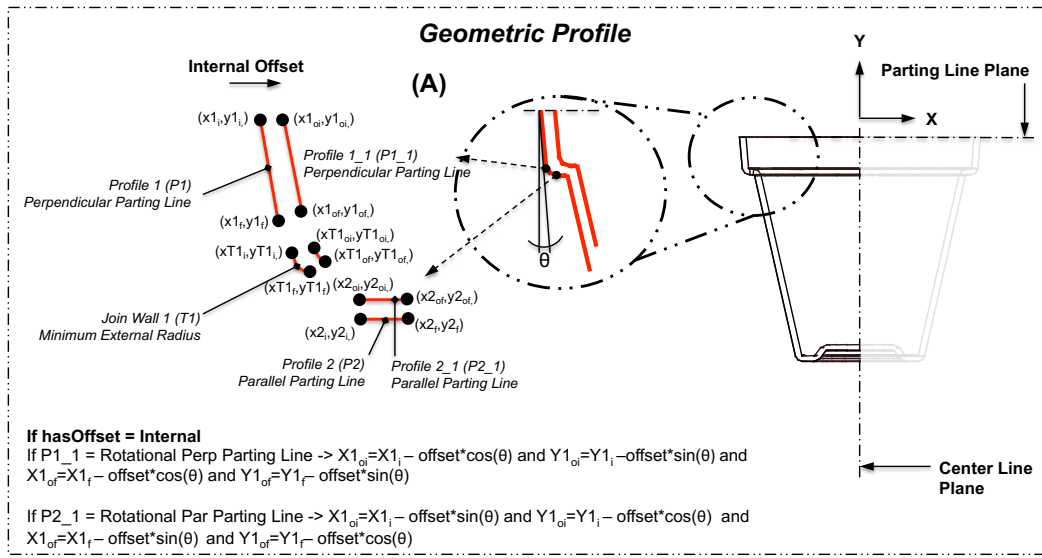
Figure 79 Semantic rule for the relationships between Primary features and Primary features with offset for the internal direction.
