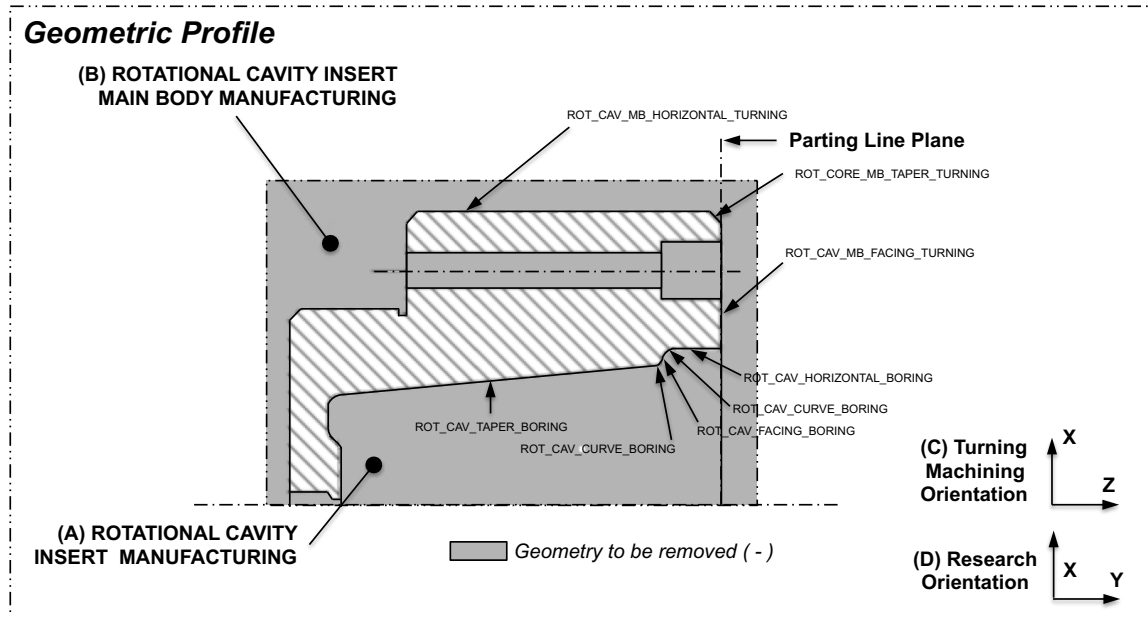
Figure 91 Rotational Cavity Insert Manufacturing Information Detailing.
