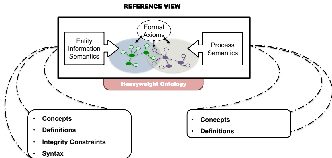
Figure 23. Structure of the Reference View Core Ontologies
