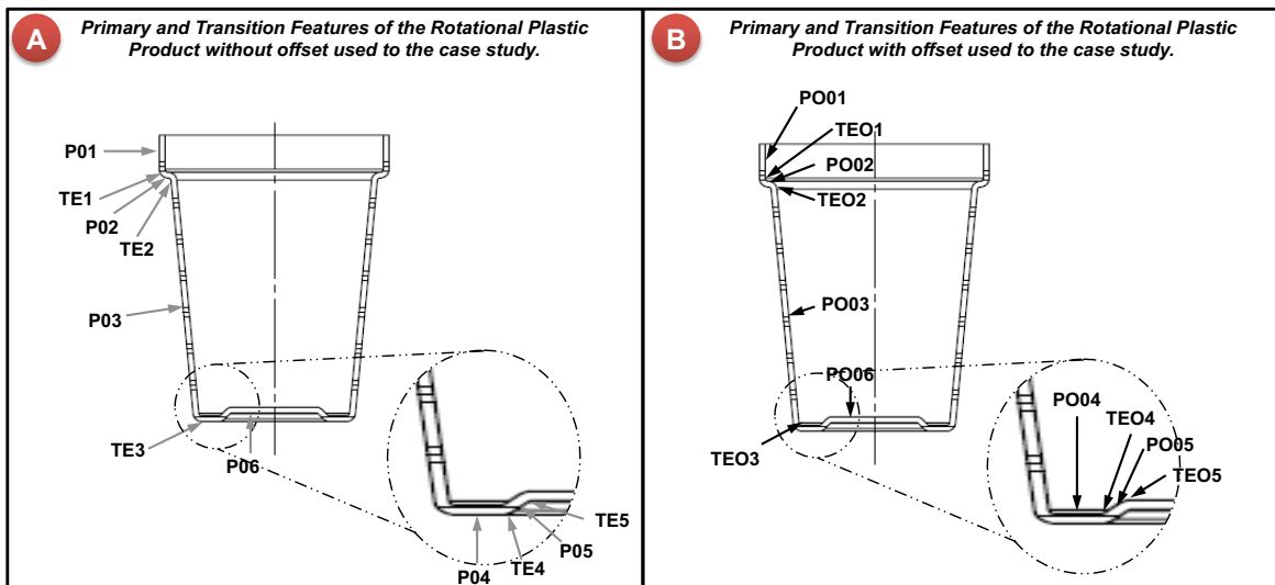
Figure 152 Representations of the Primary and Transition Features in the Product Part Model.
