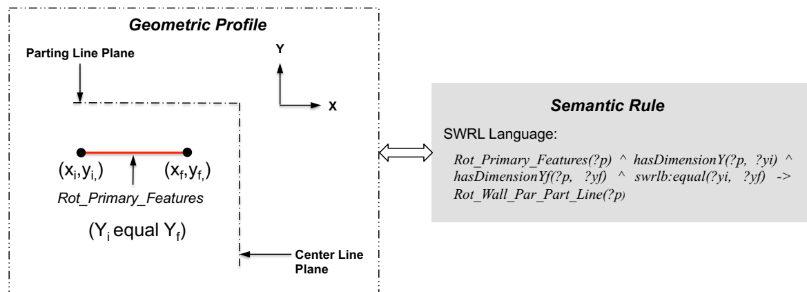
Figure 71 Semantic rule between Rotational primary features(?p) and Rotational wall parallel to the Parting Line.
