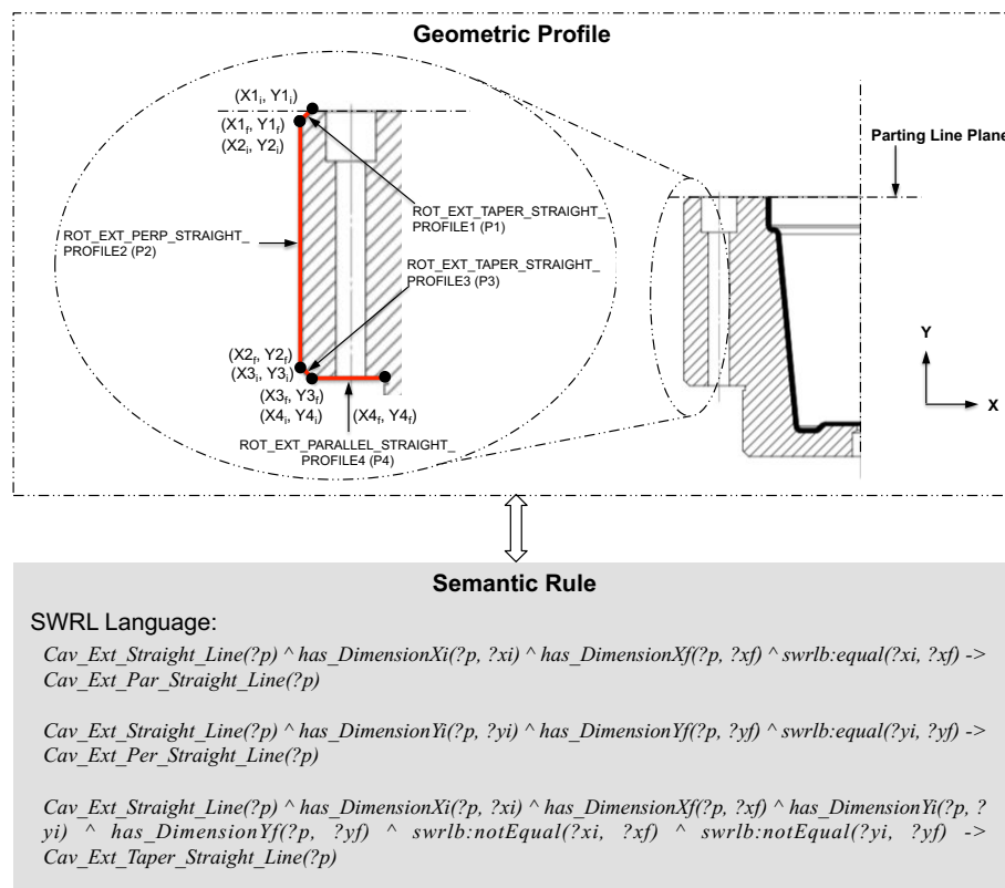
Figure 84 Semantic rule for the relationships between the External profile of the Cavity insert straight line with perpendicular, parallel and taper straight line.
