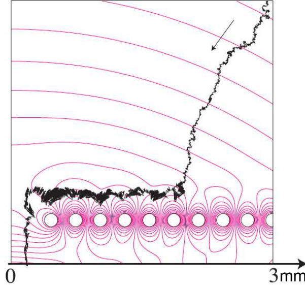
Figure 4.5 – Simulated ^{11}\text{Li}^+ trajectory above the rf-carpet electrodes. The rf-frequency applied on the carpet electrode is 16 MHz at V_{rf} = 190 \text{ V}_{pp} . The superimposed dc gradient is 12 V/cm. The pressure is 146 mbar of He gas at 300 K. Figure from [Takamine 2007].
