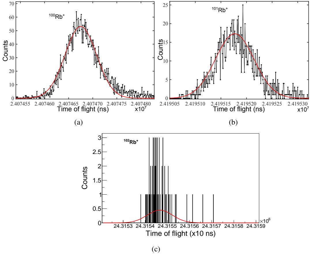
Figure 3.11 – Time-of-flight spectra of ^{100}\text{Rb} (a), ^{101}\text{Rb} (b) and ^{102}\text{Rb} (c). For each time-of-flight spectrum, the number of revolution is 1000. The fit curves are represented in red.
