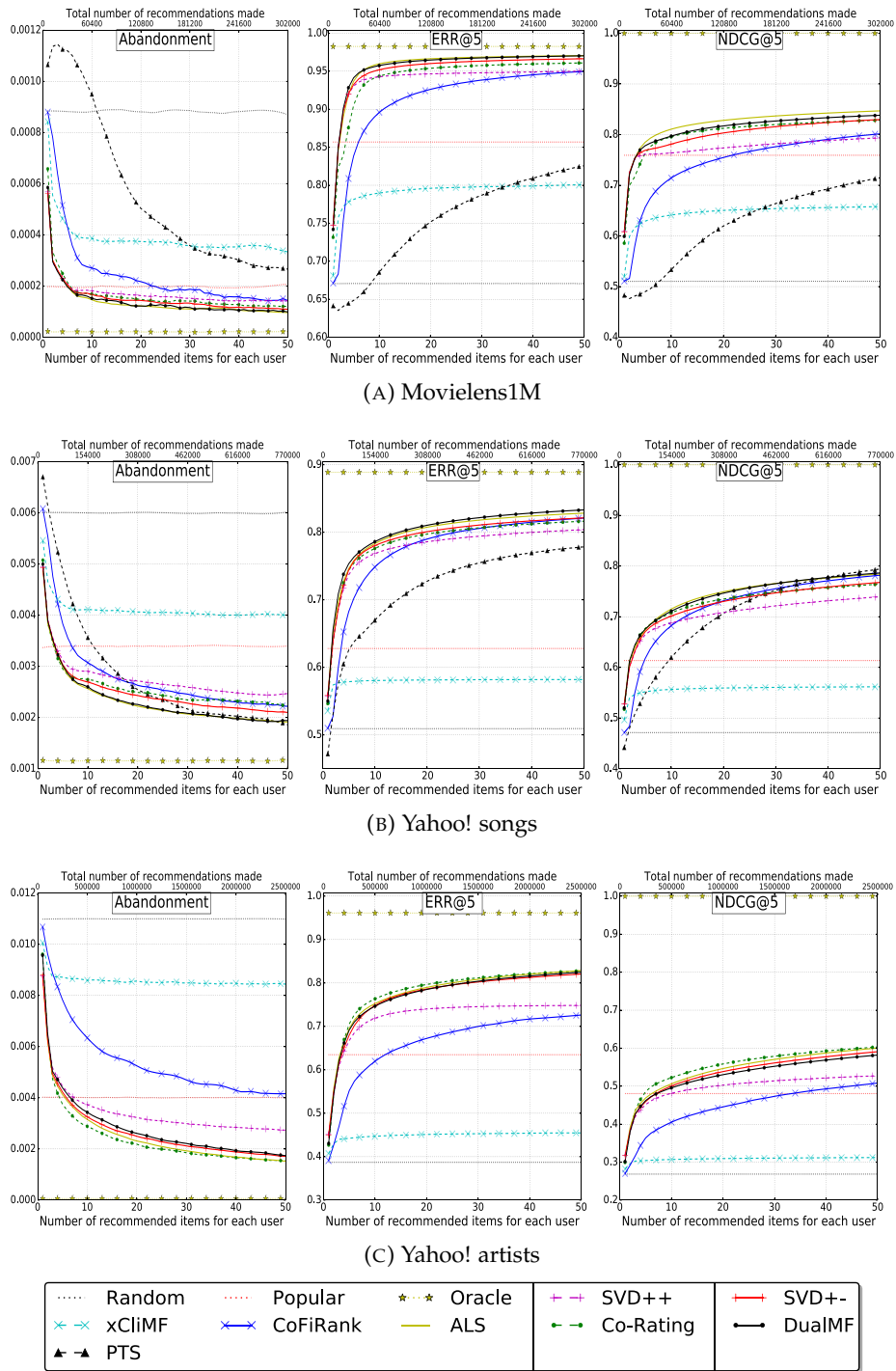
FIGURE 4.4: Evaluation of algorithms on three datasets and three metrics with the informational click model (from the left column to the right one: Abandonment, ERR@5, NDCG@5).
