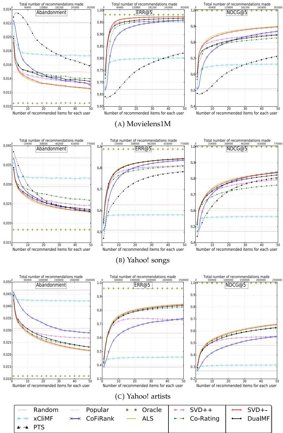
FIGURE 4.5: Evaluation of algorithms on three datasets and three metrics with the almost random click model (from the left column to the right one: Abandonment, ERR@5, NDCG@5).
