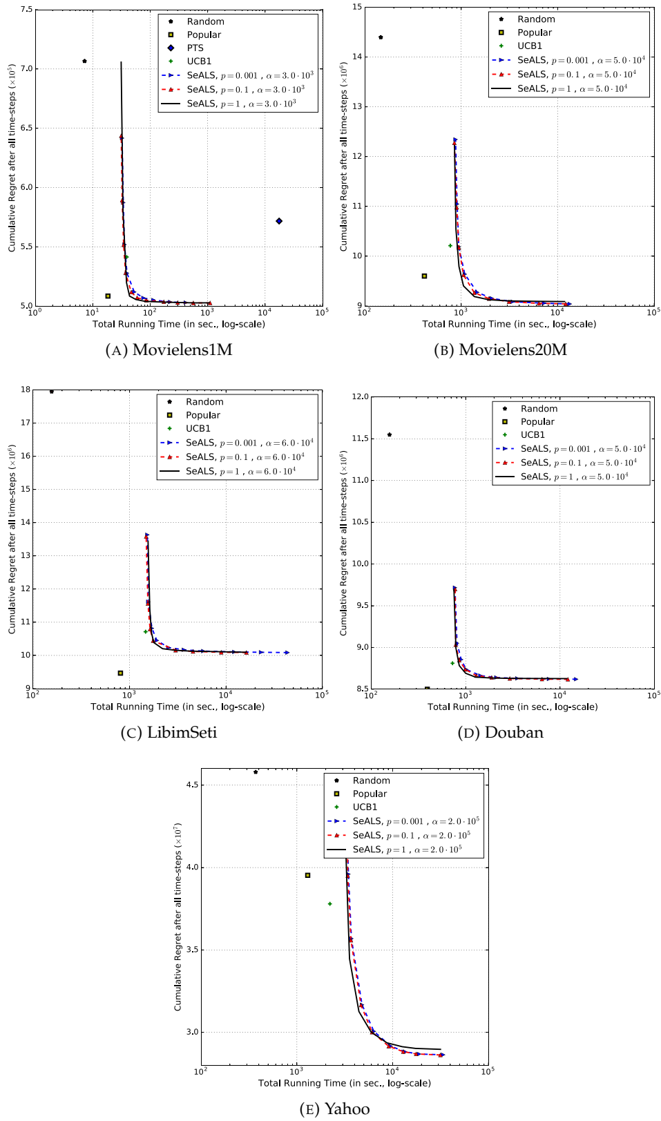
FIGURE 5.5: Impact of the update strategy on the final cumulative regret score when replay is not allowed, evaluated on five datasets.
