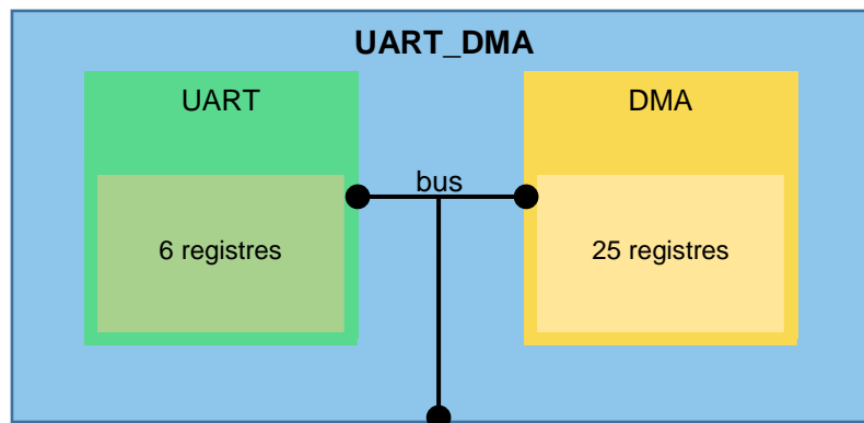
FIGURE 6-1 COMPOSANT UART_DMA
