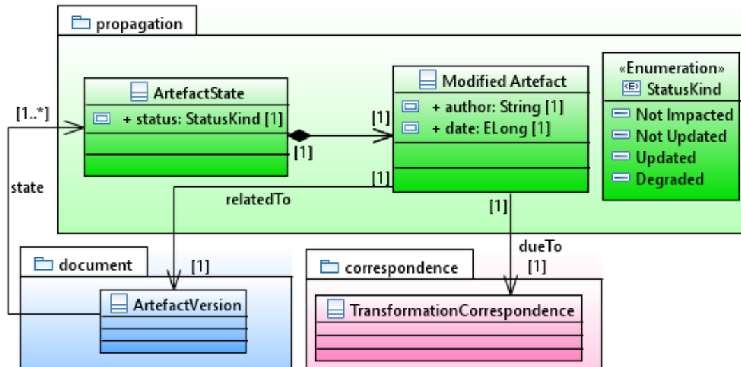
FIGURE 4-8 PAQUETAGE "PROPAGATION"
