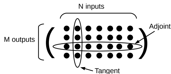
FIGURE 2.3: Computing the Jacobian elements by tangent and adjoint modes
