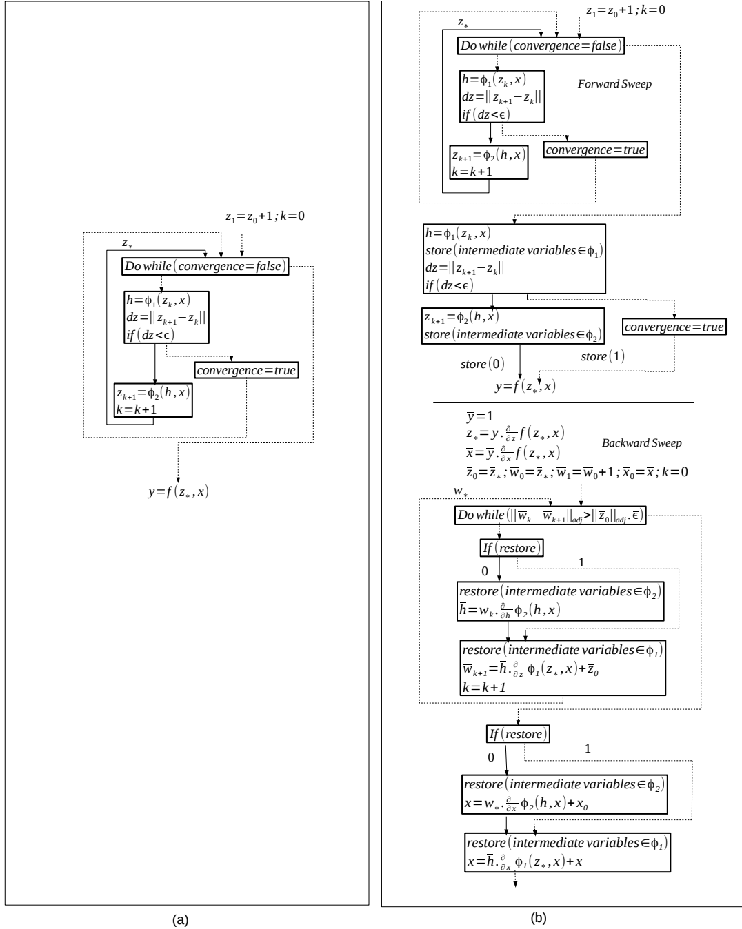
FIGURE 3.10: (a) FP Loop with one exit on the top. (b) Applying the Two-Phases method to the loop Dashed lines show the trajectory followed during run-time.
