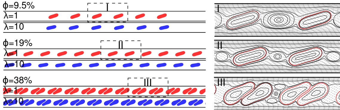
Figure 3.11: Left column: Configurations of a vesicle suspension in the confinement of W = 3.1R . Vesicles form one file in low concentration. Two vesicles couple a doublet in high concentration. Right column: The structure of the flow field in region I, II and III. \phi is the vesicle concentration (area fraction in 2D). The recirculation between two vesicles decreases when concentration increases as shown in region I and II.
