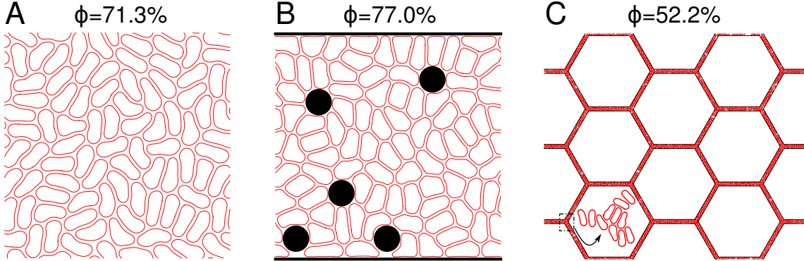
Figure 2.10: Some cases of the initialization of RBCs in high concentration situation. \phi is RBC concentration (area fraction). A: In the periodic domain. B: In a wall bounded channel with some obstacles. The black region means obstacles. C: In a network.
