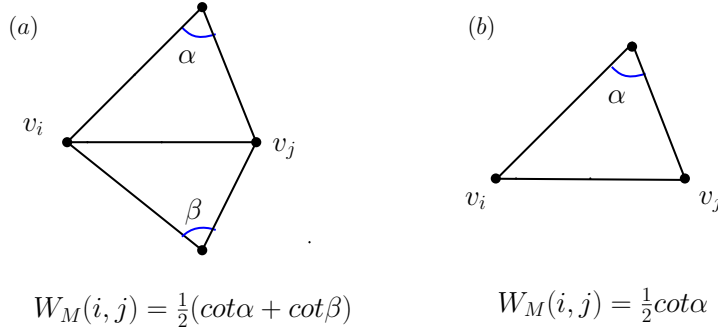
Figure 5.2: (a) W_M(i, j) for an edge (v_i, v_j) that is shared by two triangles. (b) W_M(i, j) for a boundary edge that belongs to a single triangle. If v_i, v_j are not connected by an edge, then W(i, j) = 0 . Notice that in a mesh, an edge is at most shared by two triangles.
