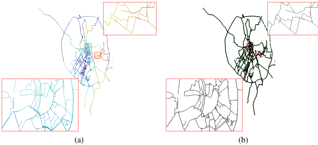
Figure 3.16: GPS data - (a) The distance functions d on each connected components. The value increases from cold to warm colors. (b) The reconstructed \alpha -Reeb graph.
