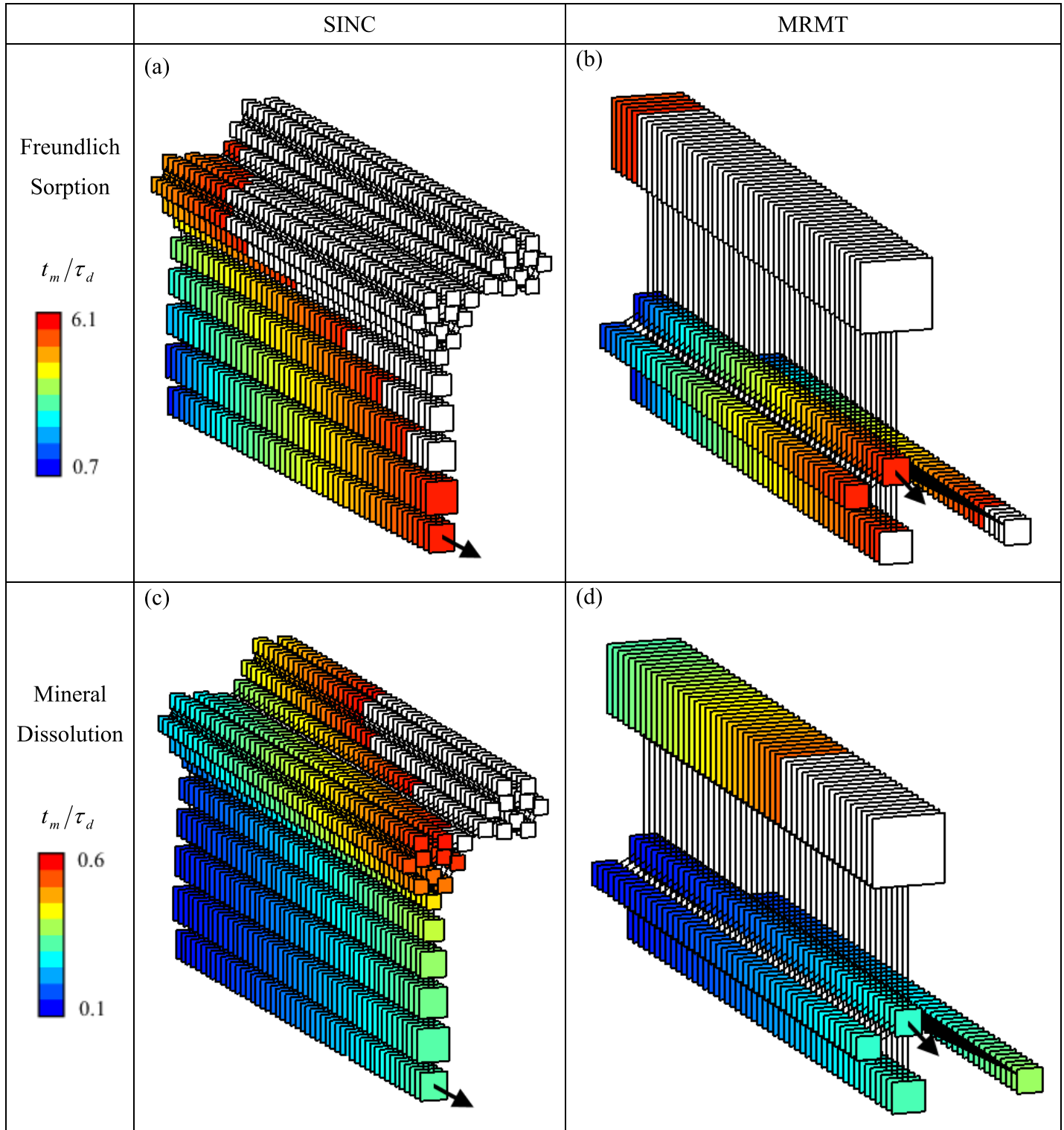
Figure 2. Mobilization times t_m/\tau_d (section 2.5) for the Freundlich sorption (equation (9)) and the mineral dissolution (equation (10)) with Da = \tau_d/\tau_r = 10 and s^0/k = 1 , for the SINC dissolution pattern (Figure 1d) and its equivalent MRMT model represented by its four zones with the largest porosities (out of 25), depicted as cross sections transverse to the mobile zone identified by the arrow. For the MRMT of the right column, the distances between the mobile and immobile zones are proportional to \log(1/\alpha_i) , and the porosities of the mobile and diffusive zones are proportional to the area of the cells.
