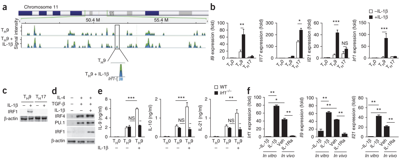
Figure 1 IRF1 controls the secretion of T_H9 -related cytokines. (a) RNA-seq analysis of genes on chromosome 11 (top row) in T_H9 cells differentiated for 1 h from sorted naive CD4^+CD62L^{hi}CD44^{lo} T cells with (bottom row) or without (middle row) IL-1 \beta in the presence of anti-CD3 and anti-CD28; signal intensity is presented as the sum of two separate 'reads' (blue and green). M, megabases (position on chromosome 11). Below, enlargement of Irf1 region, showing its expression in both conditions (blue vertical rectangles indicate the Irf1 reference sequence (exon-intron)). (b) RT-PCR analysis of Il9 , Il17 , Il21 and Irf1 mRNA in T_H0 , T_H9 or T_H17 cells differentiated for 48 h ( Il9 , Il17 and Il21 ) or 1 h ( Irf1 ) relative to naive CD4^+ T cells with (+) or without (-) IL-1 \beta ; results were normalized to the expression of mouse Actb (encoding \beta -actin) and are presented relative to those of control T_H0 cells differentiated without IL-1 \beta . (c) Immunoblot analysis of IRF1 in T_H9 or T_H17 cells differentiated for 24 h from naive CD4^+ T cells with or without IL-1 \beta ; \beta -actin serves as a loading control throughout. (d) Immunoblot analysis of IRF1, IRF4 and PU.1 in cells differentiated for 24 h from naive CD4^+ T cells in the presence (+) or absence (-) of IL-4, TGF- \beta and/or IL-1 \beta (above lanes). (e) Enzyme-linked immunosorbent assay (ELISA) of IL-9, IL-10 and IL-21 in supernatants of T_H0 cells or T_H9 cells differentiated for 3 d from wild-type (WT) or Irf1 -/- naive CD4^+ T cells with or without IL-1 \beta . (f) RT-PCR analysis of Irf1 , Il9 and Il21 in T_H9 cells induced in vitro with or without IL-1 \beta ( In vitro ) and in CCR3^+CXCR3^+CCR6^+CCR4^-CD4^+ T cells sorted from the tumor-draining lymph nodes of wild-type mice 8 d after intravenous injection of B16-F10 melanoma cells and treatment with IL-1R antagonist (IL-1Ra) or Vehicle (Veh) ( In vivo ); results normalized as in (b) and presented relative to those of T_H0 cells, set as 1. NS, not significant; * P < 0.05 , ** P < 0.01 and *** P < 0.001 (Mann-Whitney test (b,e) or Kruskal-Wallis test (f)). Data are from one experiment representative of at least two independent experiments with similar results (mean and s.e.m. of triplicates (b,e) or three biological replicates (f)).
