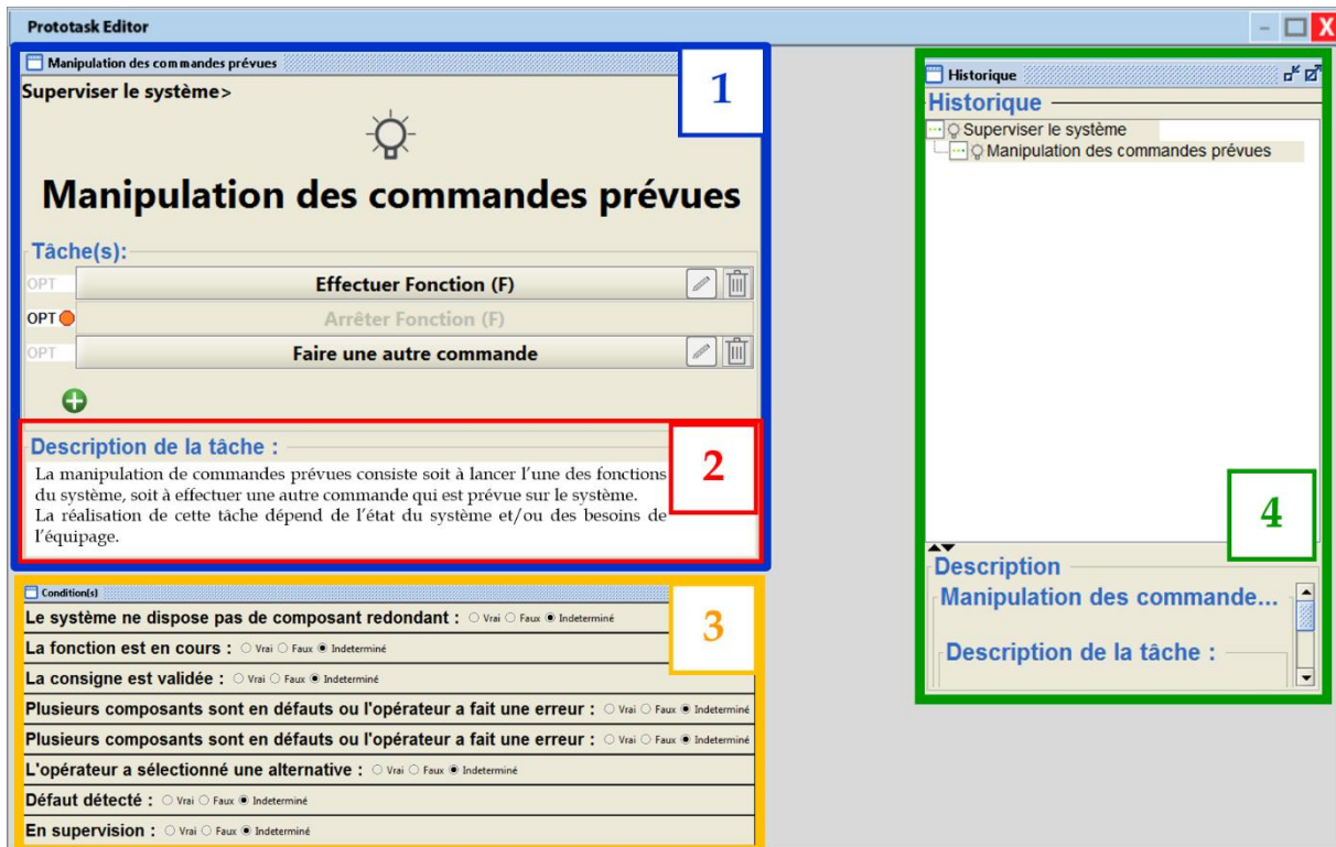
Figure 111 Prototask Editor
