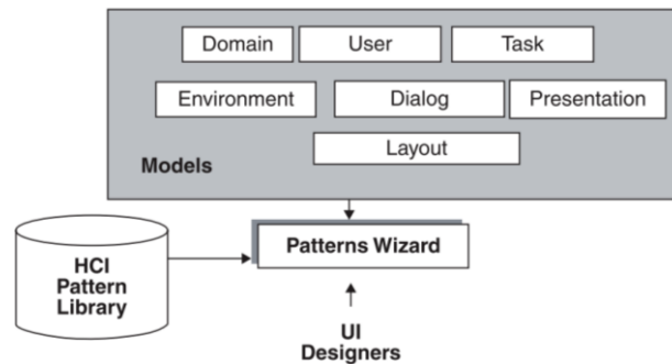
Figure 30 le Framework PD-MBUI (Pattern Driven and Model Based User Interface)
