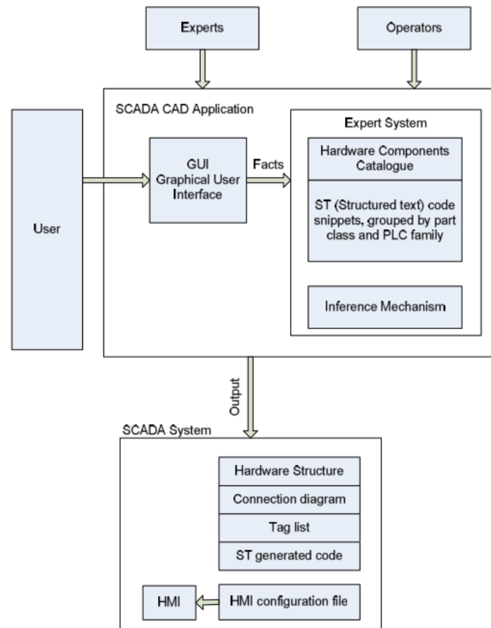
Figure 16 Structure de l'application SCADA CAD
