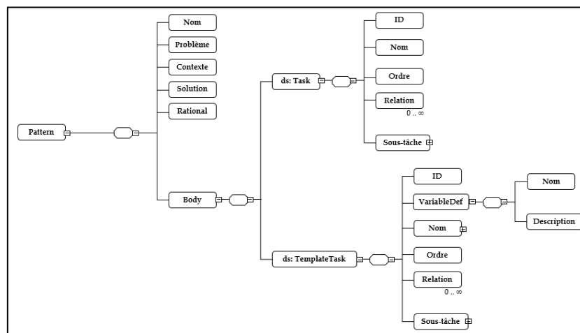
Figure 25 Structure de TPML.
