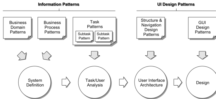
Figure 23 le Framework PSA
