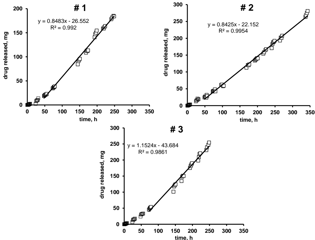
Figure 59: Theory (curves) and experiment (symbols) of diprophylline transport through an initially drug-free Aquacoat:Eudragit NM (20 :80) film in a side-by-side diffusion cell (thickness: # 1 = 48 \mu\text{m} , # 2 = 32 \mu\text{m} , # 3 = 51 \mu\text{m} ).
