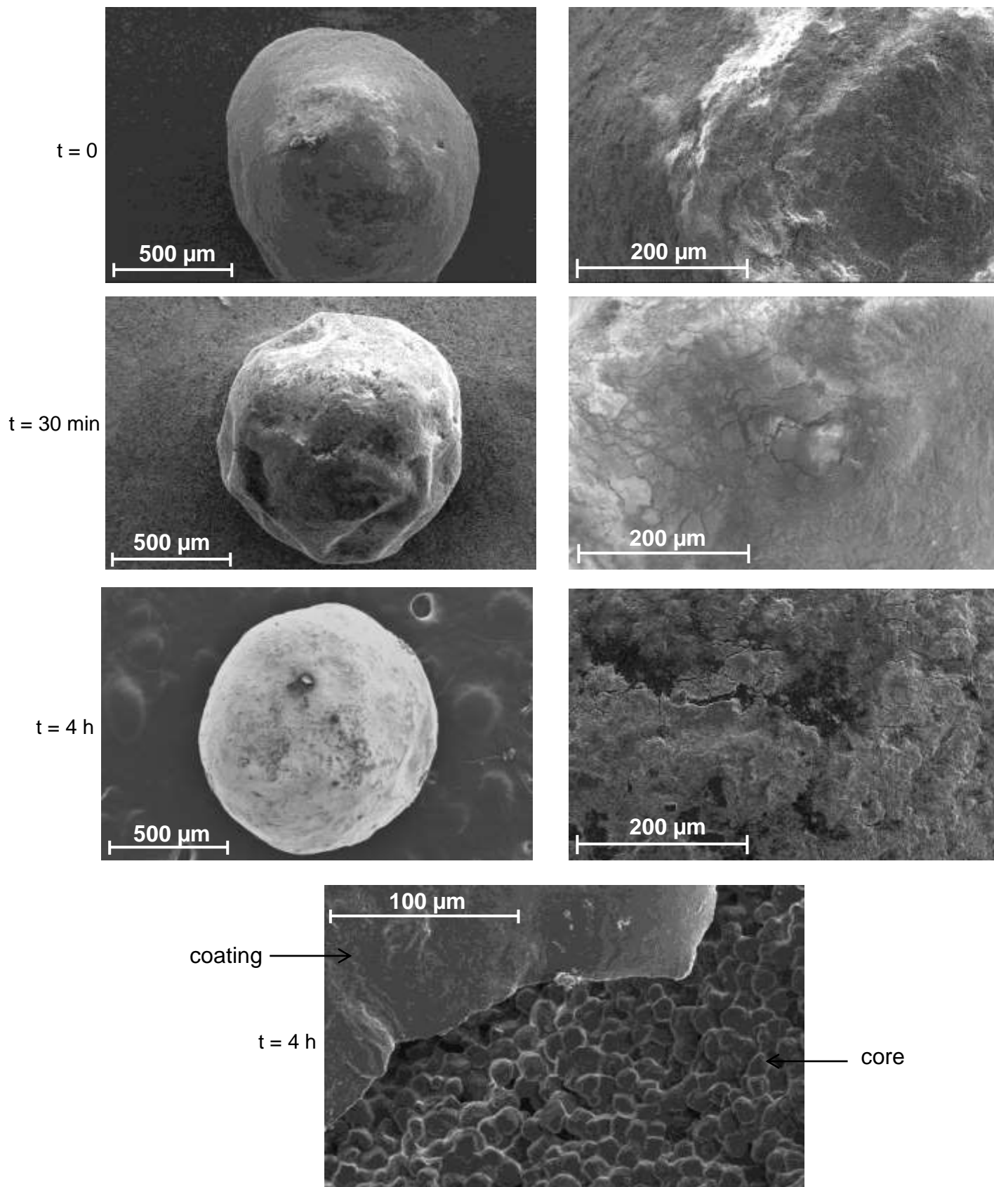
Figure 42: SEM pictures of surfaces of Kollicoat SR-coated pellets before and after 30 min or 4 h exposure to phosphate buffer pH 7.4 (as indicated) (drug loading: 10 %, coating level: 10 %). The SEM picture at the bottom shows parts of the coating and of the core of a pellet (that had been exposed for 4 h to the release medium and accidentally damaged during sample preparation).
