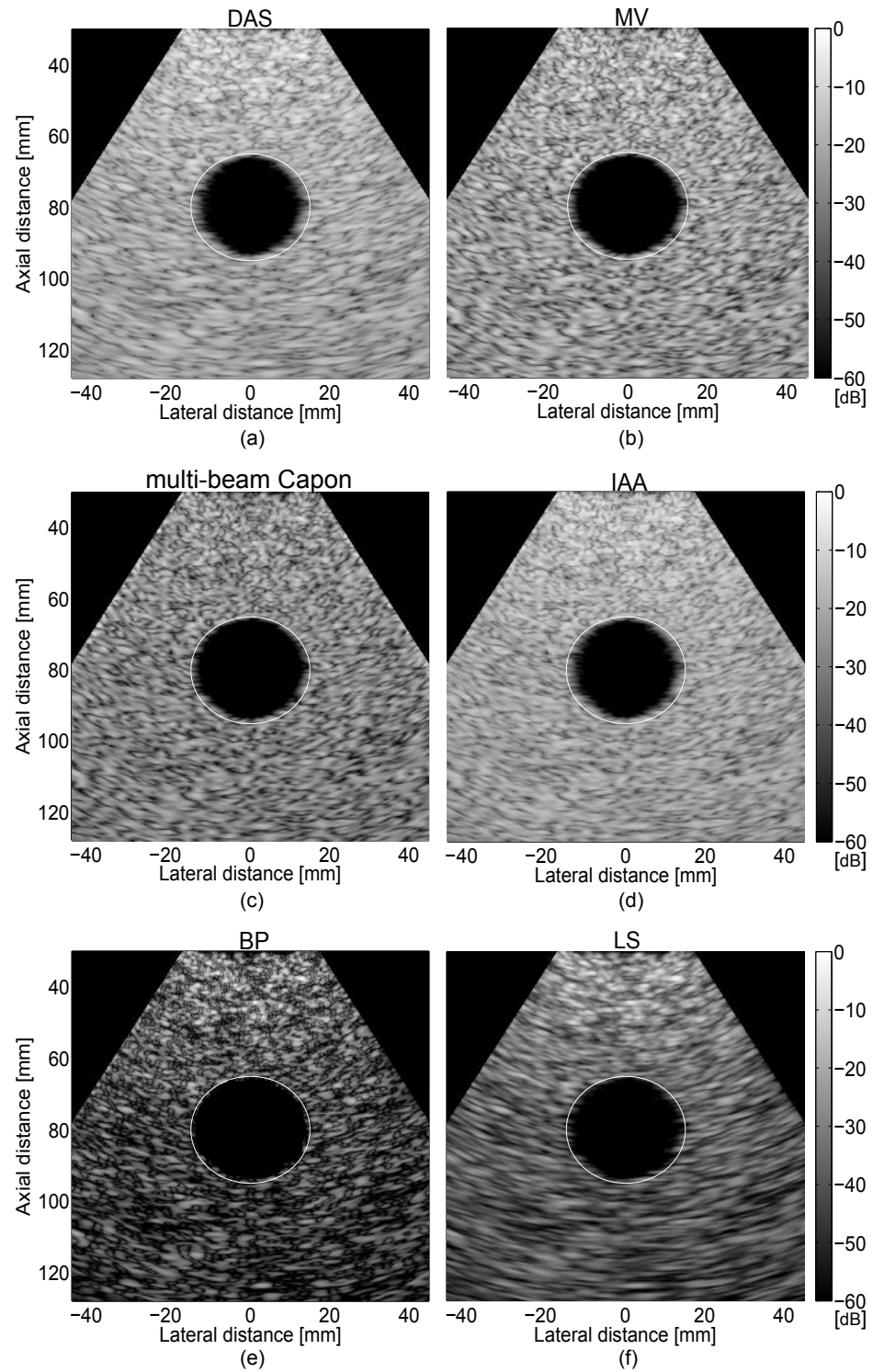
Figure 4.6: (a) DAS, (b) MV, (c) multi-beam Capon, (d) IAA, (e) BP, and (f) LS BF results of the hypochoic cyst simulation.
