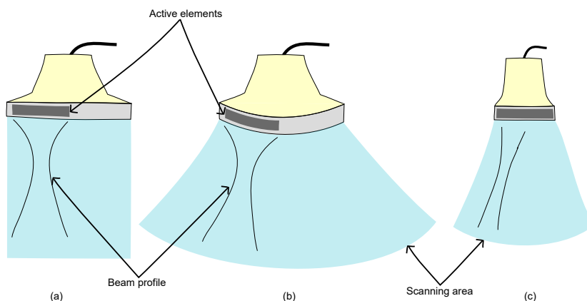
Figure 1.5: Principle of electronic sweeping with (a) linear array, (b) convex array, and (c) phased array.
