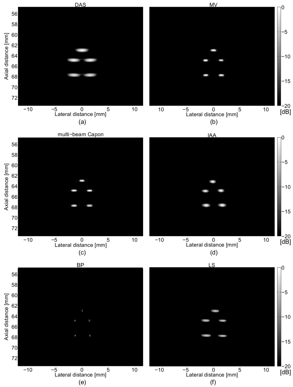
Figure 4.2: (a) DAS, (b) MV, (c) multi-beam Capon, (d) IAA, (e) BP, and (f) LS BF results of the simulation of individual point scatterers.
