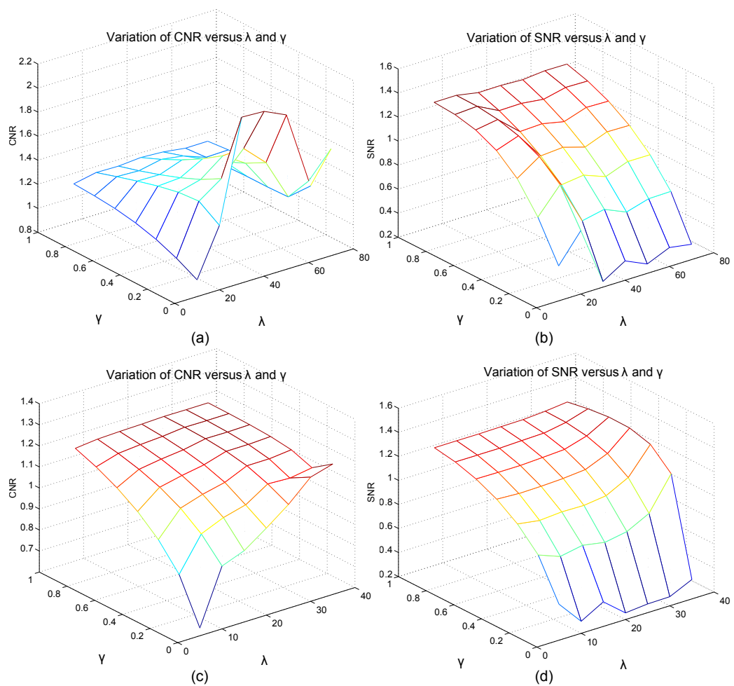
Figure 3.7: The variation of the CNR and SNR versus the parameters \lambda and \gamma when USBIC BF method ((a) and (b)), and M-USBIC BF method ((c) and (d)) are applied to the cardiac view simulation detailed in the Section 3.3.3
