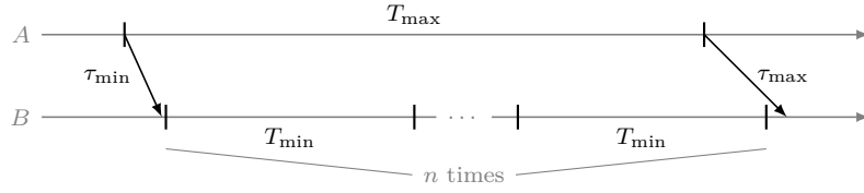
(a) Each execution of B samples the first message sent by A .
