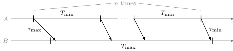
(b) All messages sent by A are overwritten by the last one.
