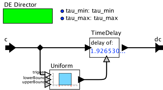
Figure 3.11: Ptolemy model of transmission delays (delay).
