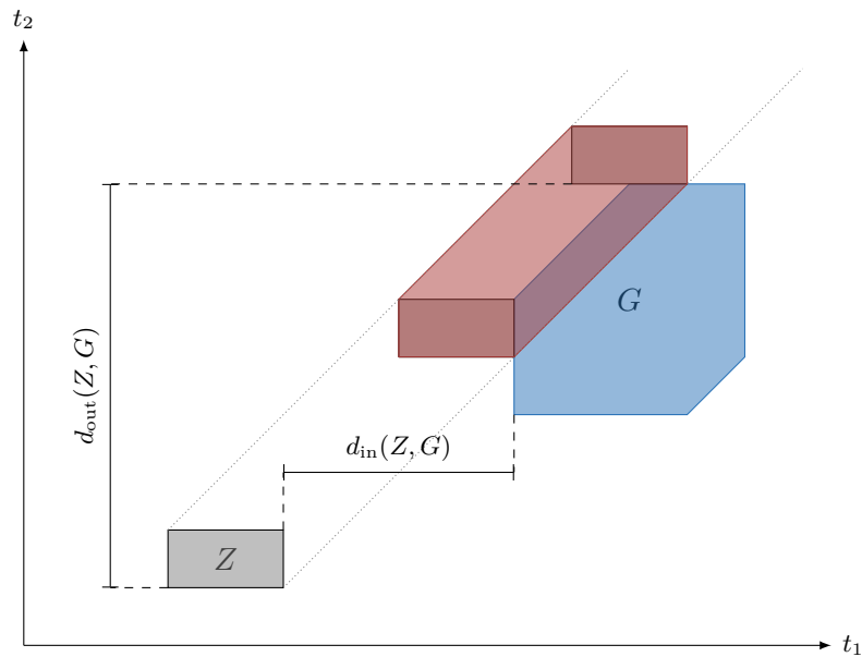
Figure 6.5: Activation and deactivation distances of a guard G from an initial zone Z . The red region is the zone where the guard is enabled.
