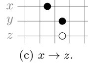
Figure 4.10: A real-time trace that is not unitary discretizable ( x \xrightarrow{1} y \xrightarrow{0} z \xrightarrow{0} x ) and that may occur whenever \tau_{\max} > 0 .
