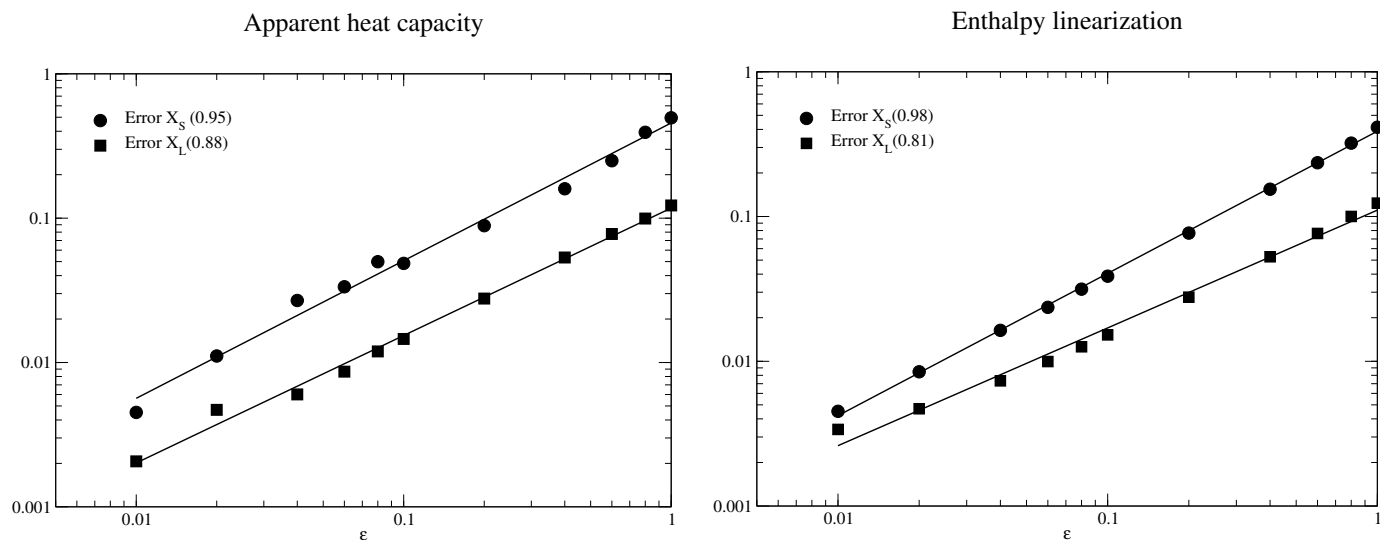
FIGURE 4.3: The errors on the fronts positions as functions of \epsilon for the apparent heat capacity and the enthalpy linearization.
