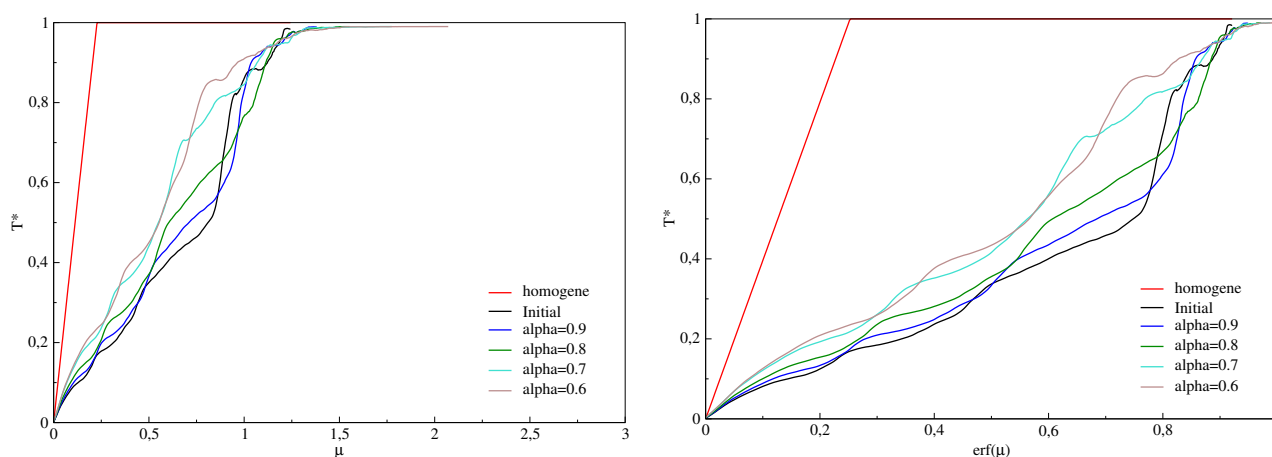
FIGURE 5.29: Mean dimensionless temperature at t = t_{end} as a function of the similarity variable (left) and as a function of \text{erf}(\mu) (right).
