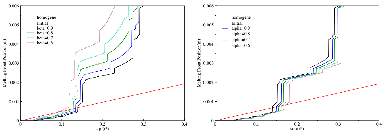
FIGURE 5.43: Evolution of the melting front's position as a function of \sqrt{t^*} for KD1 for various \beta (left) and various \alpha (right).
