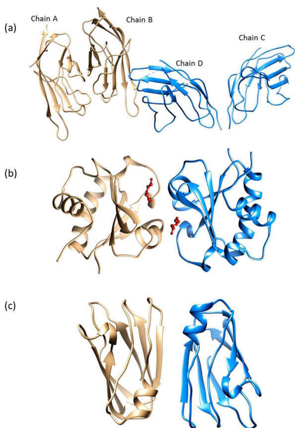
Figure 6. Typical examples of Dockground biological assemblies predicted crystallographic by IChemPIC. (A) CTLA-4 (chains A, B) / B7-2 (chains C, D) complex (PDB ID 1i85); (B) human phosphatidylinositol 3-kinase-like protein 2 with bound PEG molecules (red ball and sticks) at the interface (PDB ID 3evi); (C) plastocyanin from the cyanobacterium Synechocystis sp. PCC 6803 (PDB ID 1pcs).
