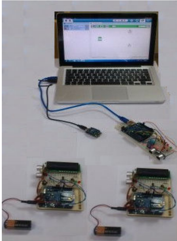
Figure 4.14. Platforme d' experimentation
