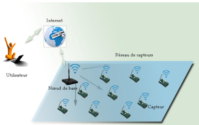
Figure 1.1 Architecture __ d'un RCSF
