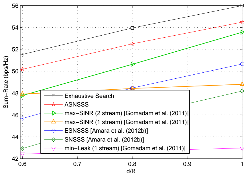
Figure 4.15: Scenario 2.3: Sum-Rate vs d/R between 0.6 and 1
