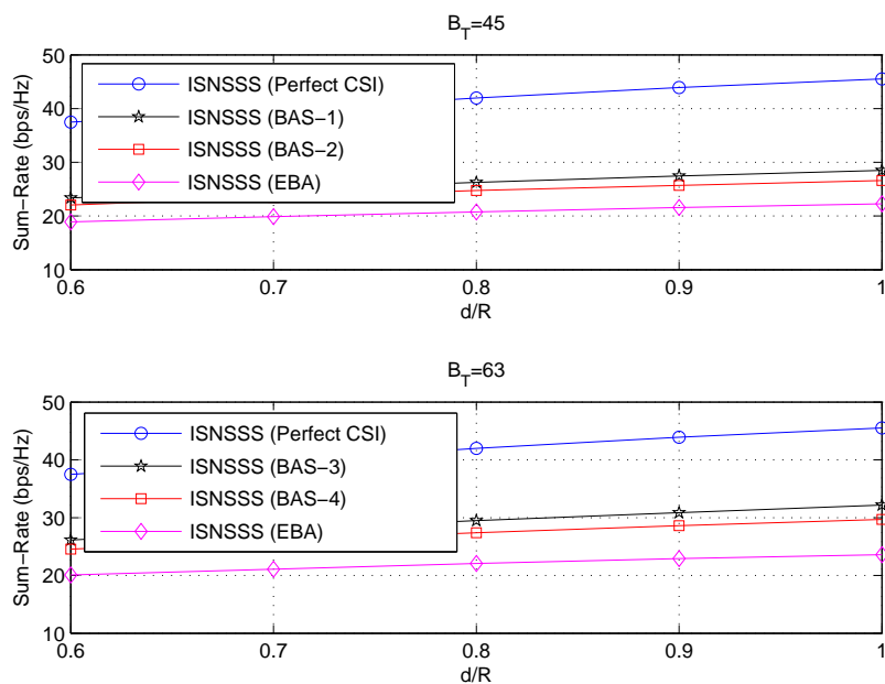
(b) Comparisons for the ISNSSS algorithm.
