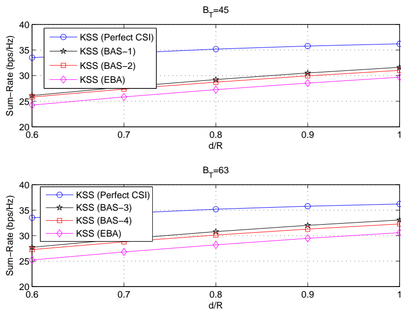
(a) Comparisons for KSS algorithm.
