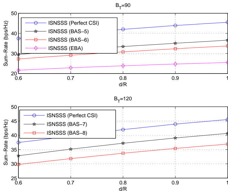
(b) Comparisons for the ISNSSS algorithm.
