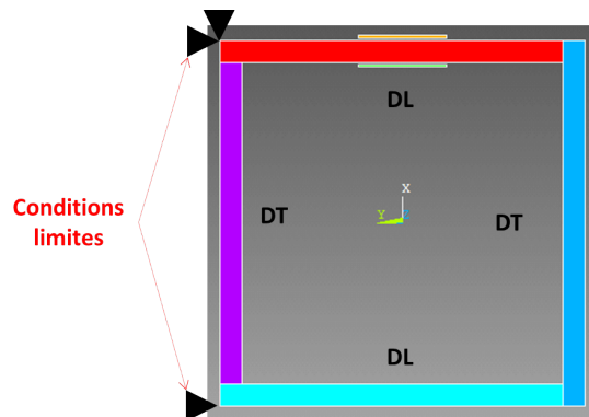
FIGURE 5.2.14 – Conditions limites mécaniques
