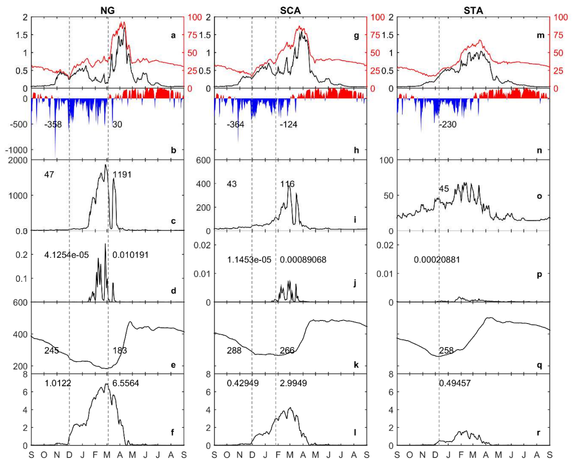
Figure 10: Conditions of the onset of the blooms in each region. Row 1. Average integrated chlorophyll in red ( mgChl.m^{-2} ) and surface chlorophyll in black ( mgChl.m^{-3} ). 2. Heat flux ( W.m^{-2} ). 3. MLD (m) 4. Turbulence average in the upper 75m ( m^2.s^{-1} ). 5. Integrated zooplankton biomass
