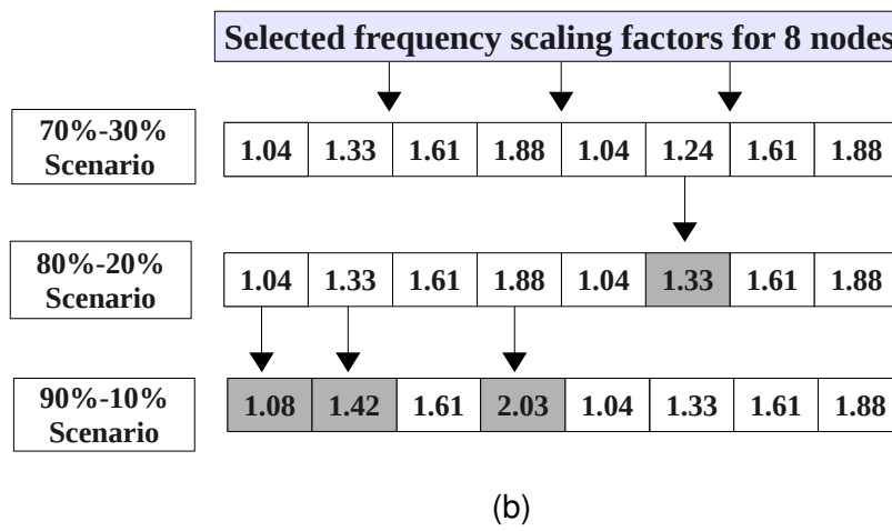
Figure 3.5: (a) Comparison the results of the three power scenarios and (b) Comparison the selected frequency scaling factors of MG benchmark class C running on 8 nodes
