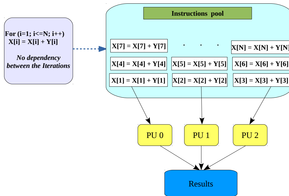
Figure 1.5: Loop-level parallelism
