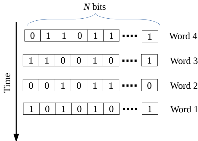
Figure 1.1: Bit-level parallelism
