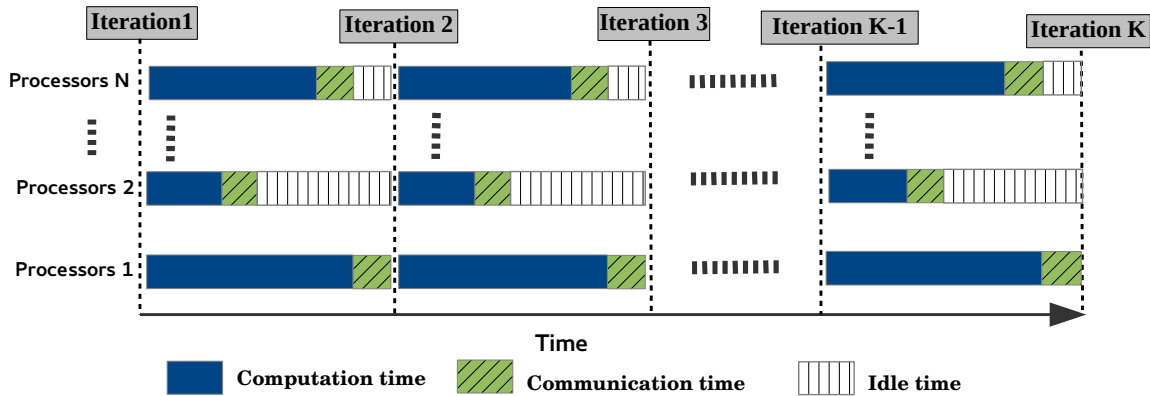
Figure 1.14: The SISC Model
