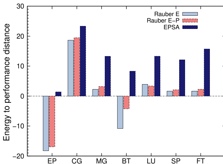
Figure 2.5: Comparing our method to Rauber and Runger's methods
