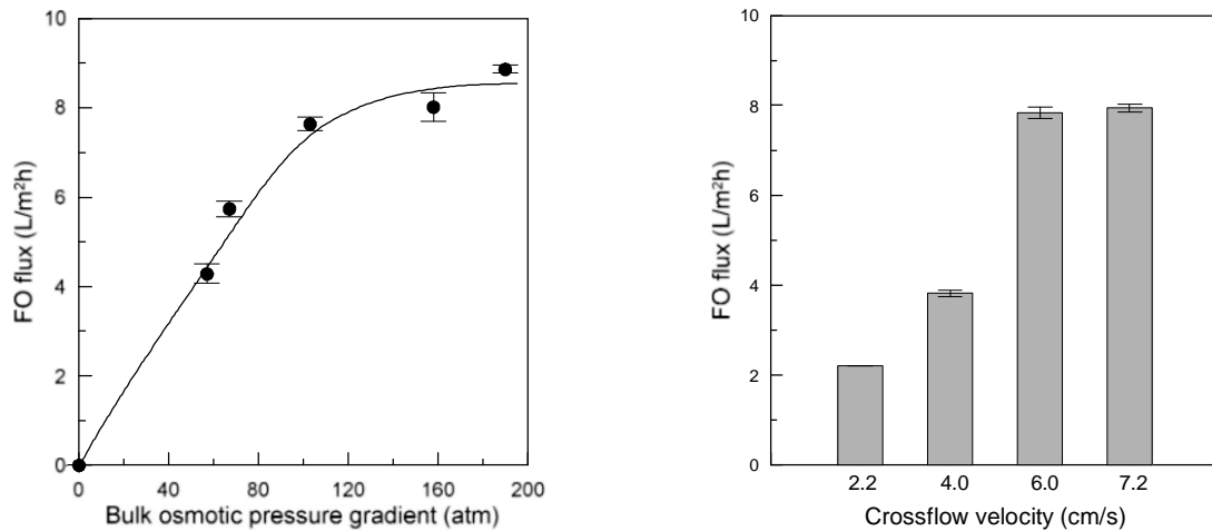
Figure 5: Effect of a) osmotic pressure gradient (feed: pure water; crossflow velocity: 6 cm/s) and b) crossflow velocity (feed: pure water; \pi_b^0 = 103 bar).
