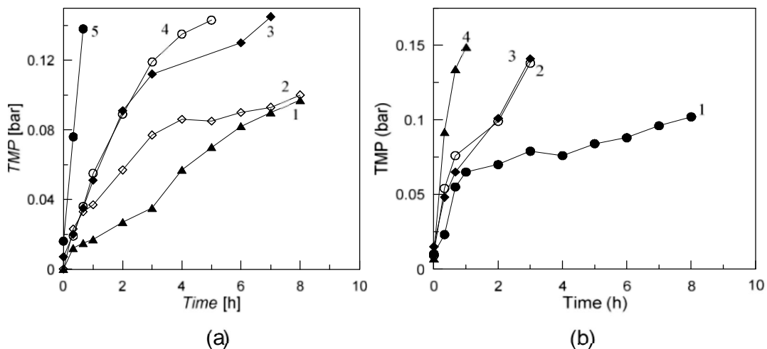
Figure 9: Operational stability of a) \text{Xyl}^{\text{SP}} (0.3 mg/mL wheat arabinoxylan feed, 17 \text{L}/\text{m}^2\cdot\text{h} flux at 25°C) and b) \text{Pcet}^{\text{SP}} (0.3 mg/mL pectin, 17 \text{L}/\text{m}^2\cdot\text{h} flux at 40°C). Numbers on the Figure represent the cycle number.
