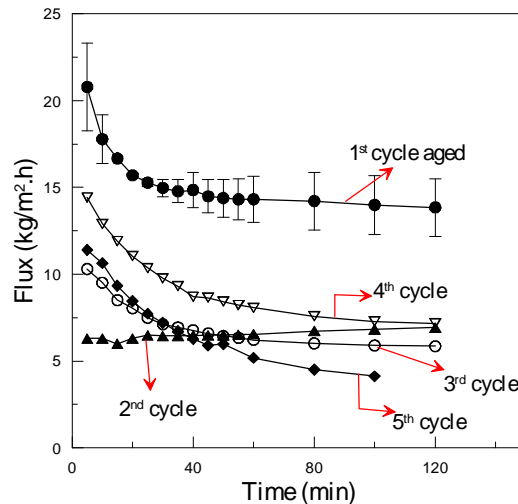
Figure 8: the membrane is subjected to a multi-cyclic ageing of the membrane in 2000 ppm solution at pH 12 with intermediate fouling using 0.3 mg/mL pectin. The flux in this figure therefore represents the flux obtained during a 2 h lasting pectin filtration at 0.25 bar.
