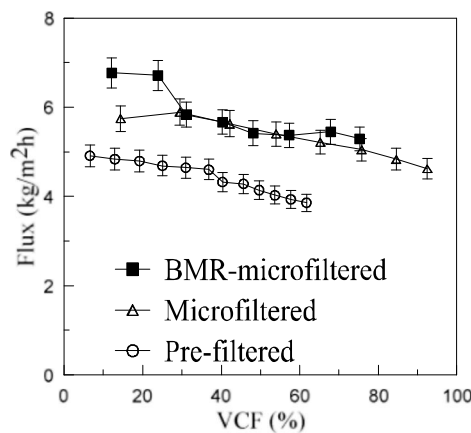
Figure 7: Effect of different pre-treatment methods on FO performance (feed: OMWW; crossflow velocity: 6 cm/s; \pi_b^0 : 103 bar).
