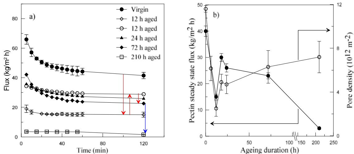
Figure 6: Transmembrane flux of membrane aged in 2000 ppm solution while filtering 0.3 mg/mL pectin at 0.25 bar and b) the steady state pectin flux measured at 0.25 bar from (a) and membrane pore density estimated based on SEM image analysis using Image J.
