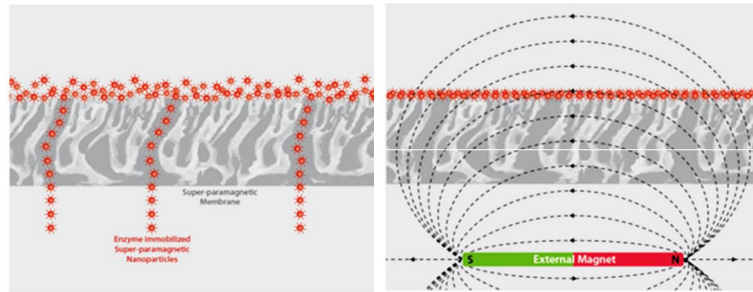
Figure 11: Permeation of an 8 nm NP SP through 0.2 \mu\text{m} diameter pores of an M SP (a) in the absence of an external magnet and (b) in the presence of an external magnet.
