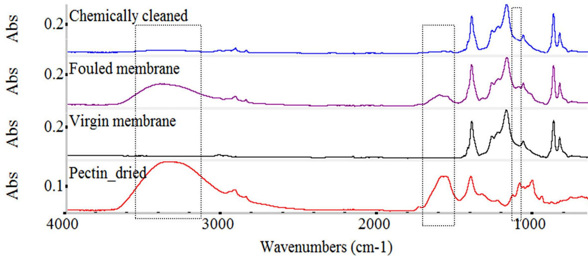
Figure 11: cross-sectional view of a) virgin membrane, b) chemically cleaned membrane and c) ATR-FTIR spectra of virgin, fouled, chemically cleaned membrane and foulants scrapped from the membrane surface. These bands are average of ATR-FTIR analysis taken at three different spots of a membrane.
