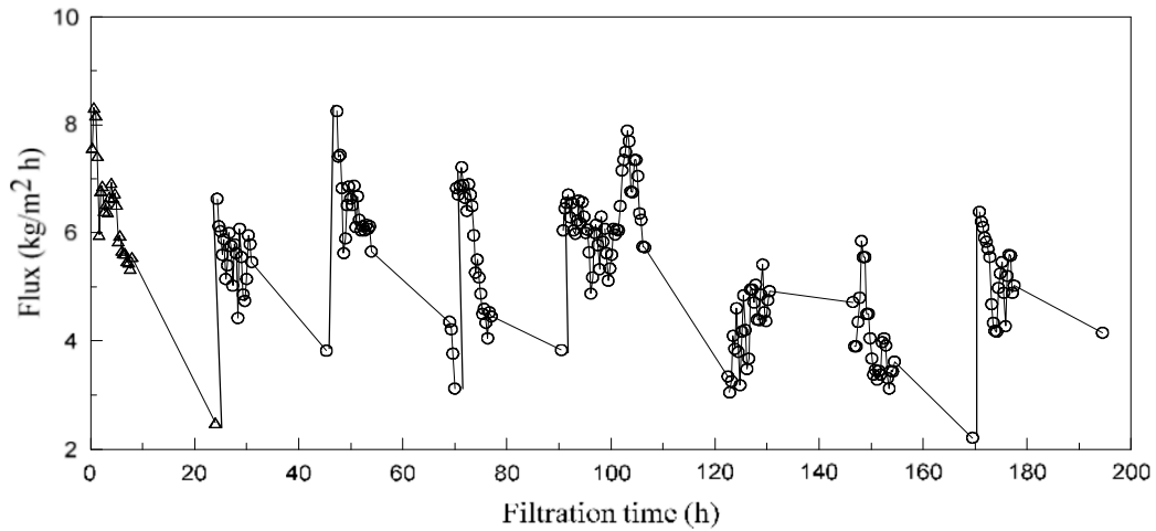
Figure 8: Single step FO performance continuously operated for ten days: OMWW volume; 3 L), DS; 4 L, DS concentration; 3.7 molal \text{MgCl}_2 at 6 cm/s.
