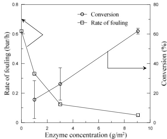
Figure 4: Effect of amount of \text{Enz}^{\text{SP}} deposited per membrane area on the rate of fouling and degree of conversion. The transmembrane flux was fixed at 15 \text{ L/m}^2\cdot\text{h} , temperature 40^\circ\text{C} and pH 4.5.
