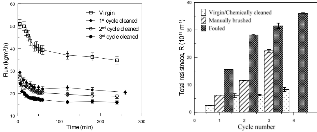
Figure 10: Flux trend of a membrane while filtering 0.3 mg/mL pectin with intermediate static cleaning in 400 ppm NaOCl at pH 12 for 1 h, and b) total resistance of virgin, fouled, manually brushed and chemically cleaned membrane estimated with Equation 2. The resistance was measured by filtering sodium acetate buffer before and after chemical cleaning at 1 bar.
