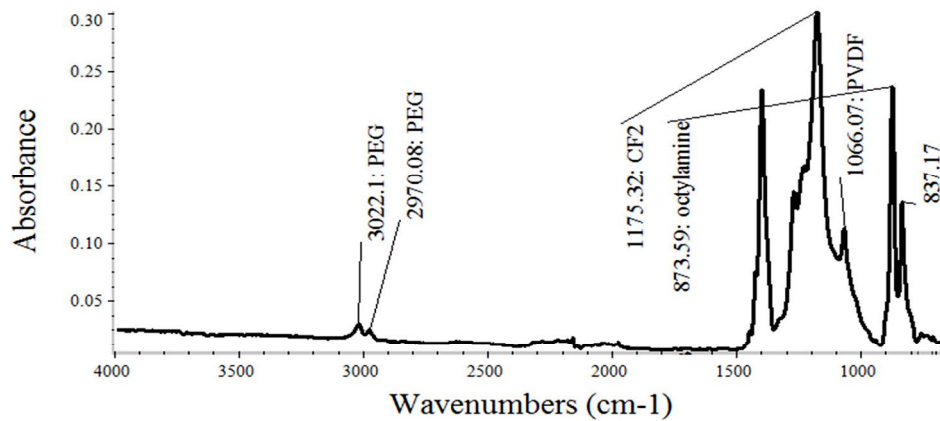
Figure 2: ATR-FTIR spectra of \text{NP}^{\text{SP}} -PVDF hybrid membrane.
