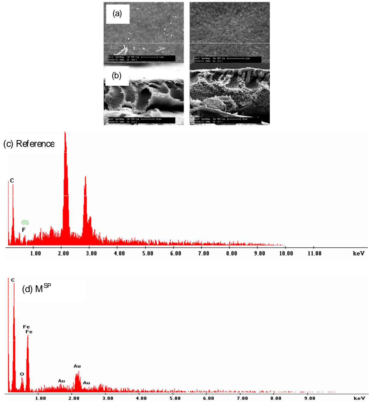
Figure 4: Surface (a) and cross-sectional (b) SEM morphology of reference (left) and M^{SP} (right) membrane, showing absence of a significant change in the membrane morphological structure due to presence of NP^{SP} layer in the polymer matrix and (c) EDX spectra of reference and (d) EDX spectra of 0.33 w/w % M^{SP} indicating inclusion of ferric particles in the polymer matrix resulted in a prominent peak related that is related to Fe.
