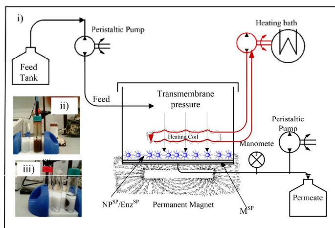
Figure 3: i) Schematic representation of a biocatalytic membrane reactor (BMR) using enzymes immobilized on superparamagnetic nanoparticles (Enz SP ) and a superparamagnetic mixed matrix membrane (M SP ) and inset Figure: ii) Solution containing Enz SP dispersion in the absence of magnetic field and iii) permeate of BMR SP and dispersion of Enz SP in the presence of magnet showing the magnetic responsiveness of the Enz SP and clear permeate solution due to the complete retention of the Enz SP by the M SP .
