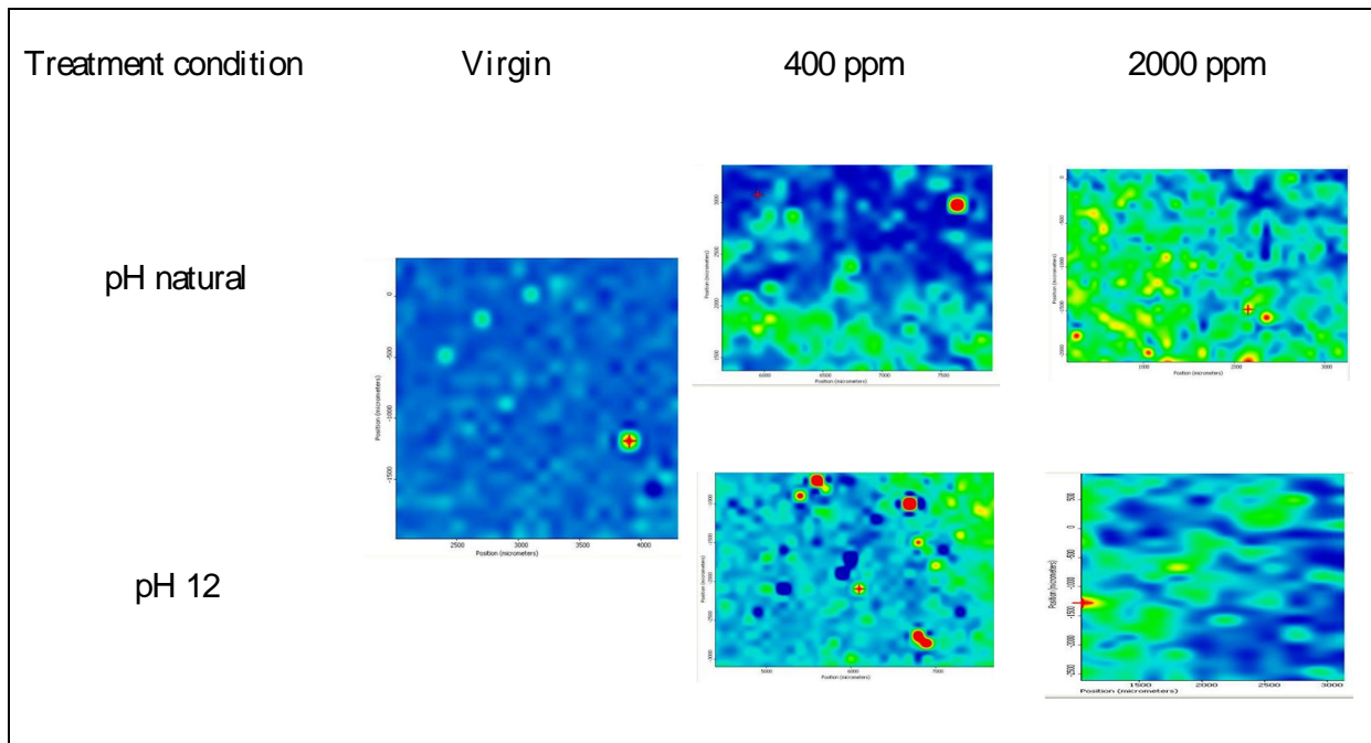
(b): H_{2850}/H_{1185}
