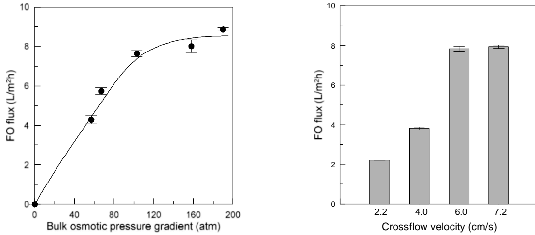
Figure 5: Effect of a) osmotic pressure gradient (feed: pure water; crossflow velocity: 6 cm/s) and b) crossflow velocity (feed: pure water; \pi_b^0 = 103 bar).
