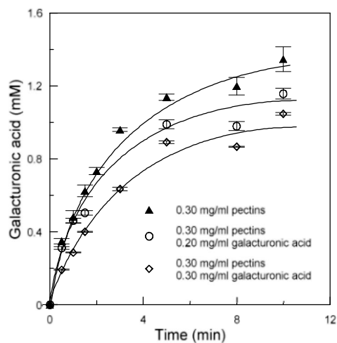
Figure 8: Inhibitory effect of galacturonic acid on the hydrolysis of pectin at 0.3 mg/mL substrate concentration and 0.0092 mg/mL enzyme concentration.
