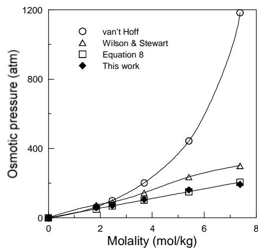
Figure 4: Osmotic pressure of the DS (MgCl 2 ) evaluated at different molal concentration.
