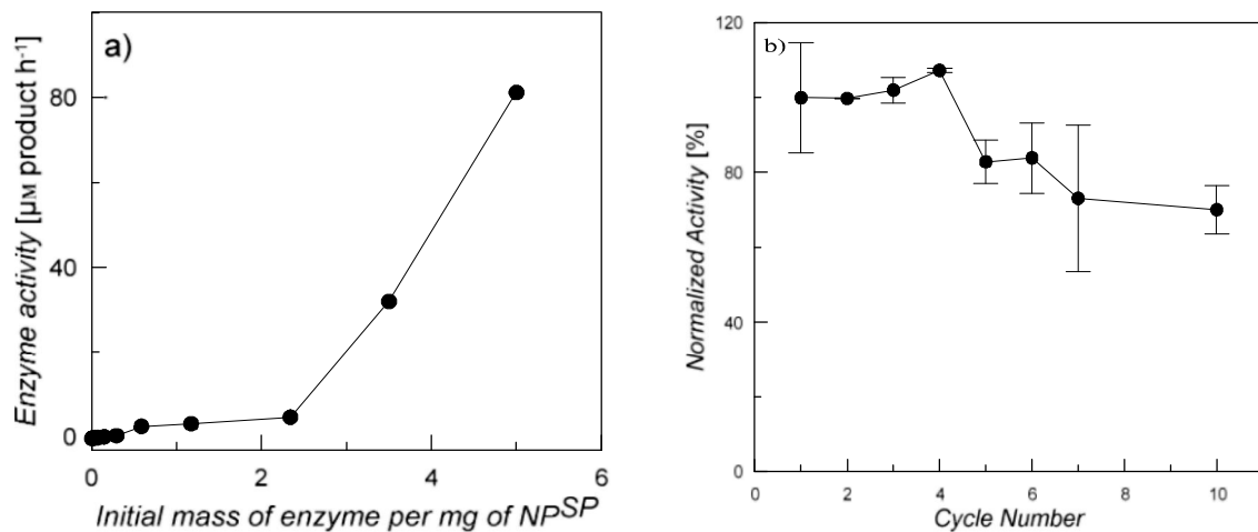
Figure 6: a) Activity at 37°C of immobilized enzyme incubated with a range of initial enzyme concentrations on 2.4 mg NP SP in a 10 mL reaction flask tested using a 5 mL and 4 mg/mL pectin solution under constant shaking at 150 rpm, b) reuse stability of the Pect SP on 2.4 mg NP SP activated with 1.2 mL a 2.34 mg/mL enzyme solution. The Pect SP was incubated with 4 mg/mL pectin solution at 37°C for one hour under constant shaking at 150 rpm for 10 consecutive cycles with intermediate magnetic isolation of the reaction product and washing to avoid residual effect to the subsequent cycle
