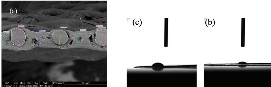
Figure 1: a) Cross-sectional SEM image of used FO membrane (Hydration Technology Inc., US; thickness \sim 50\mu\text{m} ): a polyester mesh is embedded within the polymer material as a mechanical support, b) image of water droplet on membrane and c) image of OMWW droplet on membrane.
