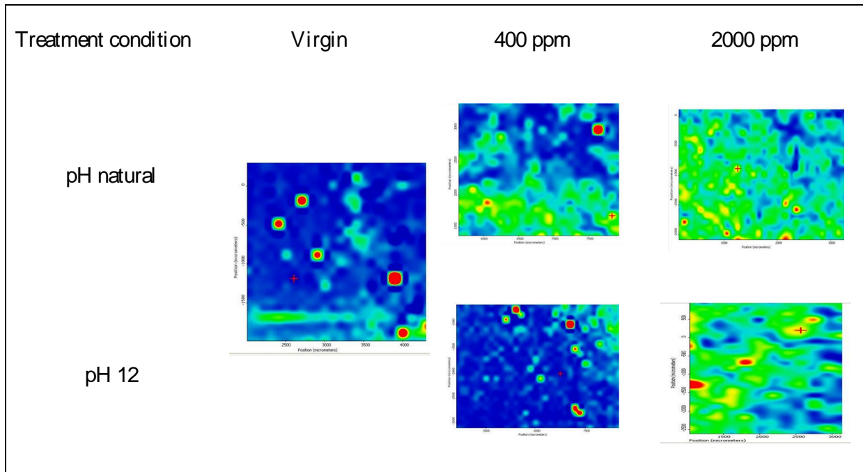
(c): H_{2920}/H_{1185}
