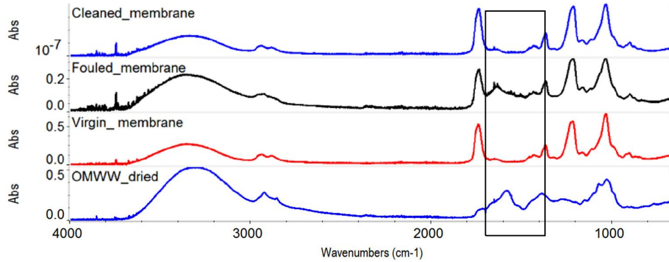
Figure 10: ATR-FTIR spectra of dried OMWW and virgin, fouled and osmotically cleaned membranes after 200 h of continuous use.
