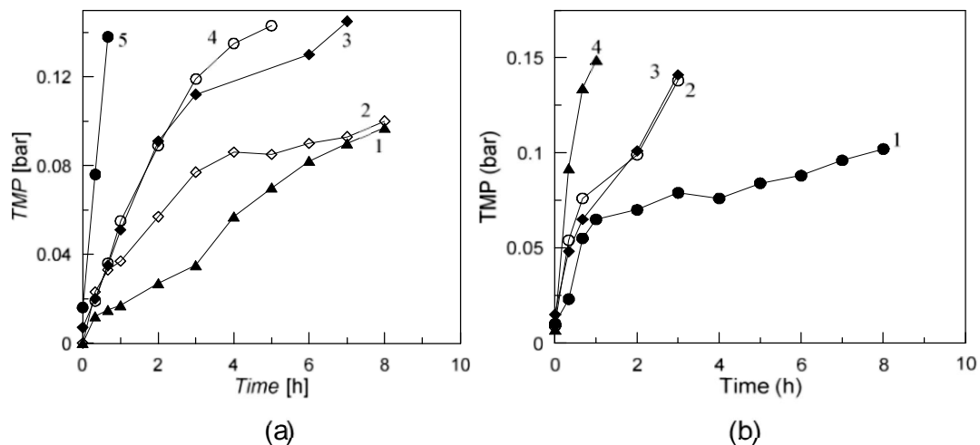
Figure 9: Operational stability of a) \text{Xyl}^{\text{SP}} (0.3 mg/mL wheat arabinoxylan feed, 17 L/m 2 .h flux at 25°C) and b) \text{Pect}^{\text{SP}} (0.3 mg/mL pectin, 17 L/m 2 .h flux at 40°C). Numbers on the Figure represent the cycle number.
