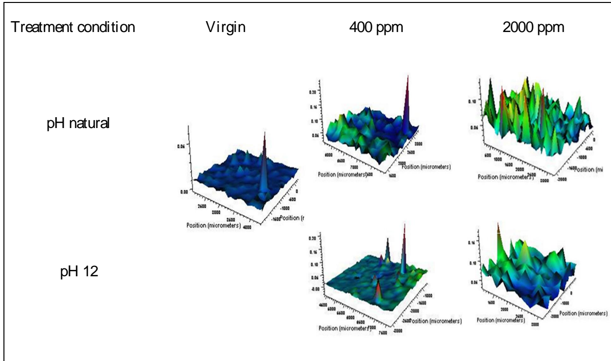
(a): H_{2850}/H_{1185}
