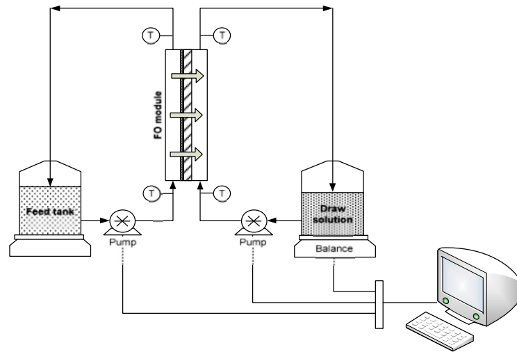
Figure 2: Flow-sheet of the lab-scale FO setup.
