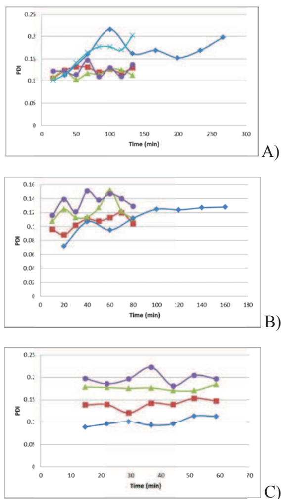
Figure S2. Variation of PDI with operating time for a bore size of 150 \mu\text{m} (A), 250 \mu\text{m} (B) and 500 \mu\text{m} (C) and for different inlet flow rates (-♦-: 0 mL/min, -X-: 0.05 mL/min, -■-: 0.25 mL/min, -▲-: 0.5 mL/min, -●-: 0.75 mL/min); reciprocating flow rate was set to 30 mL/min (A), 50 mL/min (B) and 136 mL/min (B).
