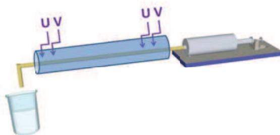
Figure 9 Schematic drawing of the UV-initiated polymerization setup to convert the polymerizable nanoemulsion into a colloidal suspension of polymer nanoparticles (not to scale).
