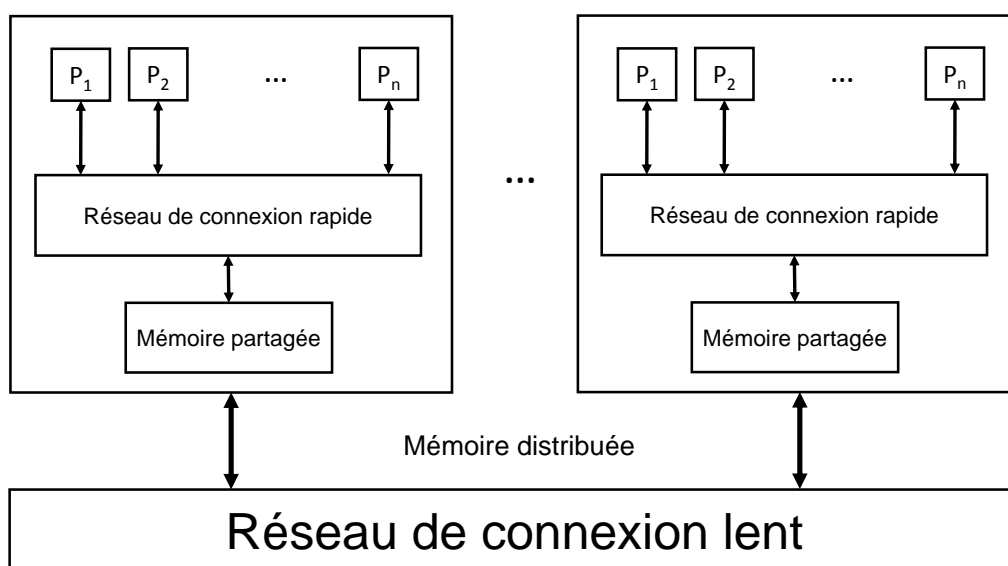
FIGURE 1.3 – Architecture hybride (Talbi, 2009)
