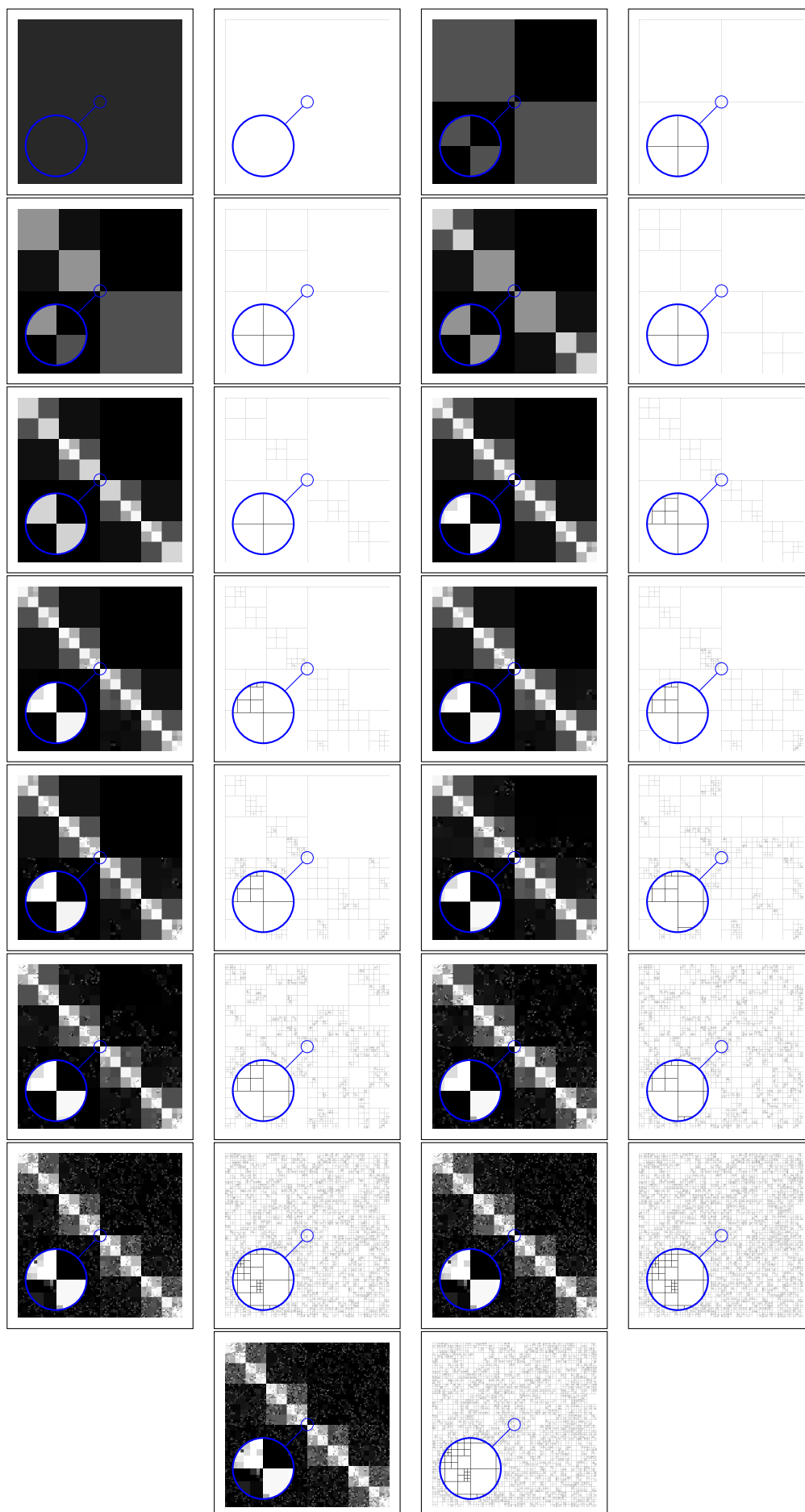
Figure 18 – Segmentation path of noisy image, at dimensions [1, 4, 7, 16, 31, 58, 121, 256, 511, 970, 2038, 4093, 8185, 9985, 9988](estimates and borders)
