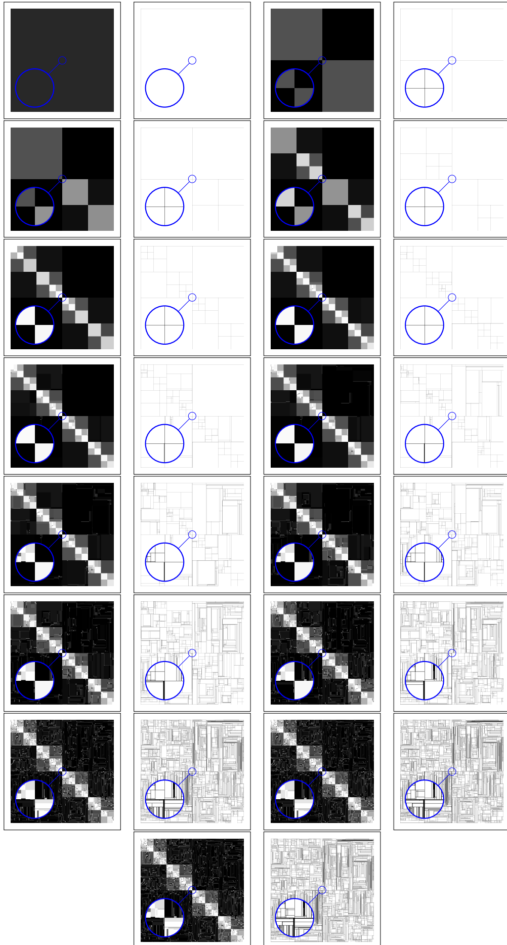
Figure 10 – Segmentation path of noisy image, at dimensions [1, 4, 7, 16, 31, 64, 127, 255, 498, 1023, 2046, 4088, 8188, 9976, 9979] (estimates and borders)
