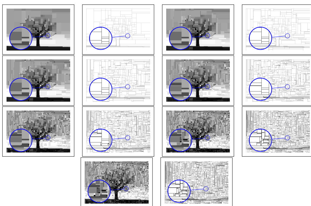
Figure 23 – Segmentation path of noisy image along noise peaks starting from near oracle, at dimensions [301, 514, 1027, 2048, 4098, 8194, 10000](estimates and borders)
