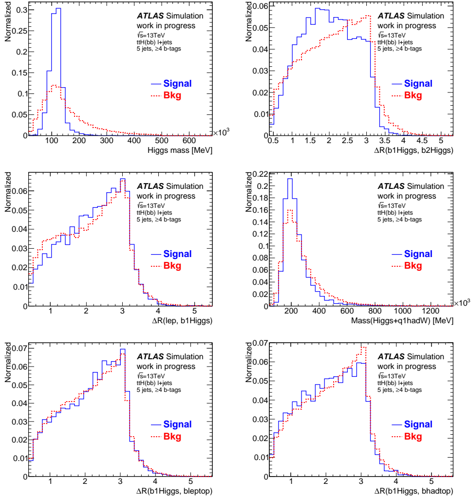
Figure 4.11.: Distributions of Higgs related variables used as inputs for the recoBDT_withHiggs in the 5 jets, \geq 4 b-tags region. Solid blue lines correspond to the correct combination (signal) while the dashed red lines show the combinatorial background.
