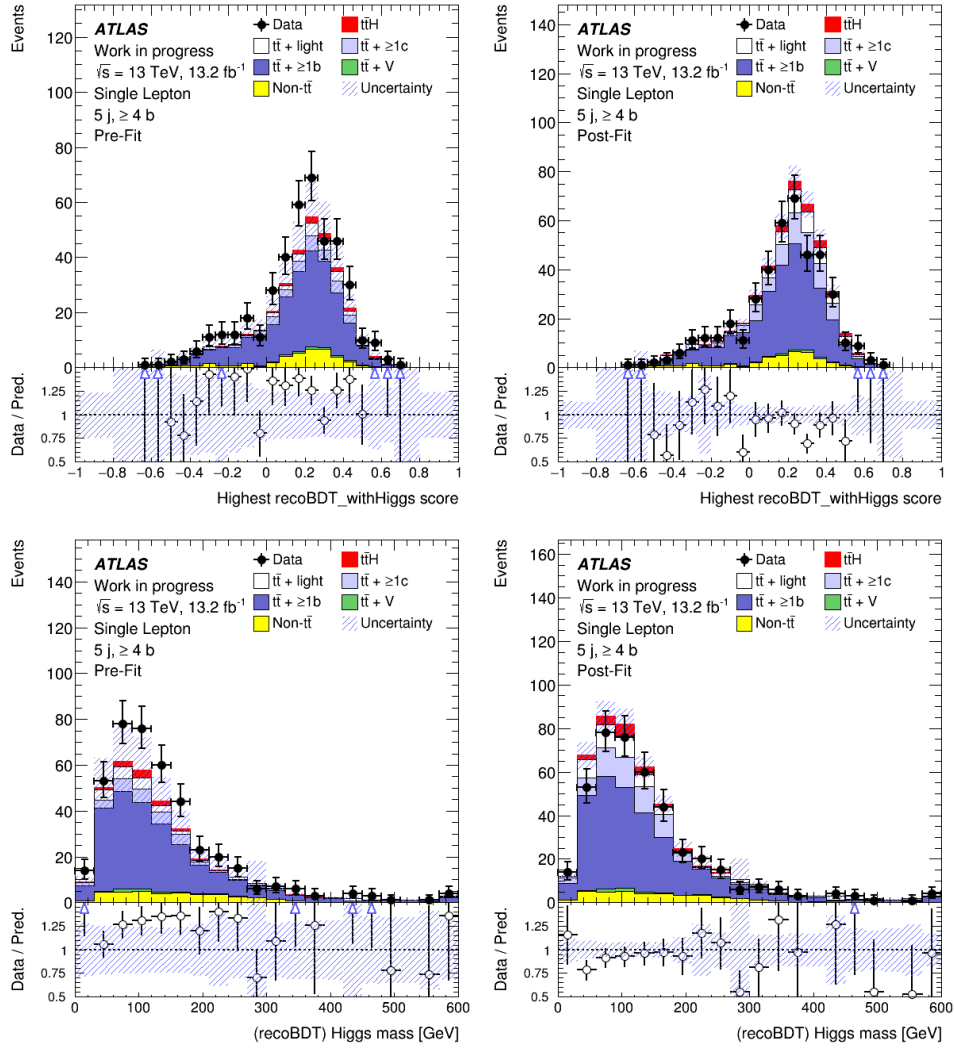
Figure B.5.: Distributions of the discriminating variables before and after the fitting procedure in the 5 jets, \geq 4 b -tags region. The uncertainty band contains the statistical and systematic contribution. The pre-fit distributions do not include an uncertainty on the normalisation of t\bar{t} + \geq 1b or t\bar{t} + \geq 1c .
