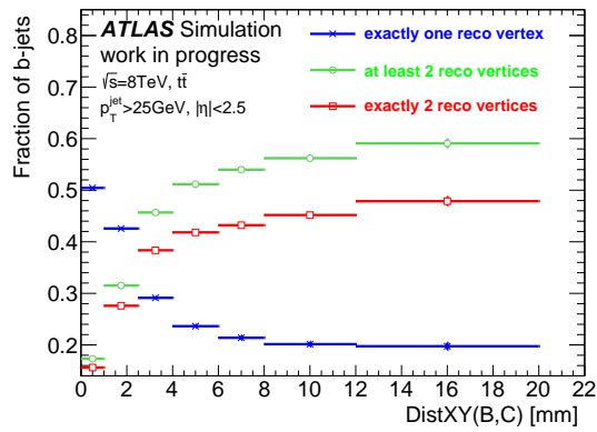
Figure 3.18.: Fraction of single- b jets with two reconstructable B and C vertices as a function of the transverse distance between B and C vertices. Three categories are shown: jets with exactly one reconstructed vertex, jets with at least 2 reconstructed vertices and jets with exactly 2 reconstructed vertices.
