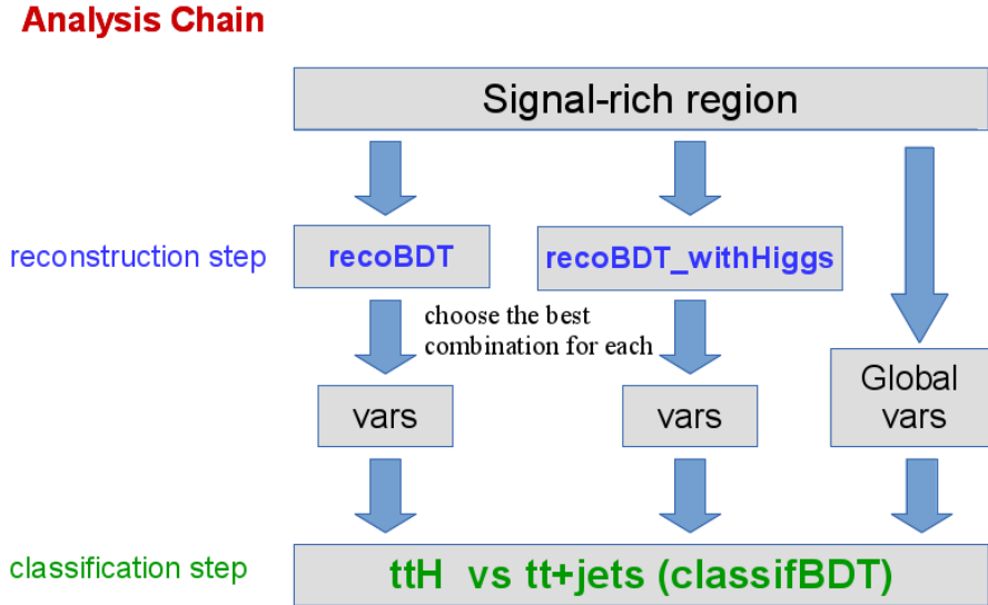
Figure 4.17.: For each signal-rich region, information from the reconstruction BDTs is combined with global kinematic variables in a classification BDT that is used to separate t\bar{t}H from the dominant t\bar{t}+\text{jets} background.
