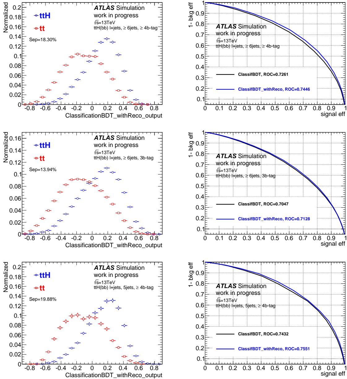
Figure 4.22.: On the left, distributions of the classification BDT with reconstruction output for the ttH signal and the tt + jets background in the signal regions. On the right, the ROC curves for the classification BDTs with and without reconstruction variables.
