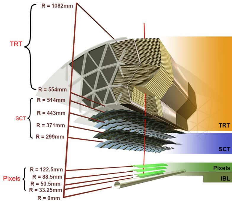
Figure 2.5.: The ATLAS Inner Detector for Run 2.
