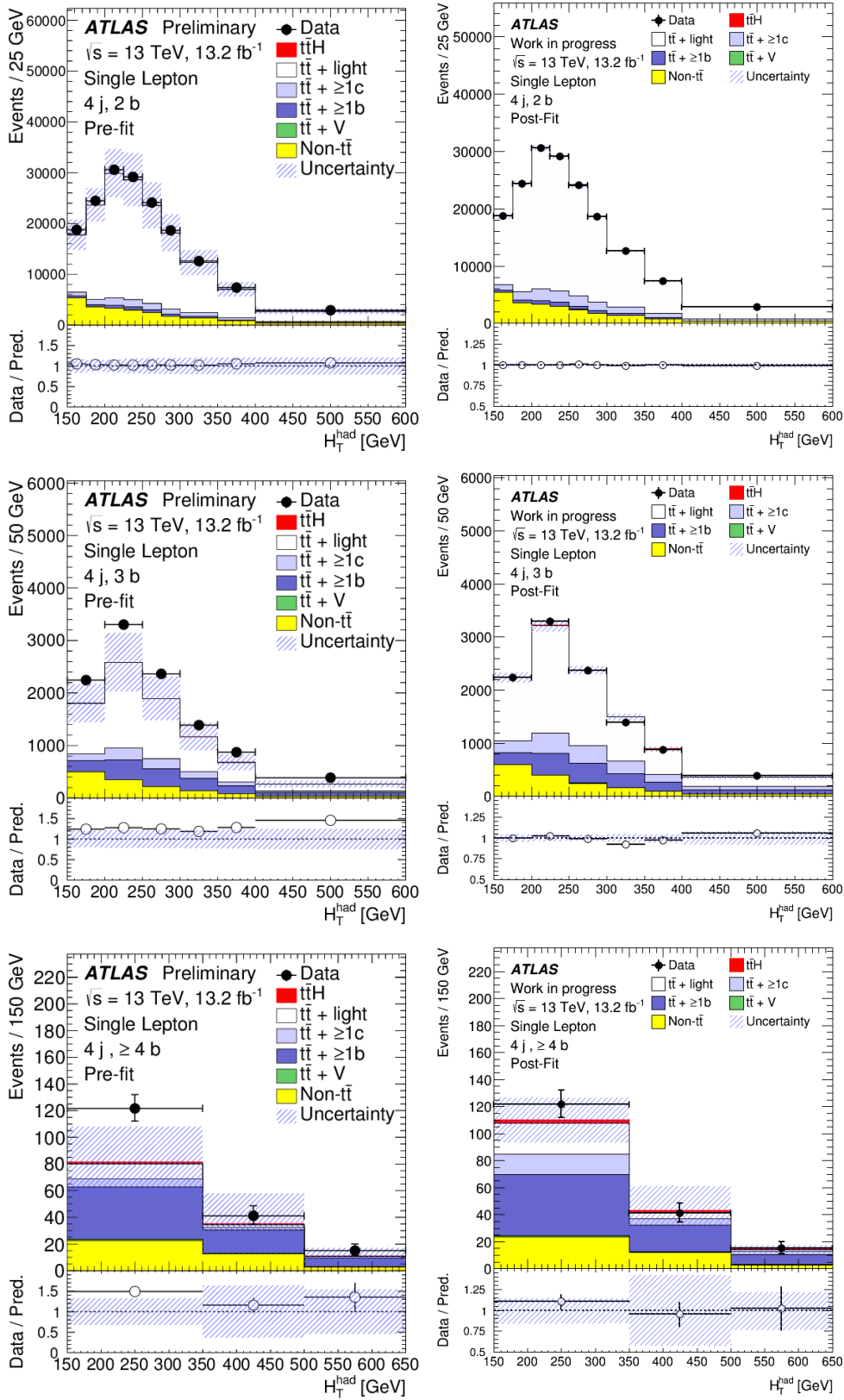
Figure 4.27.: Pre-fit [117] and post-fit plots for the H_T^{\text{had}} variable in the four exclusive jet region. The pre-fit distributions do not include an uncertainty on the normalisation of t\bar{t} + \geq 1b or t\bar{t} + \geq 1c .
