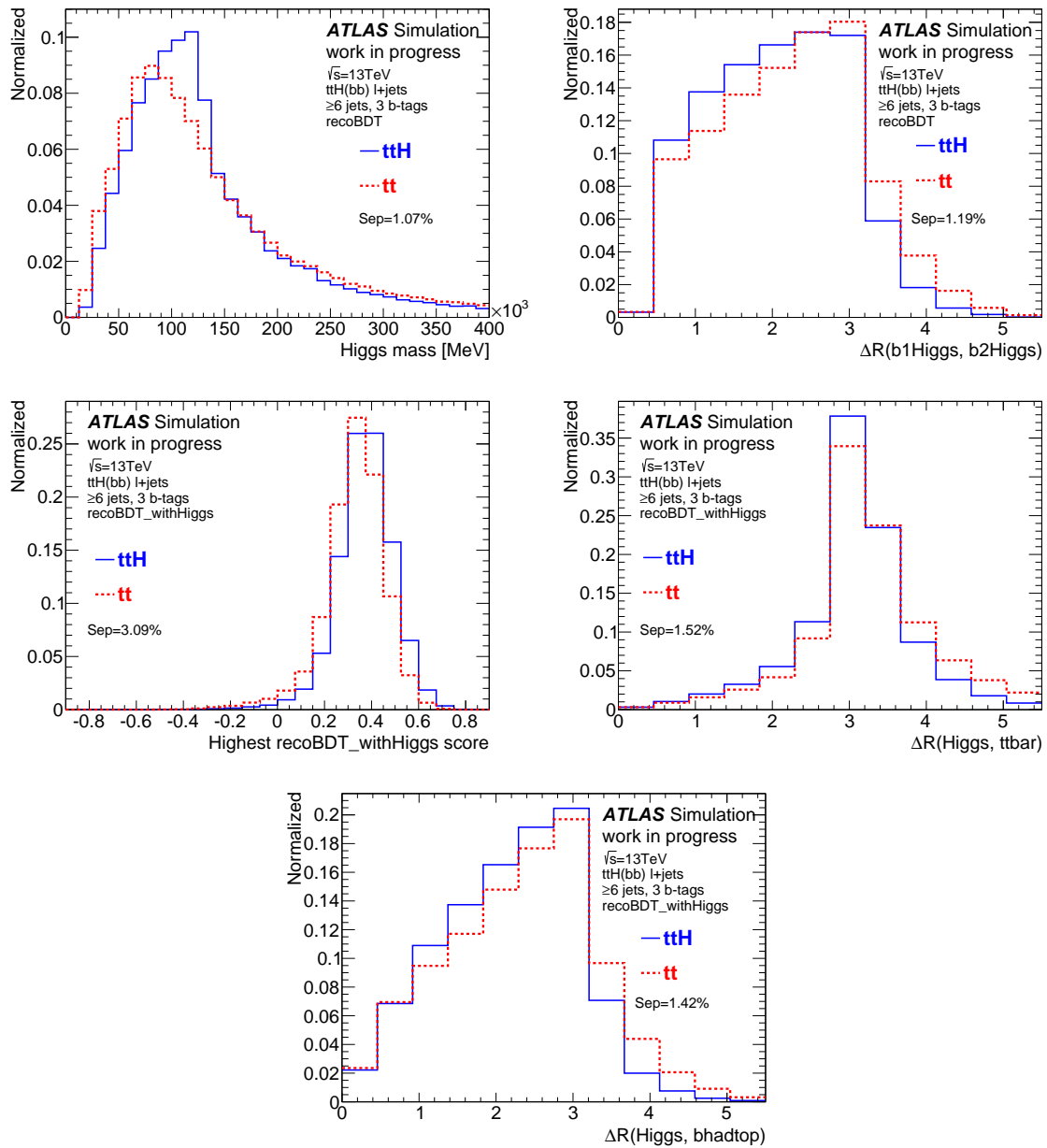
Figure 4.19.: Discriminating variables using reconstructed objects from recoBDT and recoBDT_withHiggs in the region with \geq 6 jets, 3 b-tags. Each plot shows the normalised distribution for t\bar{t}H signal (solid blue) and the t\bar{t} +jets background (dashed red). The TMVA separation (Sep), as defined in equation 4.4, is also shown.
