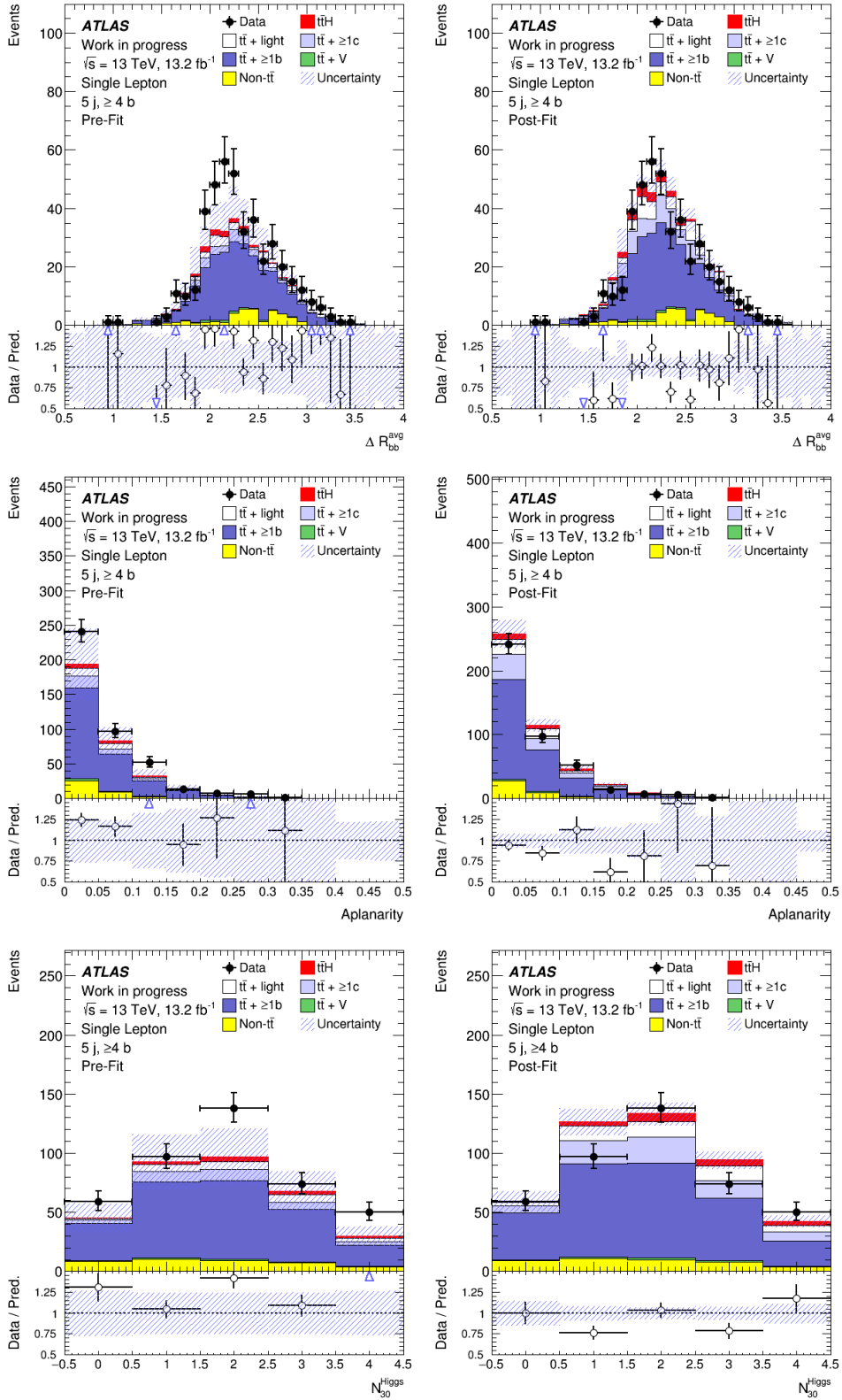
Figure B.3.: Distributions of the discriminating variables before and after the fitting procedure in the 5 jets, \geq 4 b -tags region. The uncertainty band contains the statistical and systematic contribution. The pre-fit distributions do not include an uncertainty on the normalisation of t\bar{t} + \geq 1b or t\bar{t} + \geq 1c .
