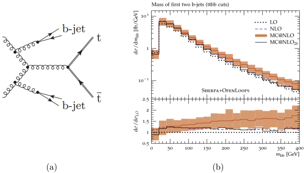
Figure 3.2.: (a) t\bar{t}b\bar{b} production via double collinear g \rightarrow bb splitting. (b) Invariant mass of the first two b -jets. The MC@NLO bands display the matching corrections. The MC@NLO 2b curve is obtained by switching off g \rightarrow bb splittings in the parton shower. The MC@NLO/NLO ratio grows with m_{bb} and reaches 25–30% in the Higgs-signal region [64].
