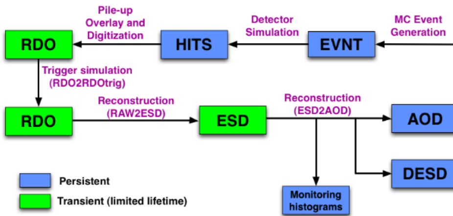
Figure 2.16.: ATLAS Monte Carlo simulation flow [35].
