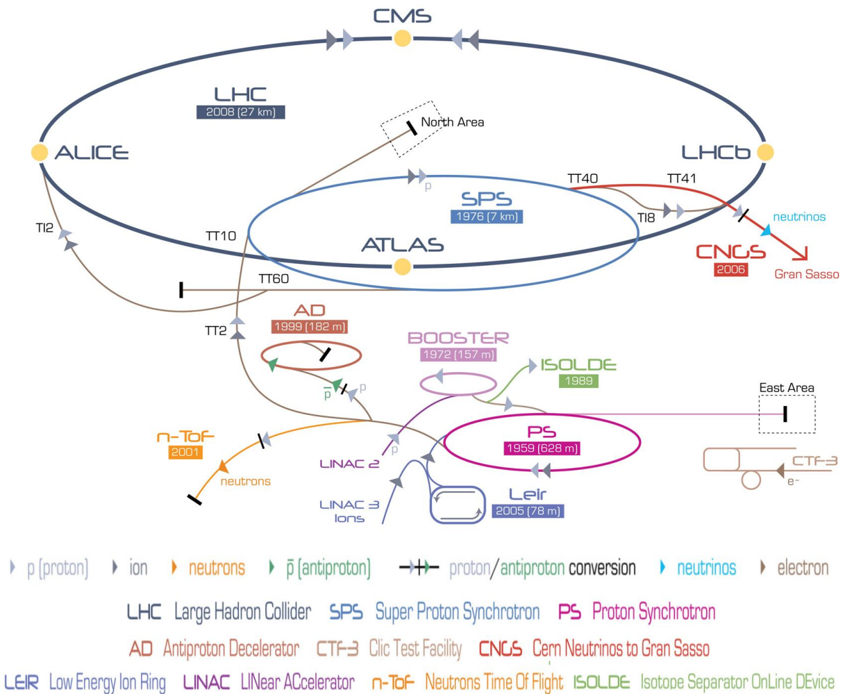
Figure 2.1.: CERN accelerator complex (not to scale), showing the injection system and the component's date of construction.
