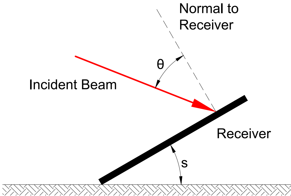
Figure 2-3: Sketch illustrating the angle of incidence on a surface
