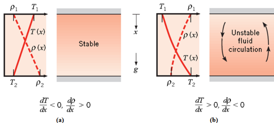
Figure C-6: Conditions in a fluid between large horizontal plates at different temperatures: (a) Stable temperature gradient, (b) Unstable temperature gradient. Source: [175]
