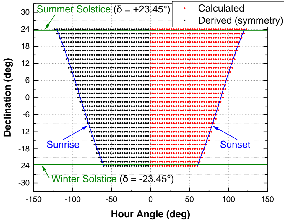
Figure 5-20: \delta - \omega space, showing the \delta - \omega pairs for which flux maps are calculated ( \omega \geq 0 ), and derived ( \omega < 0 ). Morning flux maps are derived from afternoon ones due to symmetry.
