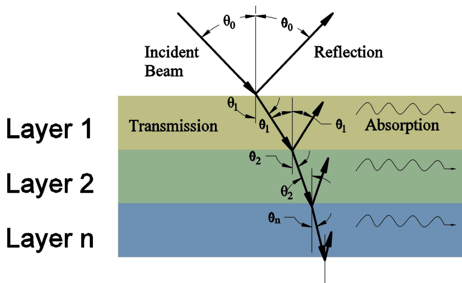
Figure 5-5: Snell's law: light is refracted as it passes into a medium with a different refraction index.
