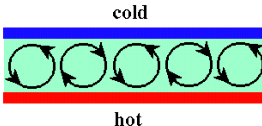
Figure C-7: Schematic of Rayleigh-Bénard convection. Source: [176]
