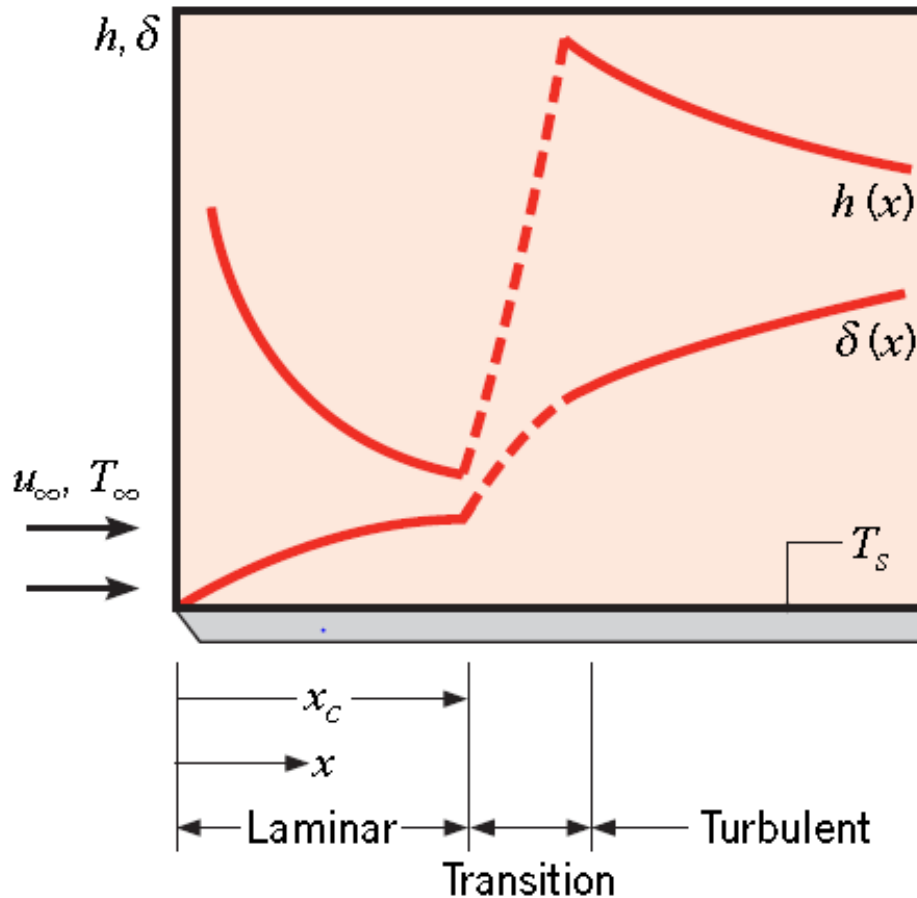
Figure C-5: Variation of velocity boundary layer thickness \delta and the local heat transfer coefficient h for flow over an isothermal flat plate. Source: [175]
