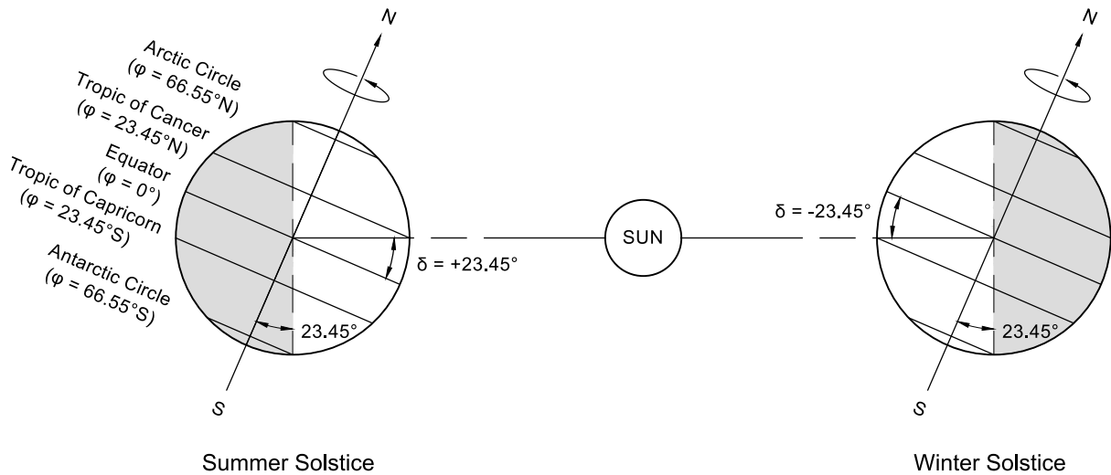
Figure 2-1: Sketch illustrating the solar declination. The Sun and Earth sizes and distances are not to scale.
