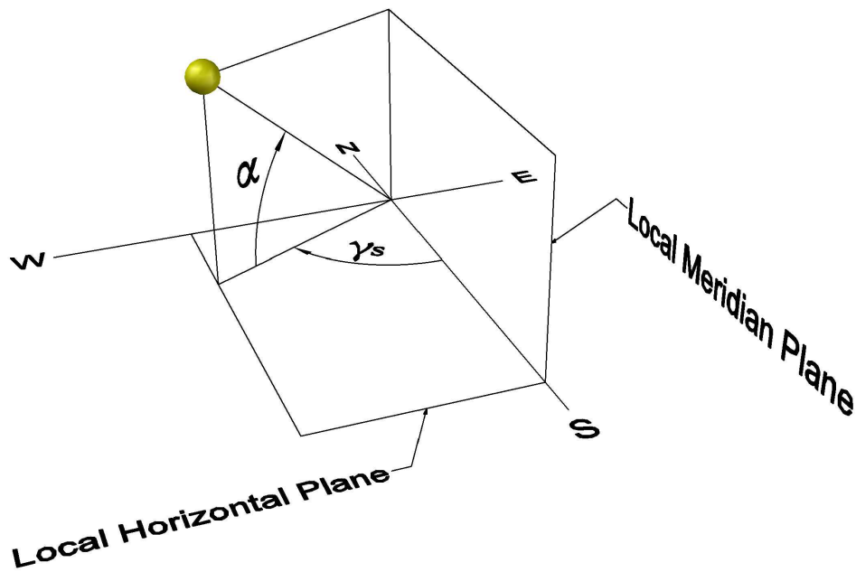
Figure 2-4: Sketch illustrating the solar altitude angle, \alpha , and the solar azimuth angle, \gamma_S . The convention used for the solar azimuth angle is 0 for South, and increasing towards West.
