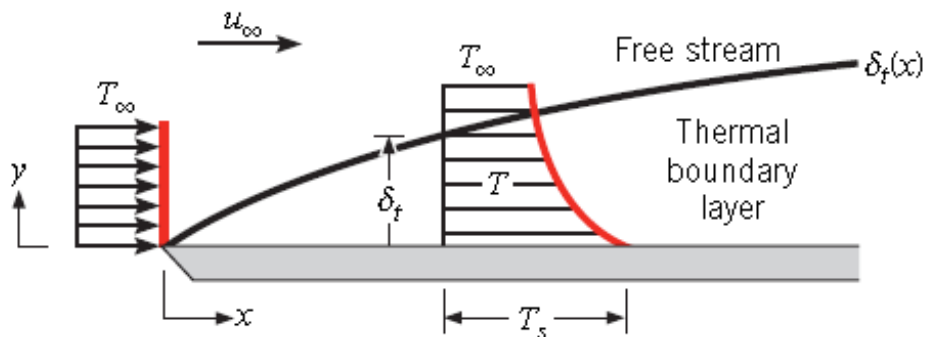
Figure C-3: Thermal boundary layer. Source: [175]
