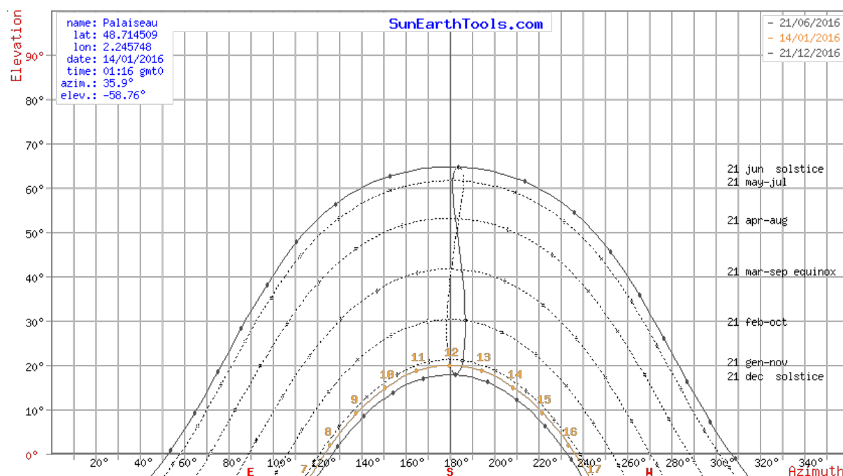
Figure 5-19: Sun path diagram for Palaiseau. Downloaded from www.sunearthtools.com
