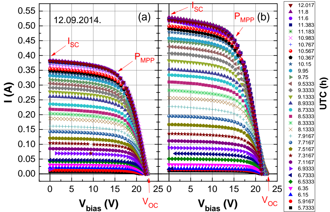
Figure 3-4: A morning of I - V curves measured on a sunny day for (a) a frontal a -Si:H module (module 6), and (b) a reflector-equipped a -Si:H module (module 15).
