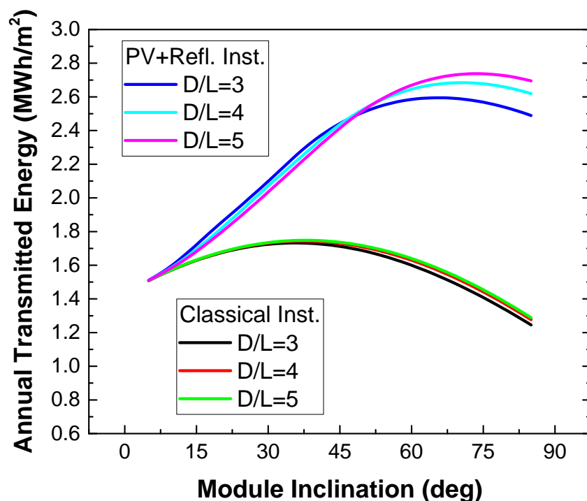
Figure 5-13: Results of geometrical optimisations of infinitely-long PV+Reflector and Classical installations for D/L values of 3, 4, and 5, for maximising the annual transmitted energy under clear-sky conditions.
