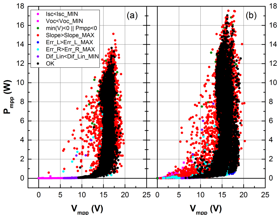
Figure 3-8: Visualisation of the filters as applied to almost two years of measurements (31.03.2014 - 07.03.2016), for (a) module 5 (a frontal p -Si module), and (b) module 16 (a reflector-equipped p -Si module).
