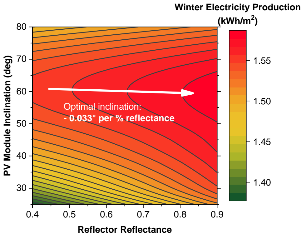
Figure 9-4: Winter energy production of a -Si:H modules equipped with planar reflectors, as a function of PV module inclination and mirror reflectance. Spacing between contour lines: 0.01 kWh/m 2 .
