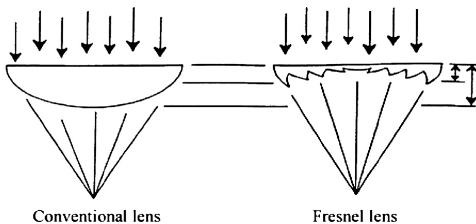
Figure 1-7: Conventional lens and Fresnel lens. The advantage of Fresnel lens is a lower material consumption. Source: Sierra and Vazquez, 2005 [14]
