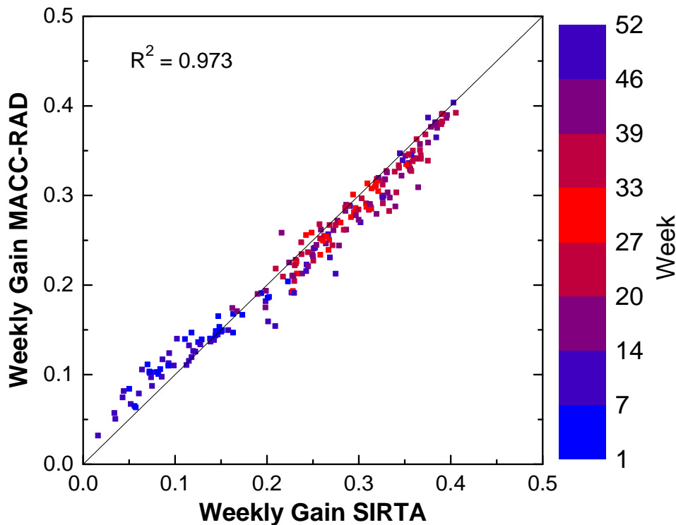
Figure 9-1: Validation of MACC-RAD surface irradiance data. A simulation was run for each year using two sets of data (MACC-RAD and locally measured) to calculate the weekly gain in energy transmitted to the cells. The geometry of both control and reflector-equipped modules were set to match the experiment (module inclination of 49^\circ and D/L of 3.00).
