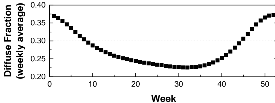
Figure 5-15: The annual distribution of weekly average diffuse fraction under clear sky (using McClear data for Palaiseau). A higher concentration of aerosols in the spring period results in a slightly higher diffuse fraction in spring compared to the fall.
