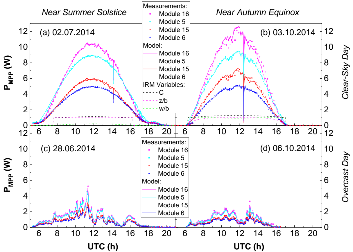
Figure 5-12: Analytical optical model validation (indirectly through P_{MPP} measurements and predictions) on a clear-sky and an overcast day near the summer solstice (a, c), and near the autumnal equinox (b, d). Modules 6 and 15 are row 1 and row 3 a -Si:H modules, while modules 5 and 16 are row 1 and row 3 p -Si modules. Variables C , z/b , and w/b are respectively the average concentration factor, the fraction of module being highlighted, and the fraction of useful reflector. The underperformance of PV modules from 6 to 7h in (b) is due to shading by a bungalow on site, situated south-east from the experiment.
