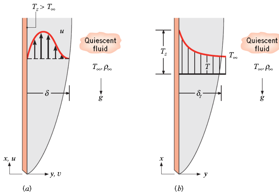
Figure C-8: Boundary layer development on a heated vertical plate: (a) Velocity boundary layer. (b) Thermal boundary layer. Source: [175]
