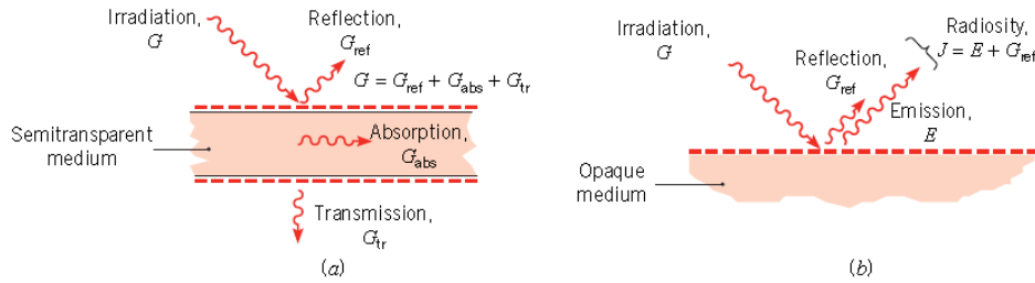
Figure C-10: Radiation at a surface. (a) Reflection, absorption, and transmission of irradiation for a semi-transparent medium. (b) The radiosity for an opaque medium. Source: [175]
