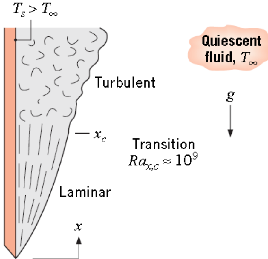
Figure C-9: Free convection boundary layer transition on a vertical plate. Source: [175]
