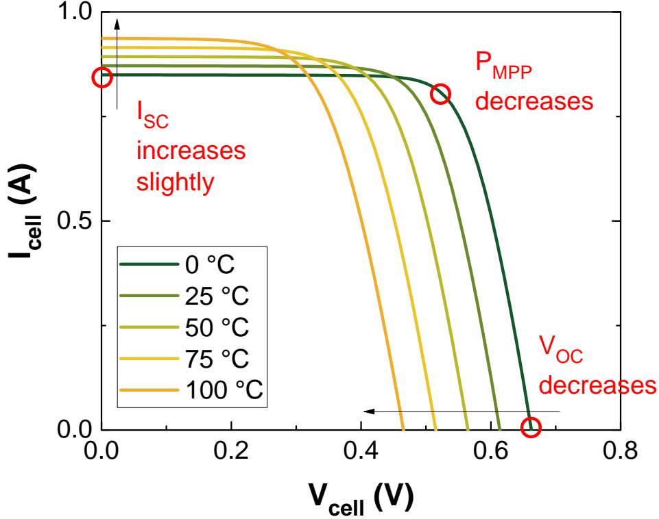
Figure 2-5: Typical p -Si cell I - V characteristic submitted to an irradiance of 1000 \text{ W/m}^2 and various operating temperatures. The increased temperature decreases the open-circuit voltage, V_{OC} , while slightly increasing the short-circuit current, I_{SC} . The overall impact is a decrease in the maximum power output, P_{MPP} .
