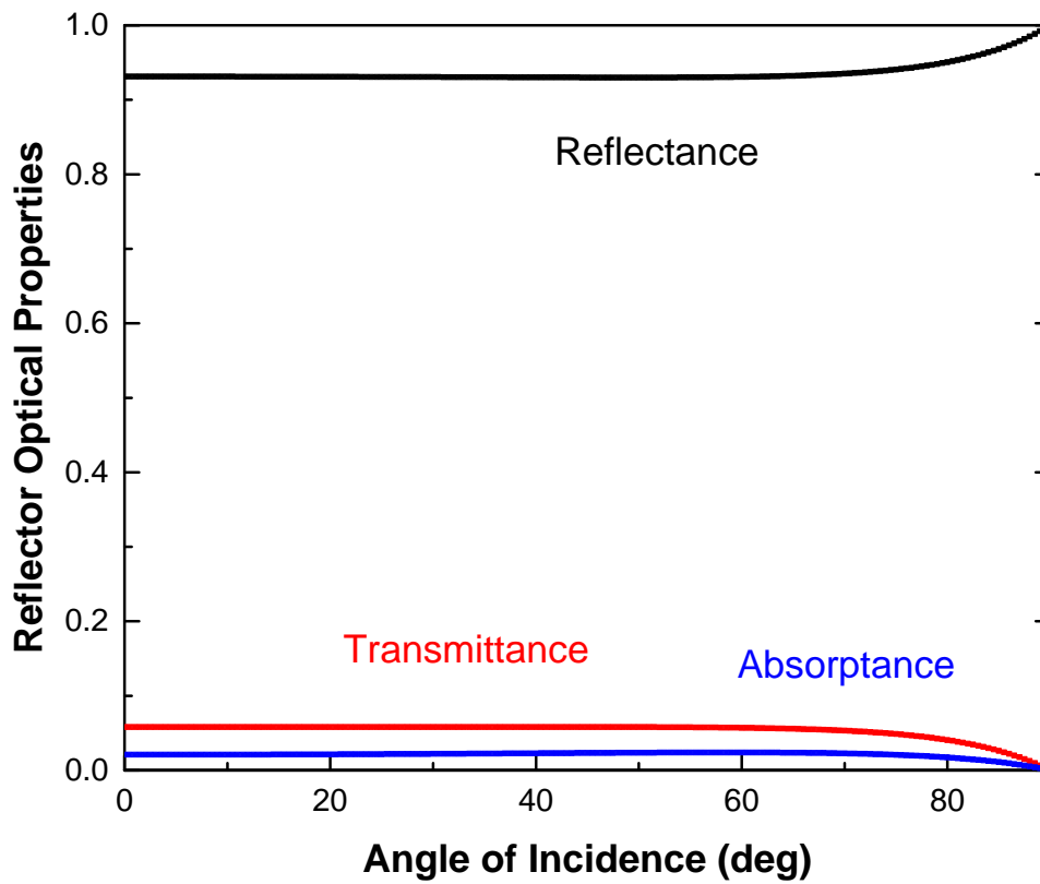
Figure 5-7: Modelled optical performance of the reflector.
