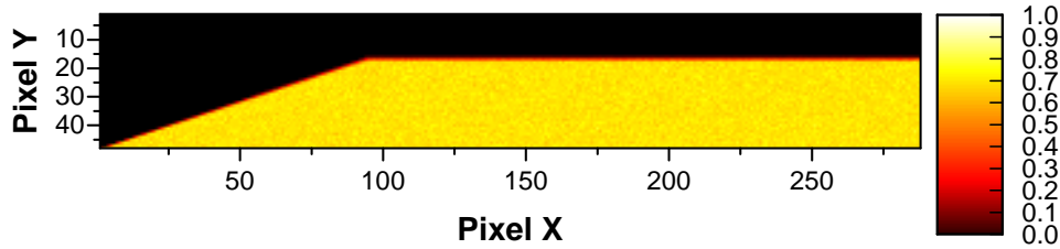
(c) Map B: Reflector contribution to the direct light on the reflector-equipped receiver
