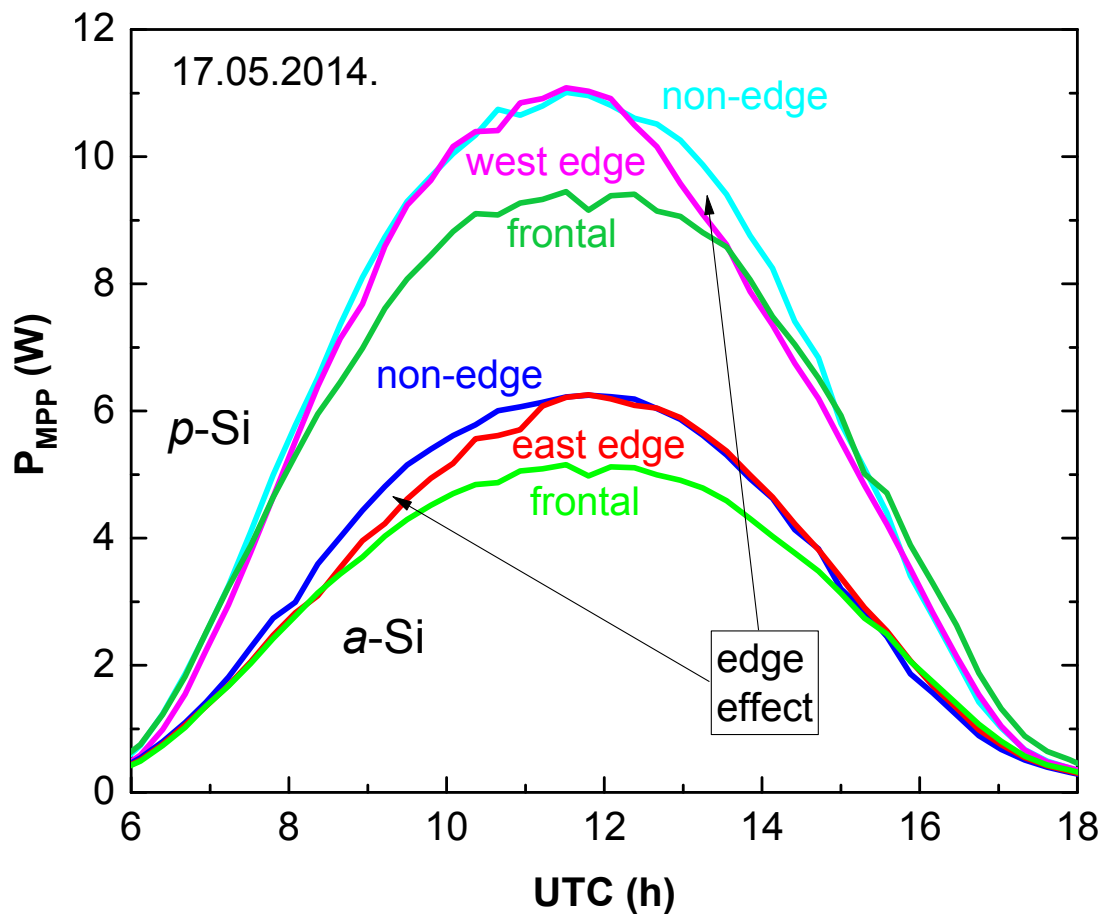
Figure 3-12: Experimental data taken on May 17th, 2014, showing an increased power production of non-edge and edge reflector-equipped modules compared to frontal modules. The edge effect is a result of the finite length of the reflector in the East-West direction, and is the most pronounced on modules closest to the row edges.
