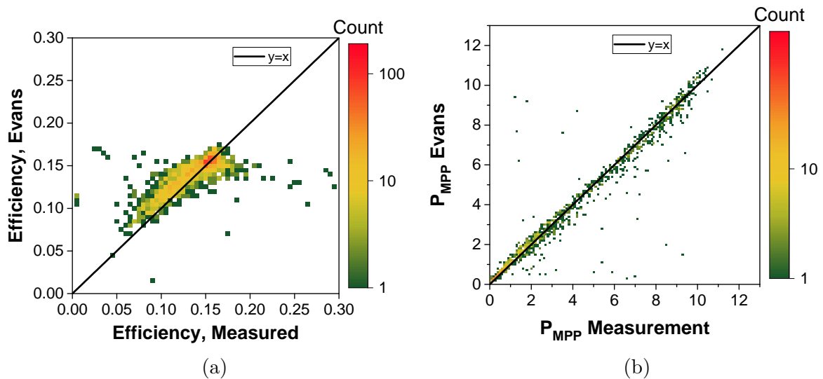
Figure 6-4: Evans model performance in predicting (a) module conversion efficiency, and (b) the P_{MPP} for module 5 (frontal p -Si) and the period 17th May - 6th October, 2014. The analytical optical model was used for calculating irradiances.
