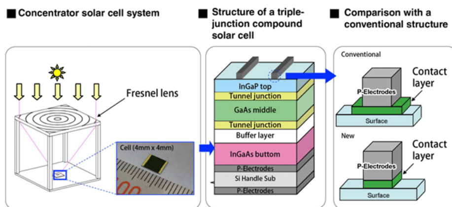
Figure 1-8: Sharp Concentrator solar cell system, operating at 44.4% efficiency. Source: Sharp, 2013 [15]
