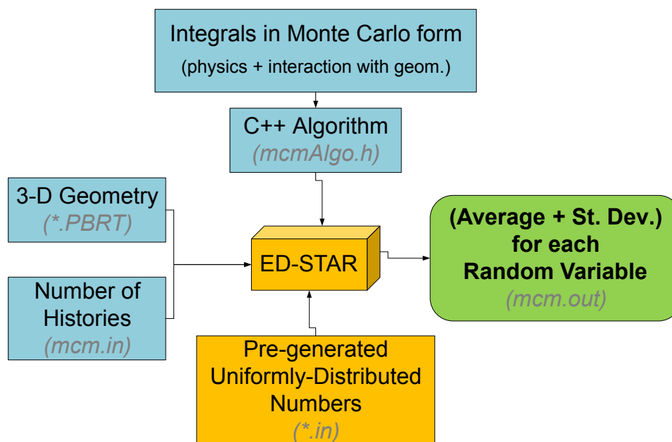
Figure 5-18: Major inputs and outputs of EDStaR. The items in orange were developed by StarWEST, the items in blue are inputs prepared by the user for each Monte Carlo simulation, and the items in green are the outputs.
