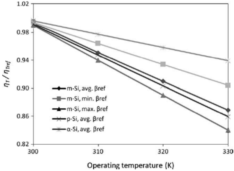
Figure 1-12: The ratio of temperature-adjusted to reference efficiency, as predicted by the Evans-Florschuetz efficiency correlation for typical silicon-based PV modules. Source: Skoplaki, 2009 [64]
