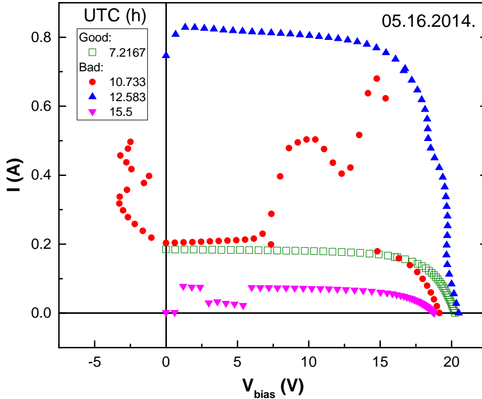
Figure 3-6: Examples of good and bad I - V measurements (module 5). Bad I - V curves are to be eliminated through quality control.
