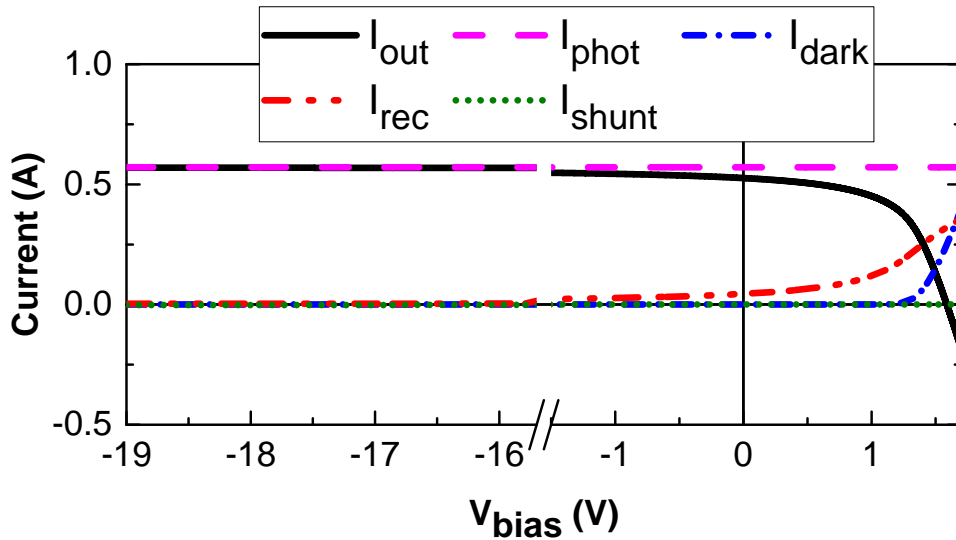
Figure 6-13: The I - V characteristics of each component of the double diode model circuit under STC conditions ( T=25\text{ }^\circ\text{C} , G_{POA}=1000\text{ W/m}^2 ). The following parameters were used: I_0=5.4 \times 10^{-17}\text{ A} , I_{SC,STC}=0.571\text{ A} , R_{sh}=9.7 \times 10^3\ \Omega , R_s=5.0 \times 10^{-1}\ \Omega , and n=1.700 .
