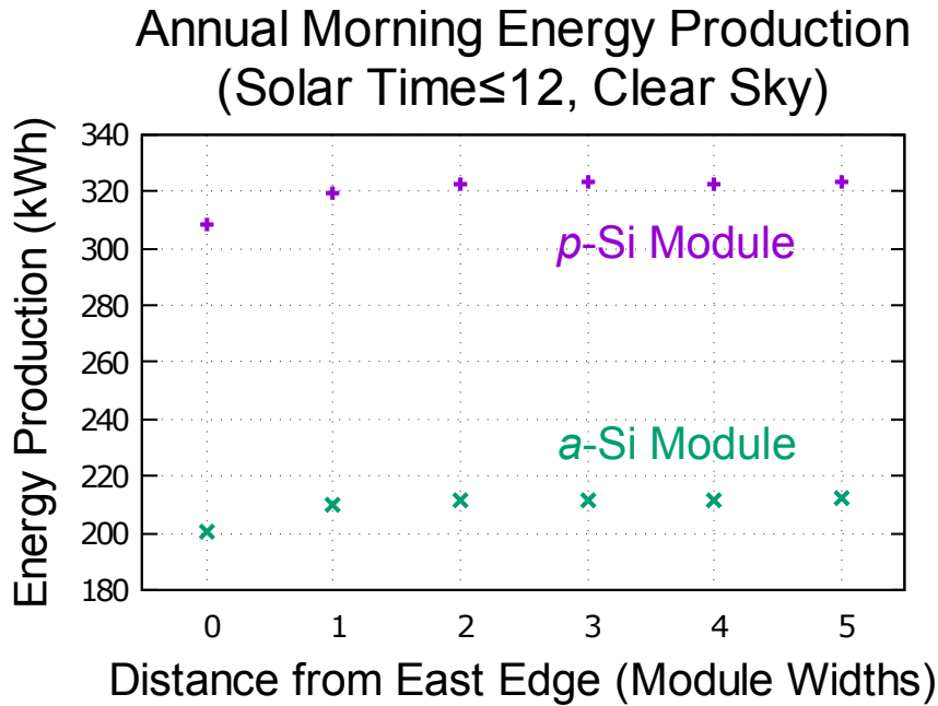
Figure 9-6: Annual morning energy production of a -Si:H and p -Si modules as a function of distance from the east row edge, evaluated under clear sky conditions [95]. The equivalent energy productions for frontal a -Si:H and p -Si modules are 183 kWh and 282 kWh, respectively.
