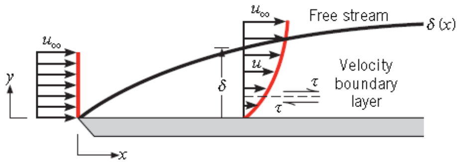
Figure C-2: Velocity boundary layer. Source: [175]
