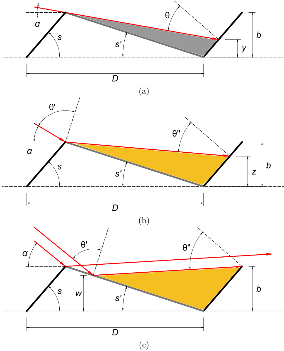
Figure 5-10: Three principal cases of the system behaviour: a) partial or total shading of the PV module, b) heterogeneous concentration and c) homogeneous concentration with a varying degree of utility of the reflector. The PV modules are denoted with thick black lines, the reflectors are denoted with thick gray lines, and the beam irradiance is denoted in red. The schematic is in the meridian plane.
