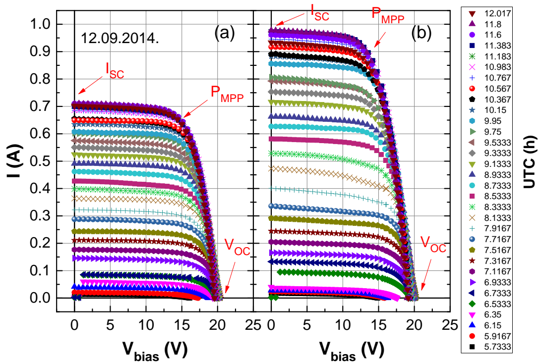
Figure 3-5: A morning of I - V curves measured on a sunny day for (a) a frontal p -Si module (module 5), and (b) a reflector-equipped p -Si module (module 16).
