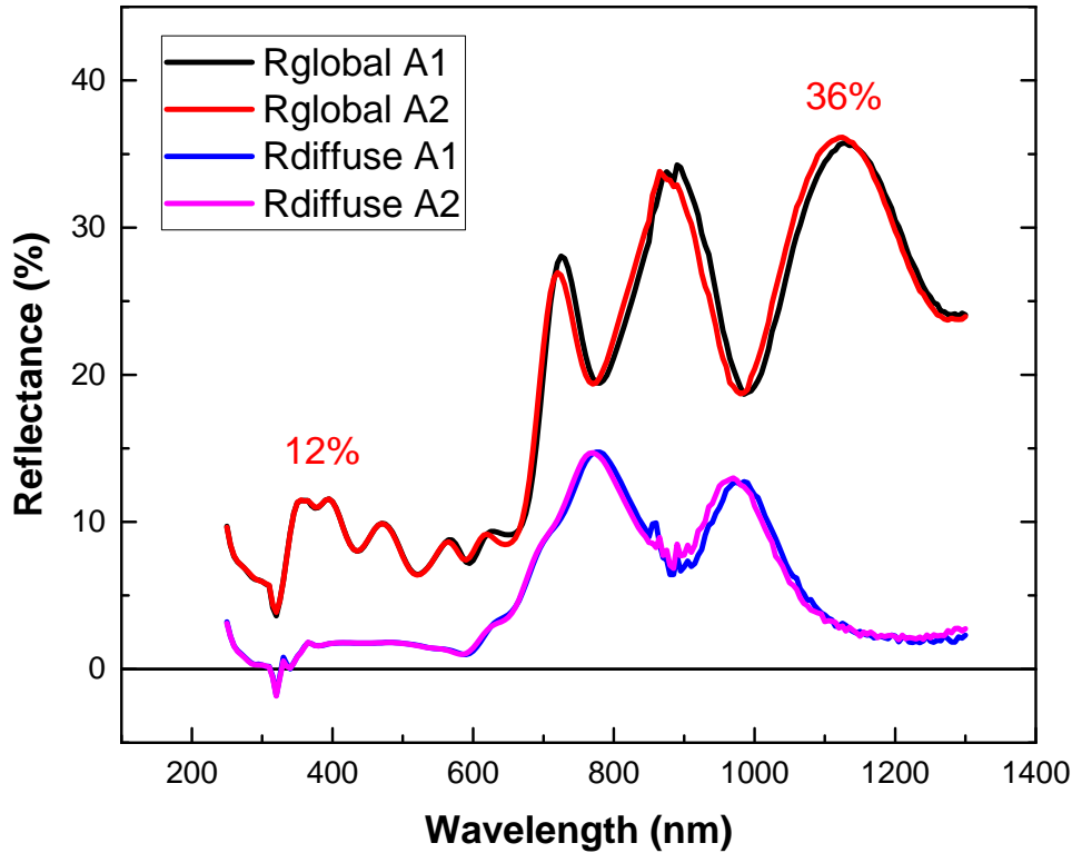
Figure 5-1: Laboratory measurements of total and diffuse reflectance as a function of wavelength for two a -Si:H samples.
