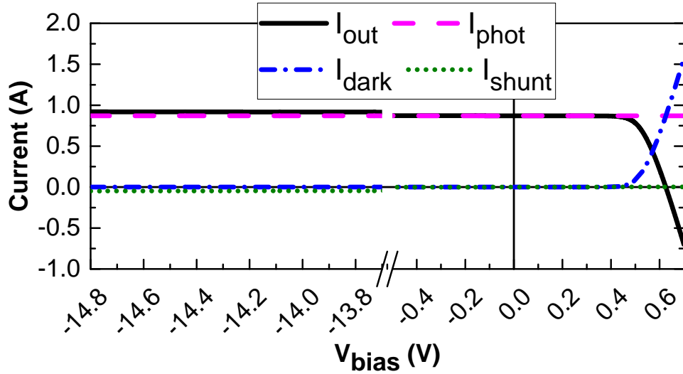
Figure 6-9: The I - V characteristics of each component of the single diode cell model circuit under STC conditions ( T=25\text{ }^\circ\text{C} , G_{POA}=1000\text{ W/m}^2 ). The following parameters were used: I_0=9.8 \times 10^{-11}\text{ A} , I_{SC,STC}=0.871\text{ A} , R_{sh}=3.0 \times 10^2\ \Omega , R_s=4.2 \times 10^{-2}\ \Omega , n=1.000 . The axis break is shown to demonstrate the evolution of the shunt current with voltage bias.
