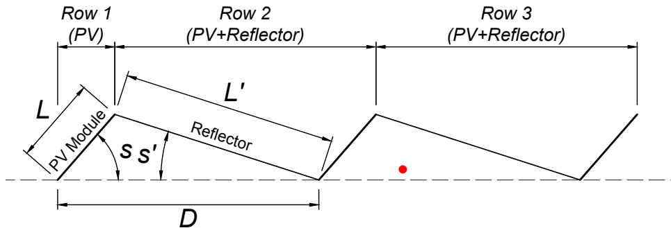
Figure 3-2: Schematic of the experiment showing the geometry of the system. The red dot represents the position of the temperature probe within the back cavity (5 cm off the ground).
