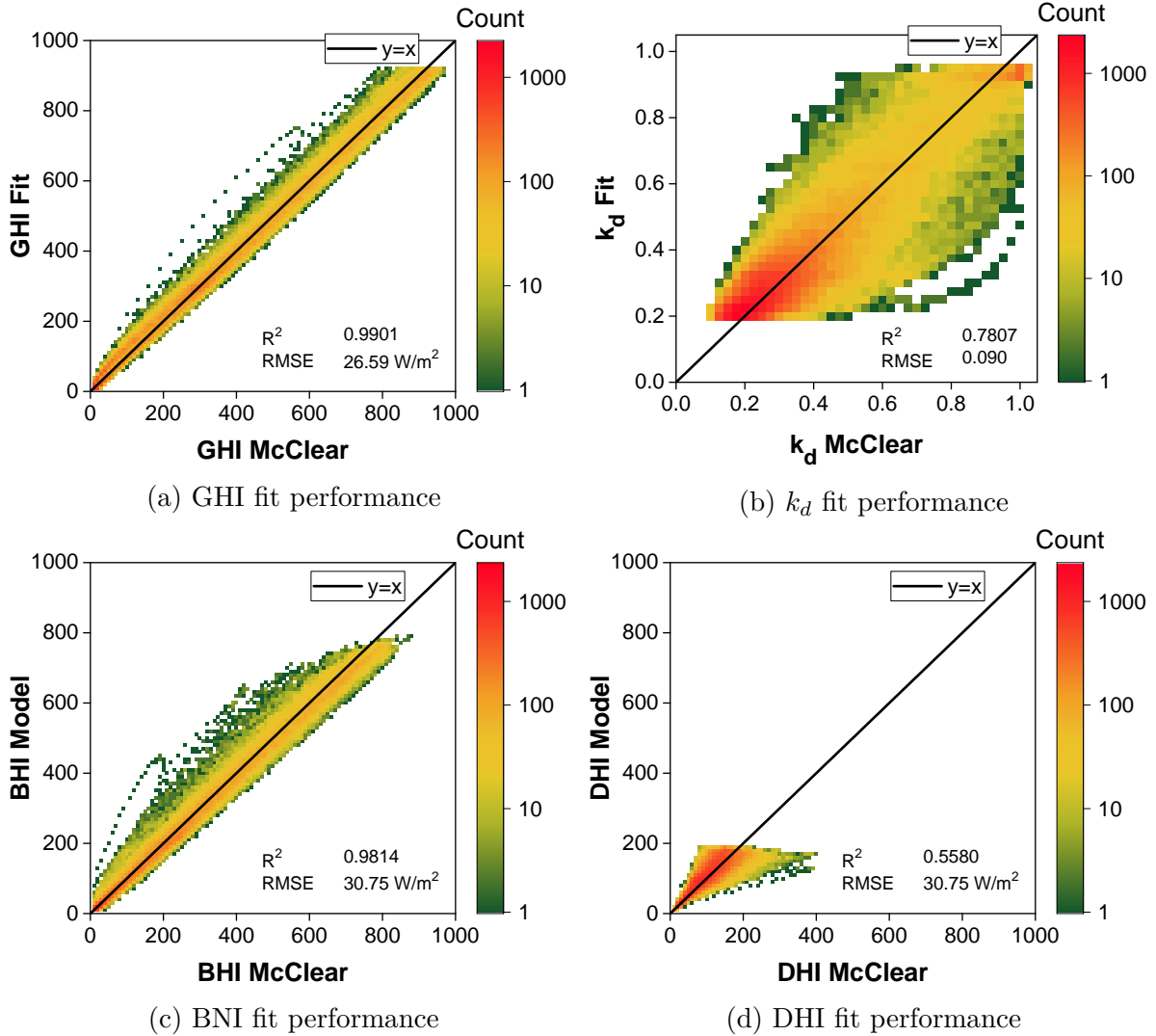
Figure 4-3: 2D histograms representing the performance of the fitting functions for (a) GHI, (b) k_d , (c) BHI, and (d) DHI, against the same 4 years of data. Figures (c) and (d) were reproduced using the McClear GHI and modelled k_d . The fitting functions show a high performance, indicated by the close proximity of red squares (representing high bin counts) to the y = x line.
