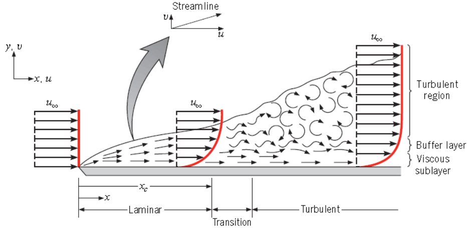
Figure C-4: Velocity boundary layer development on a flat plate. Source: [175]
