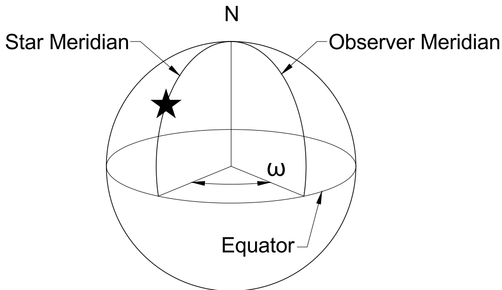
Figure 2-2: Sketch illustrating the local hour angle
