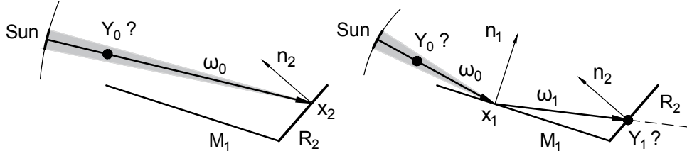
Figure 5-21: Illustration of vectors used in Equations (5.33) through (5.38)
