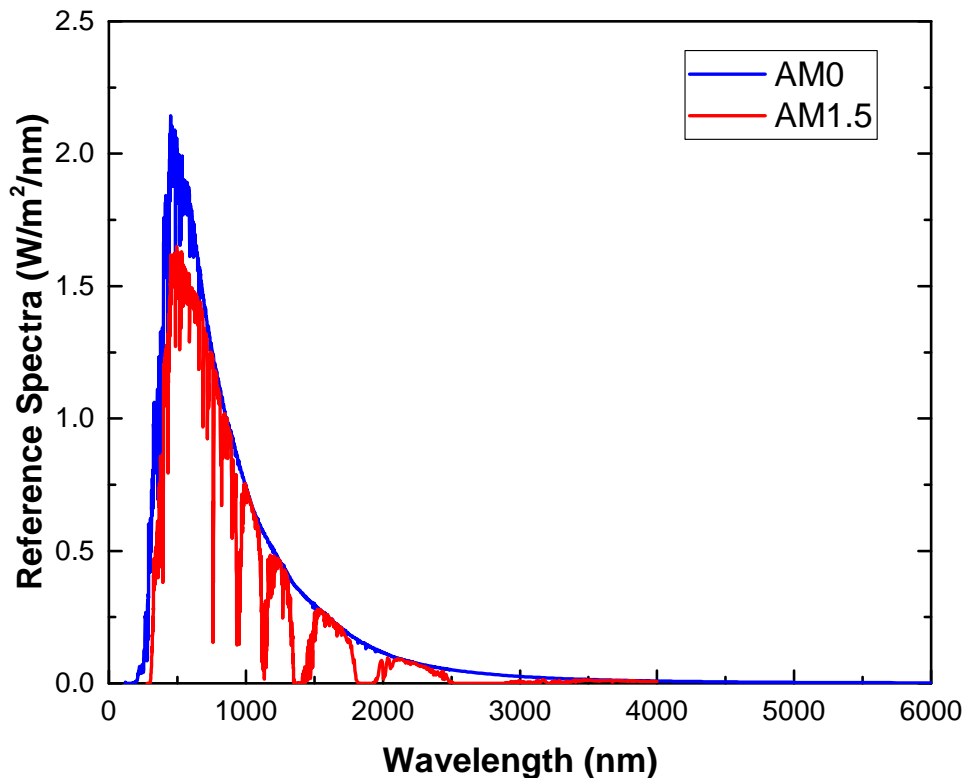
Figure 4-1: Reference spectra AM0 (TOA) and AM1.5, according to the standards ASTM E-490-00 and ASTM G-173-03, respectively. The difference between the two curves is due to the atmospheric attenuation of certain wavelengths.
