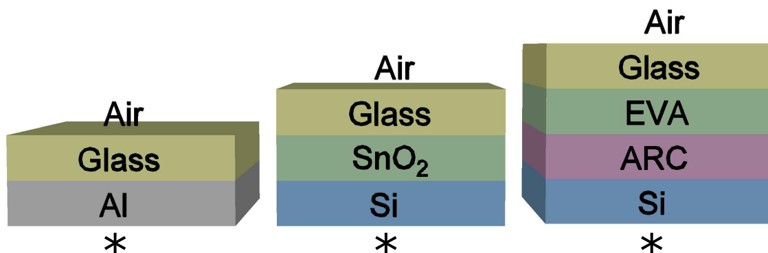
Figure 5-6: Principal material layers that photos interact with, present on the reflector (left), a -Si:H module (center), and p -Si module (right). Note that there are additional layers (not shown) below the presented structure, which do not interact with photons. The layer thicknesses are not to scale.
