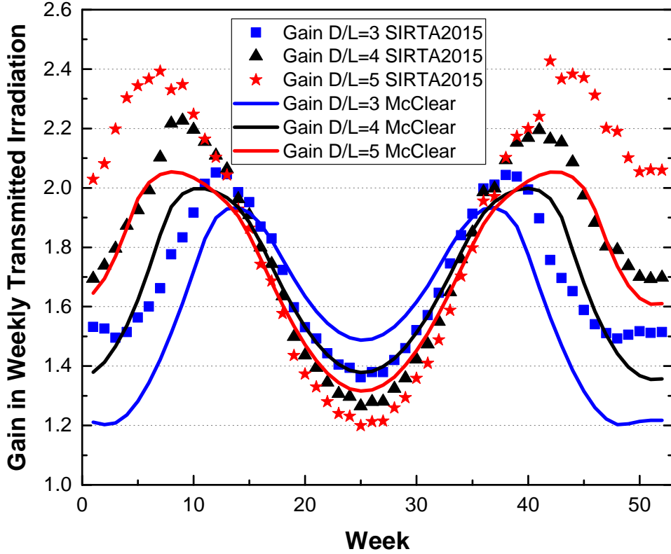
Figure 5-17: Weekly relative gains in transmitted irradiation of an optimised infinite PV+Reflector installation compared to an optimised infinite classical installation, under clear-sky (solid lines) and 2015 measured irradiance data (symbols). The two systems were optimised for annual transmitted energy at three different values of spacing D/L.
