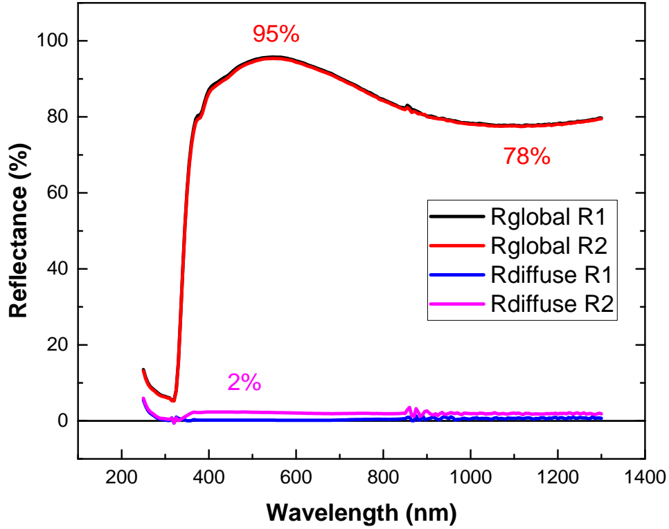
Figure 5-2: Laboratory measurements of global and diffuse reflectance as a function of wavelength for two reflector samples. Reflector sample R1 was cleaned before the measurement was taken. Reflector sample R2 was left in exterior conditions for two weeks, with visible dust on the surface, resulting up to 2% of incident flux being diffused.
