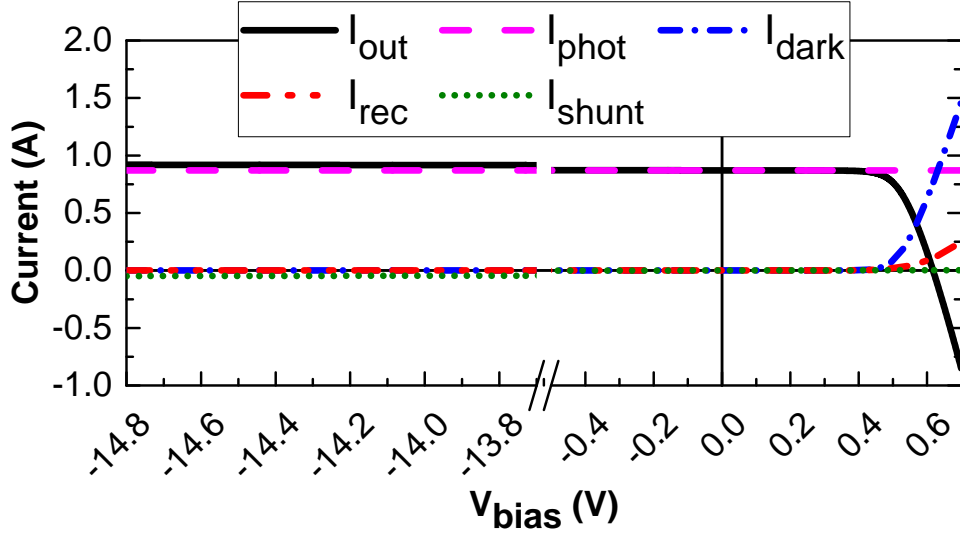
Figure 6-11: The I - V characteristics of each component of the double diode model circuit under STC conditions ( T=25\text{ }^{\circ}\text{C} , G_{POA}=1000\text{ W/m}^2 ). The following parameters were used: I_{01}=9.8 \times 10^{-11}\text{ A} , I_{02}=2.2 \times 10^{-7}\text{ A} , I_{SC,STC}=0.871\text{ A} , R_{sh}=3.0 \times 10^2\text{ }\Omega , R_s=4.2 \times 10^{-2}\text{ }\Omega , n_1=1.000 , and n_2=1.819 .
