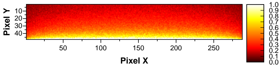
(c) Map B: Reflector contribution to the diffuse light on the reflector-equipped receiver
