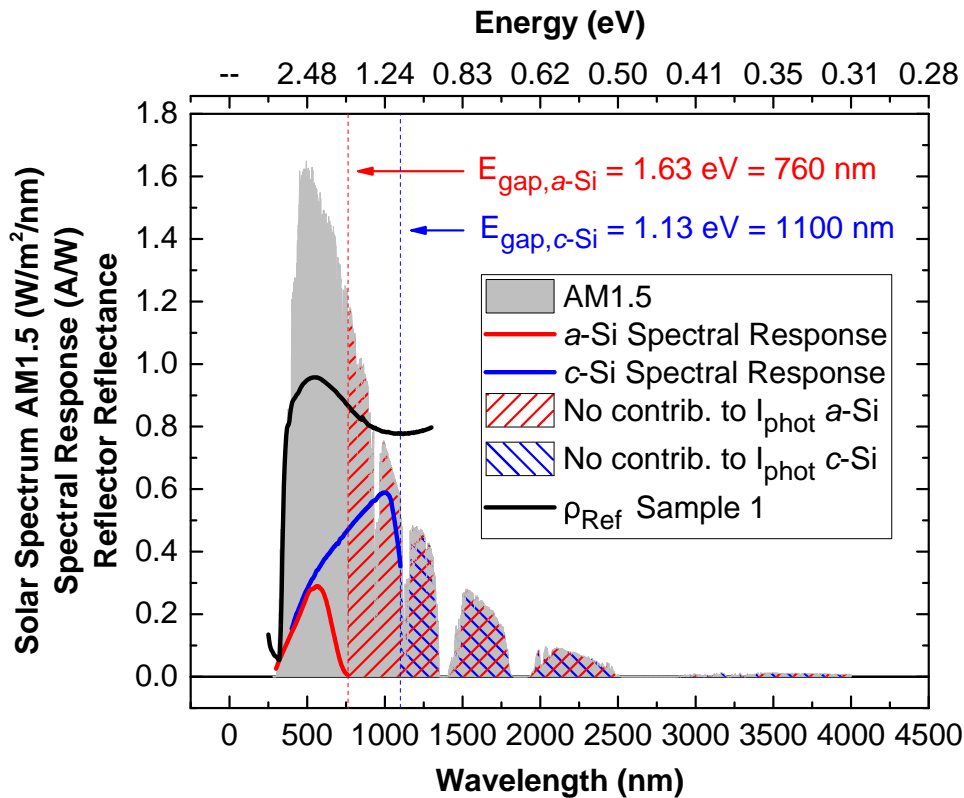
Figure 5-3: Measured spectral response of typical a -Si:H and c -Si modules (not the ones in the experiment). The AM1.5 spectrum and the reflector reflectance are given as a reference.
