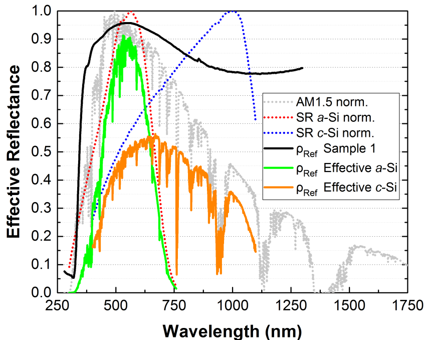
Figure 5-4: Calculated effective reflector reflectances for a -Si:H cells (green) and c -Si cells (orange), taking into account their spectral responses and the solar spectrum AM1.5. The effect of spectral transmittance is not incorporated here.
