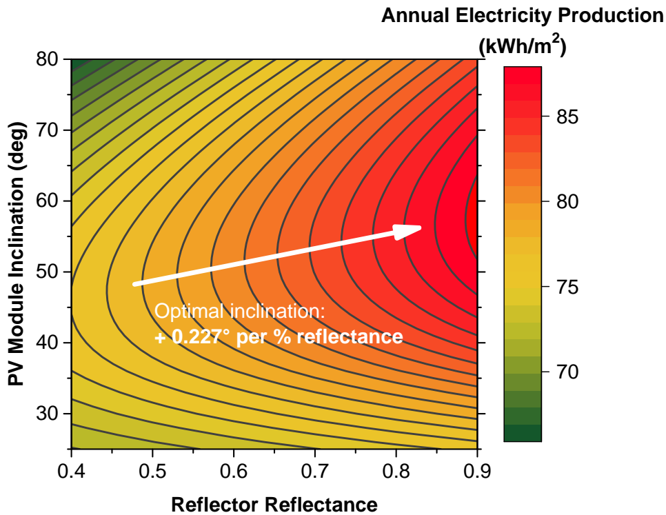
Figure 9-3: Annual energy production of a -Si:H modules equipped with planar reflectors, as a function of PV module inclination and mirror reflectance. Spacing between contour lines: 1 kWh/m 2 .
