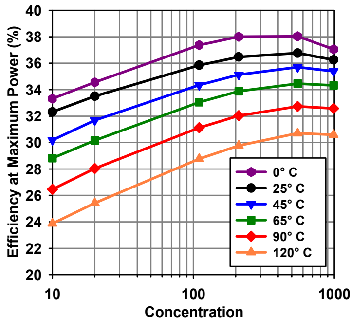
Figure 1-11: Relationship between the efficiency and the concentration factor for Spectrolab's CDO-100 concentrator solar cell at different operating temperatures. Source: Spectrolab, 2008 [63]
