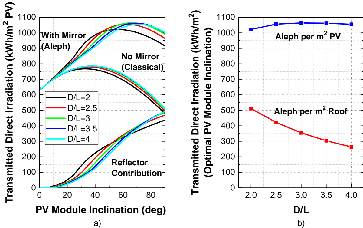
Figure 5-26: Geometrical optimisation of the Aleph system for different inter-row spacings D/L : (a) Transmitted direct irradiation for Aleph and classical installations, along with the associated reflector contribution; (b) Effect of D/L on the transmitted direct irradiation.
