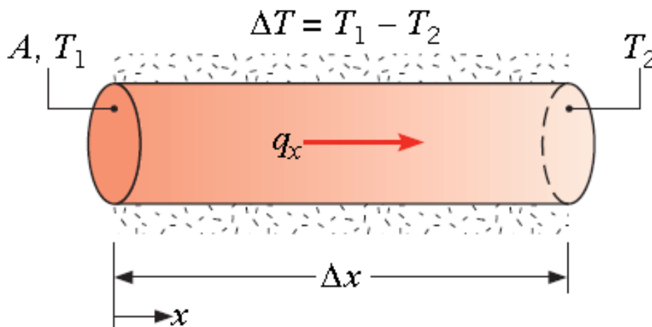
Figure C-1: Steady-state heat conduction experiment. Source: [175]
