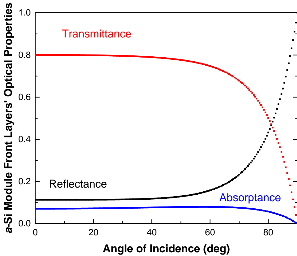
Figure 5-8: Modelled optical performance of the a -Si:H module front layers.
