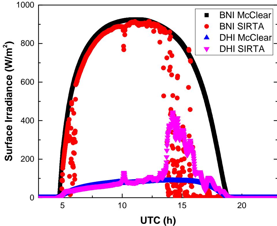
Figure 4-2: Measured and McClear-estimated surface irradiance on 16. August 2013. The day was relatively clear in the morning, and cloudy in the evening.
