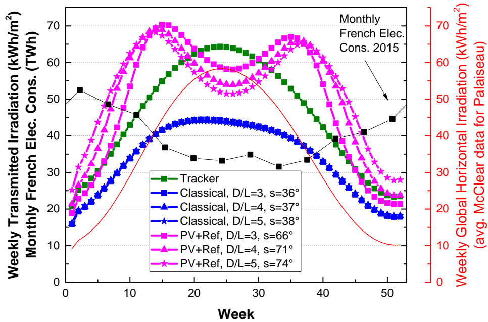
Figure 5-14: Total weekly transmitted irradiation under clear-sky conditions for a PV tracker, an infinite classical installation and an infinite PV+Reflector installation, the latter two being optimised for annual transmitted energy at three different values of spacing D/L .
