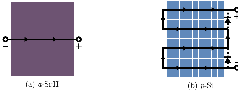
Figure 3-10: Module electrical interconnections: a) a -Si:H module: 14 tandem a -Si:H cells connected in series. No bypass diodes are installed; b) p -Si module: 2 strings of 18 cells connected in series with a bypass diode across each string.
