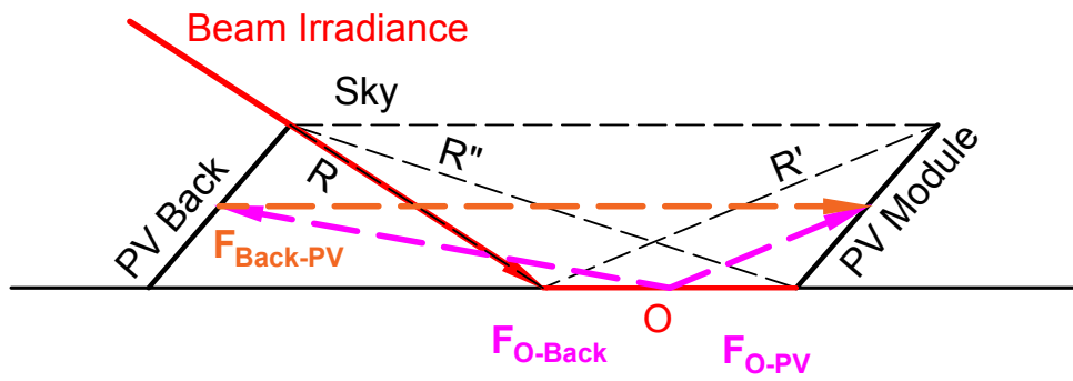
(c) View factors for classical installations, part 2
