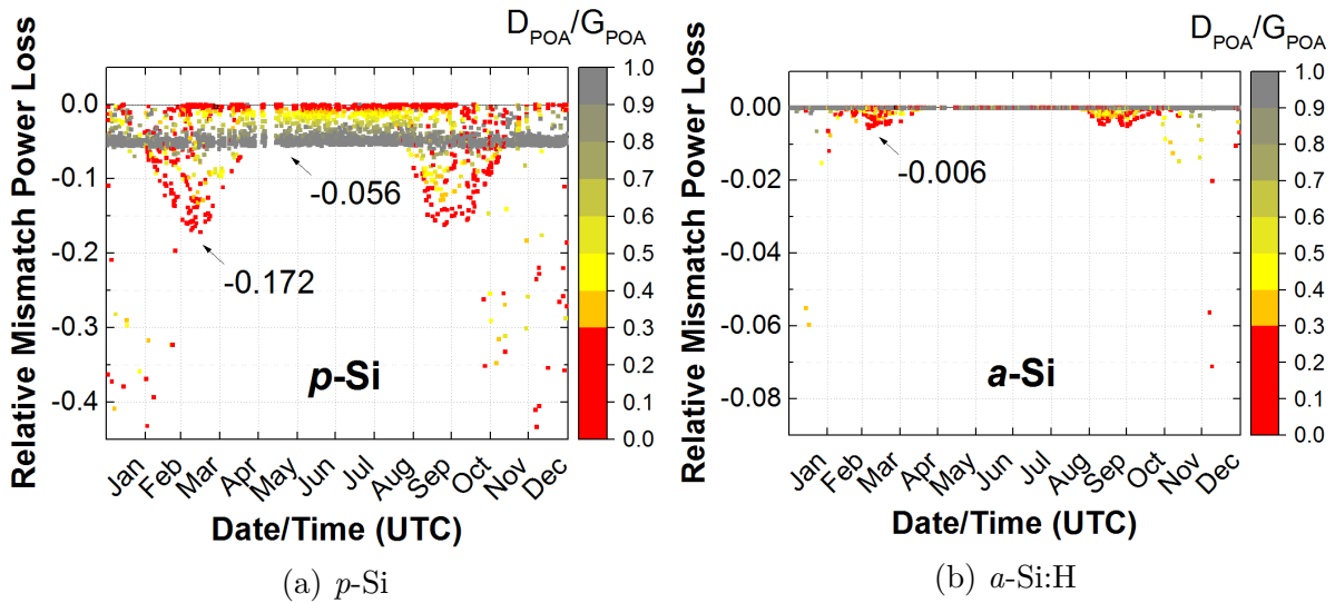
Figure 9-7: Relative power losses due to string mismatch in reflector-equipped modules, for (a) a central p -Si module, and (b) a central a -Si:H module. The relative losses in the annual produced energy are 2.82% and 0.02% for p -Si and a -Si:H modules, respectively.
