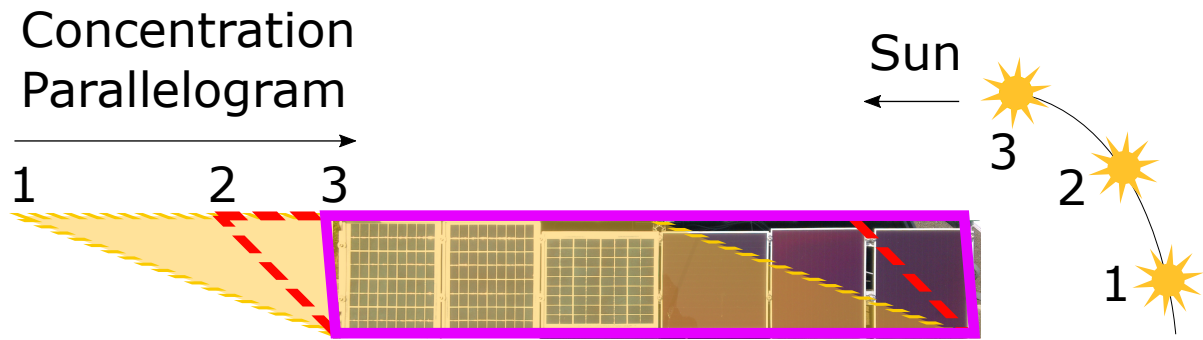
Figure 3-11: Edge effect sketch, showing the eastward movement of the concentration zone in the plane of the second row PV modules throughout the morning period. The edge effect is the most severe for the far-edge modules.
