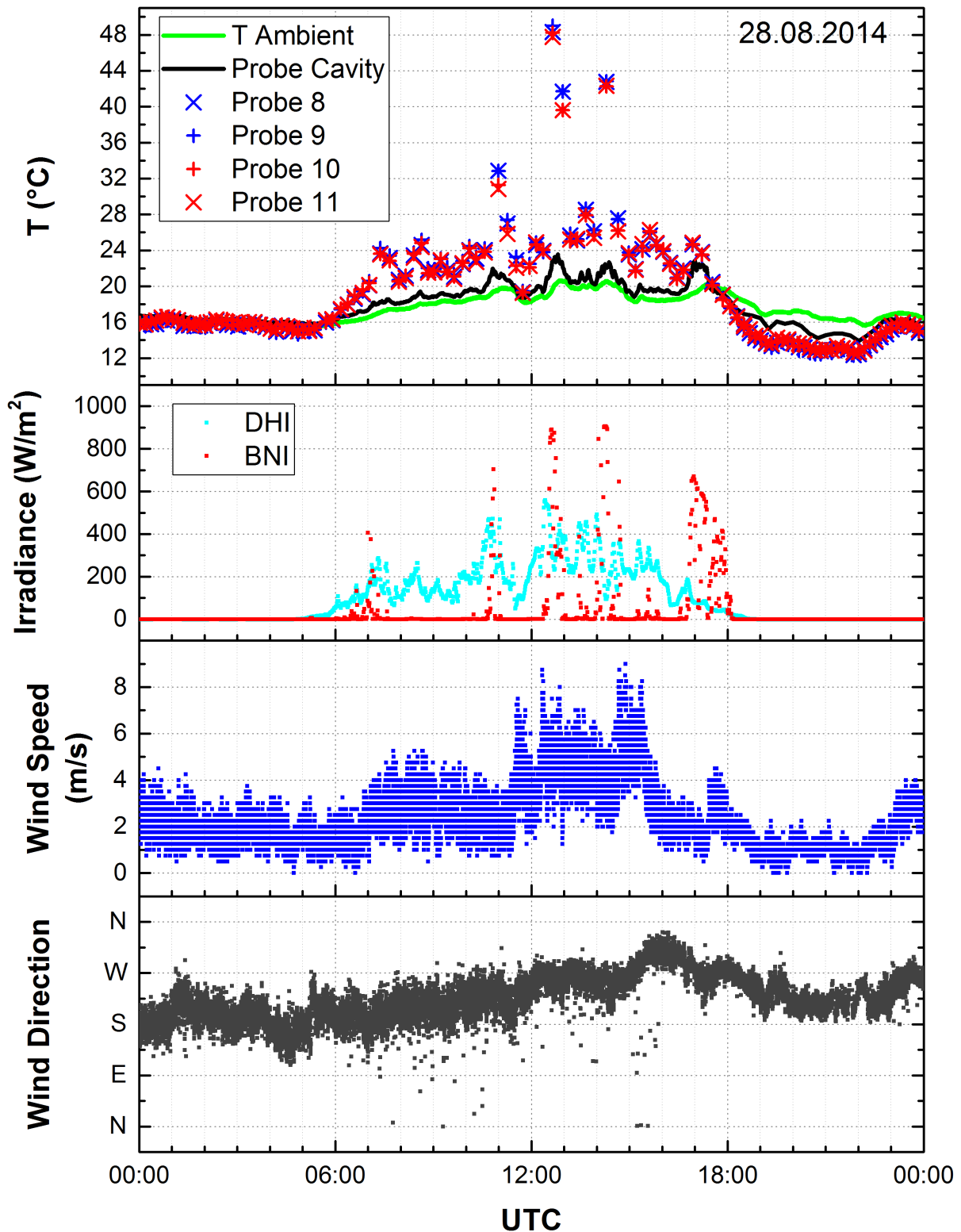
Figure 3-13: Experimental data taken on August 28th, 2014, a cloudy day. (Top graph) Green line: ambient temperature probe; black line: probe situated inside the back triangular cavity; blue symbols: probes on p -Si modules; red symbols: probes on a -Si:H modules. (Lower graphs) Cyan and red: diffuse horizontal and beam normal irradiances, respectively; blue and gray: wind speed and direction, respectively.
