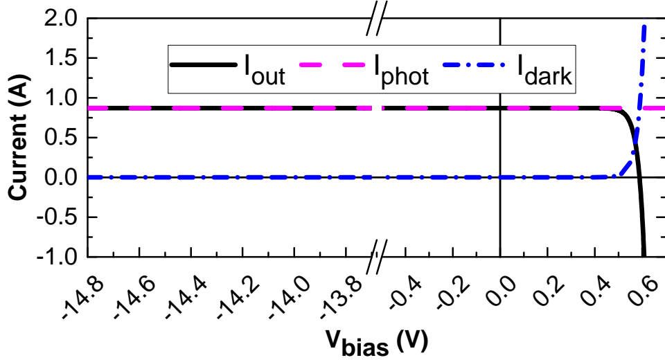
Figure 6-7: The I - V characteristics of each component of the ideal cell model circuit under STC conditions ( T=25\text{ }^\circ\text{C} , G_{POA}=1000\text{ W/m}^2 ). The following parameters were used: I_0=9.8 \times 10^{-11}\text{ A} , I_{SC,STC}=0.871\text{ A} . The axis break is shown to demonstrate that the currents stay the same at high negative polarisations.
