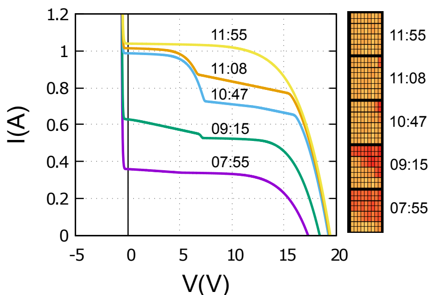
Figure 9-5: Simulated I-V characteristic of an edge p -Si module, equipped with two bypass diodes, resulting from different distributions of the concentration zone and hence degrees of string mismatch. The bypass diodes are active in mismatch conditions, as well as in reverse bias.
