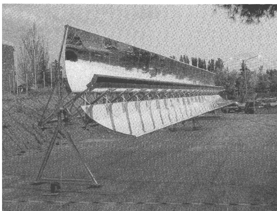
(a) EUCLIDES prototype
