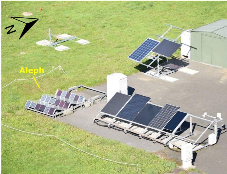
Figure 1-14: Aerial view of the three PV systems installed in SIRTÀ: Aleph (left center), tracker (right top) and classical fixed-mount (right bottom). Photo credit: Jordi Badosa
