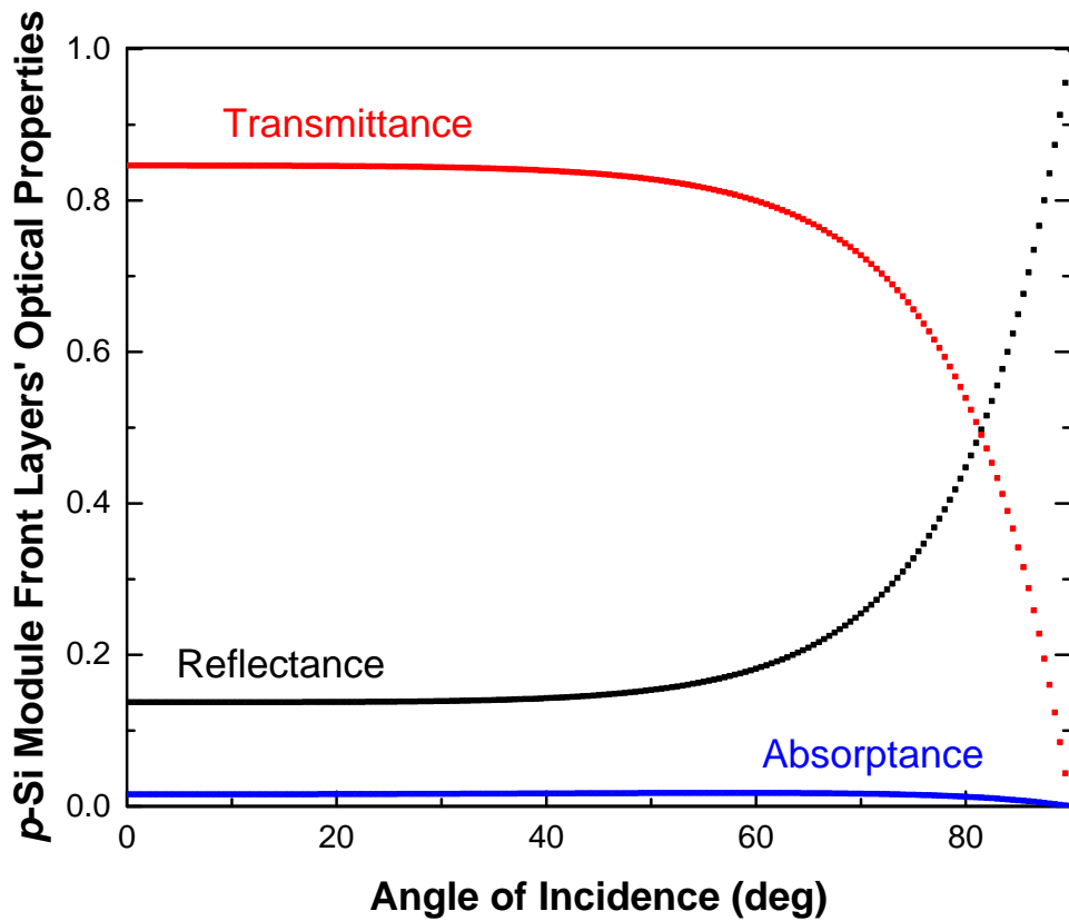
Figure 5-9: Modelled optical performance of the p -Si module front layers.
