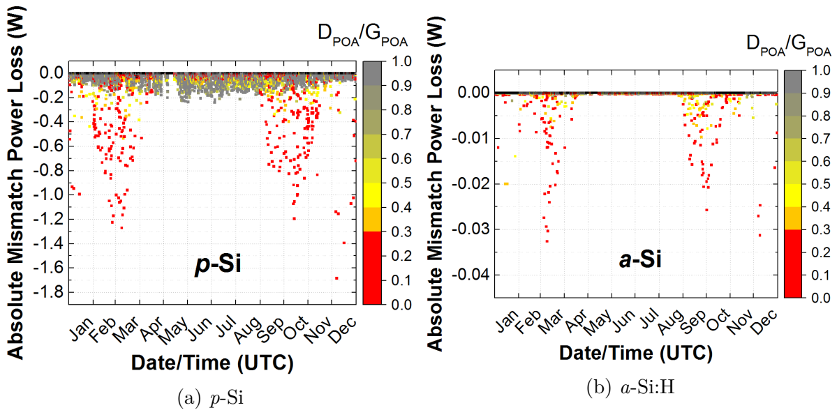
Figure 9-8: Absolute string mismatch power losses in reflector-equipped modules, for (a) a central p -Si module, and (b) a central a -Si:H module
