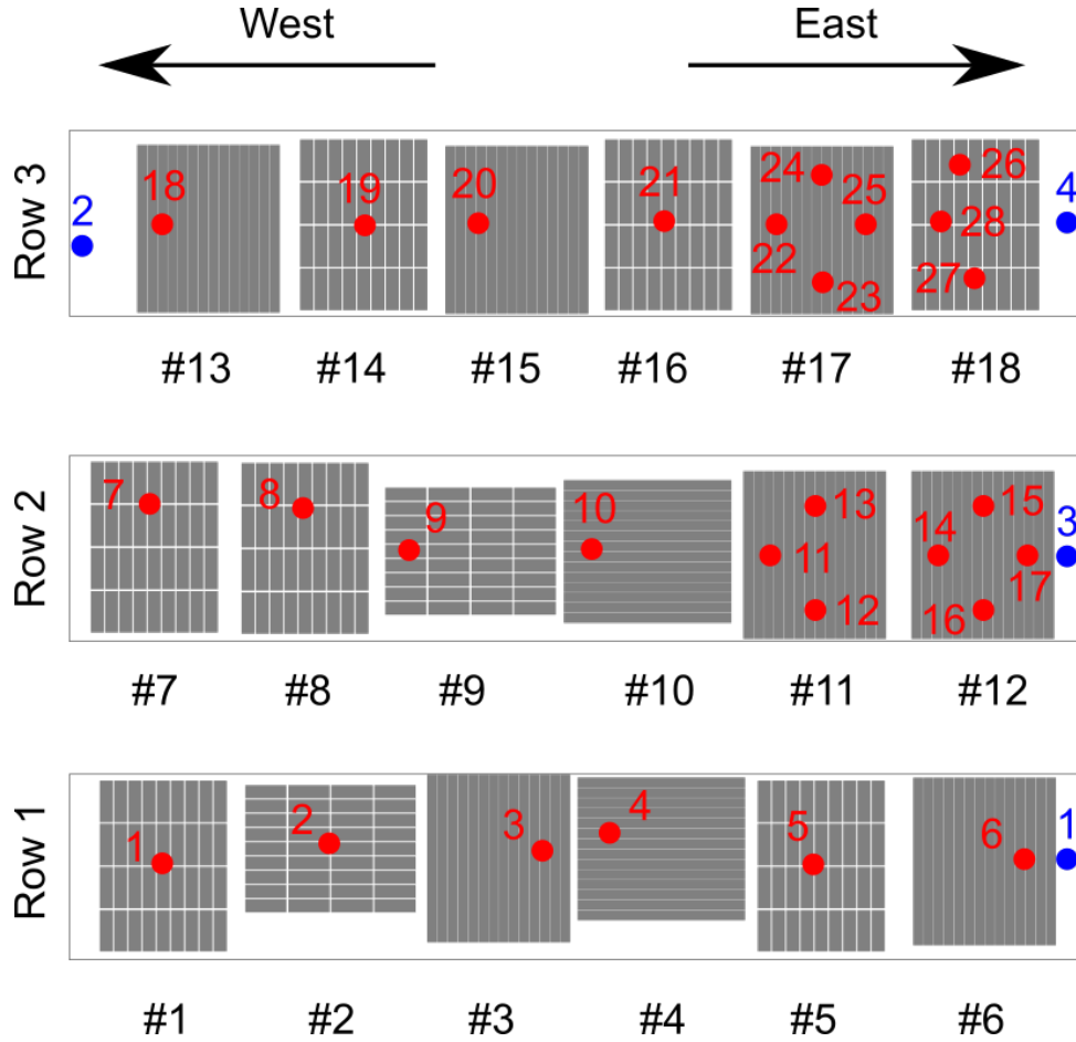
Figure 3-3: Positions and labelling of: (gray) 18 PV modules amongst the three rows; (red) 28 temperature probes Pt-100, attached to the backsheets of the modules; (blue) 4 reference cells RG-100.
