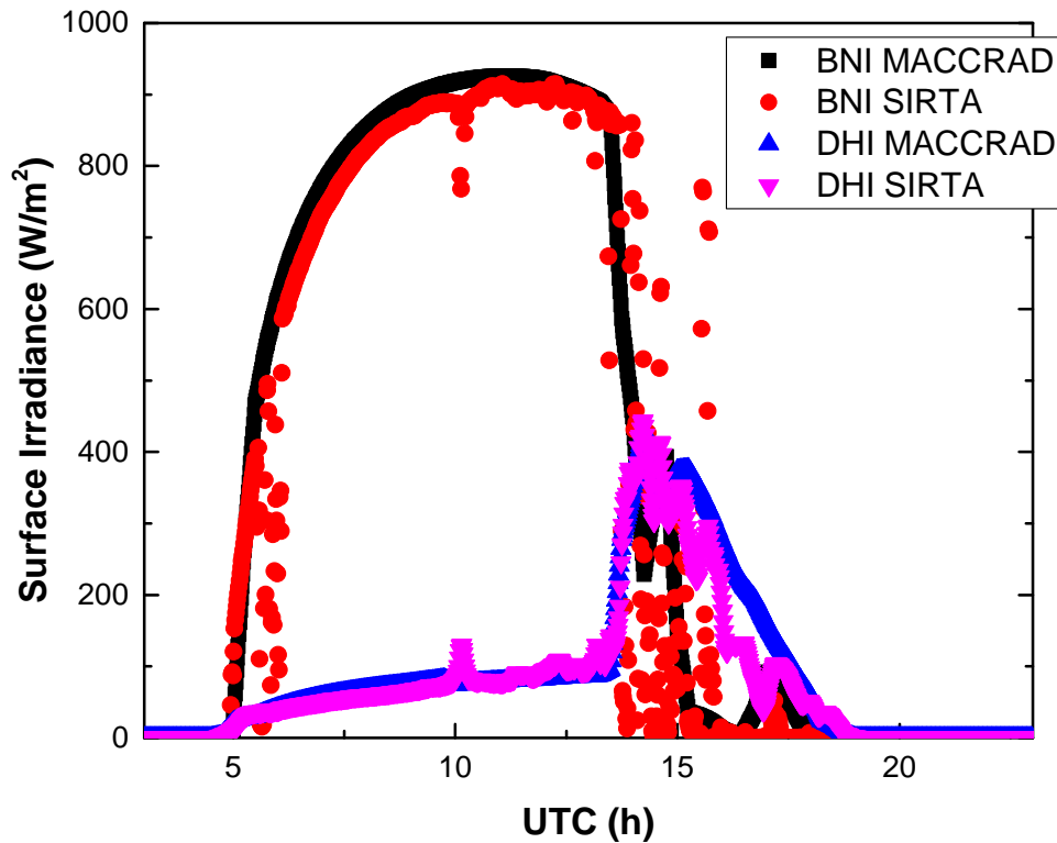
Figure 4-4: Measured and MACC-RAD-estimated surface irradiance on 16. August 2013.
