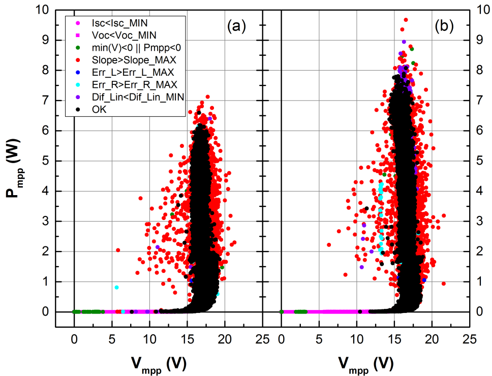
Figure 3-7: Visualisation of the filters as applied to almost two years of measurements (31.03.2014 - 07.03.2016), for (a) module 6 (a frontal a -Si:H module), and (b) module 15 (a reflector-equipped a -Si:H module).
