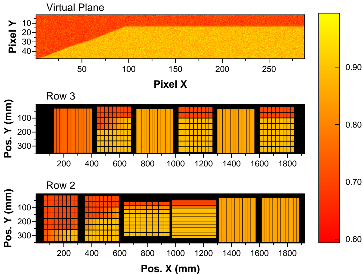
Figure 5-25: Result of the mapping algorithm, calculating the average shape factor by cell from several flux maps (in this case from a -Si:H and p -Si direct flux shape factor maps on October 15, 2014 at 13:50 UTC).
