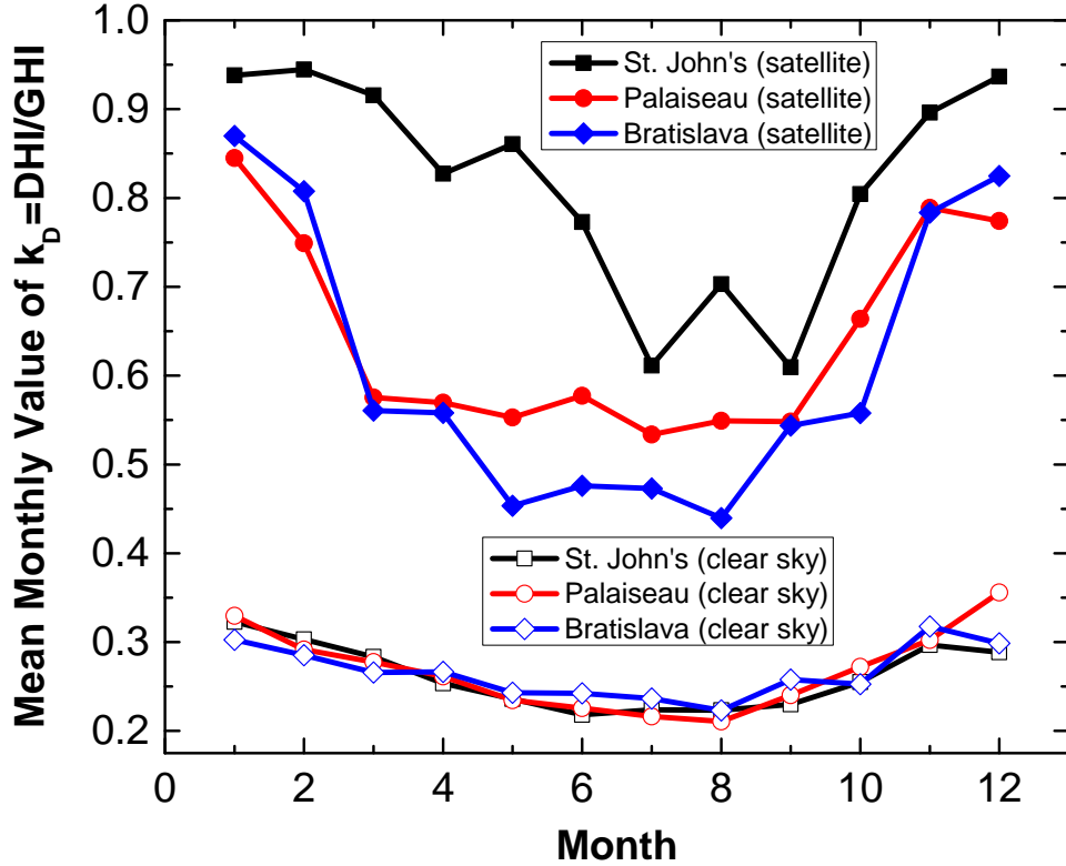
Figure 9-2: Comparison three cities' climates based on the 4-year average mean monthly value of k_D , the diffuse component of the global horizontal irradiance. Filled symbols represent the satellite-estimate surface irradiance, empty symbols represent the local clear-sky surface irradiance [95].
