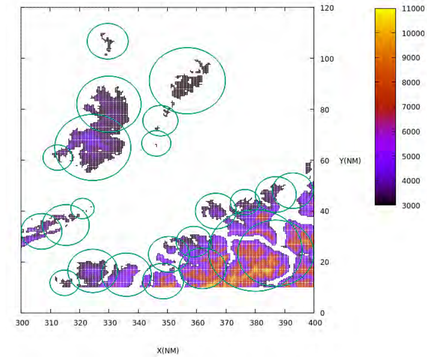
Figure 6.19: Obstacles modeling in the TMA of Zurich airport, illustration in 2D.
