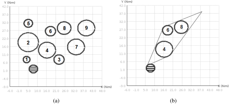
Figure 4.14: Test 1, obstacles illustration. (a) Buffer obstacle (striped) and 9 obstacles. (b) 3 remaining obstacles after using CVH-filter.
