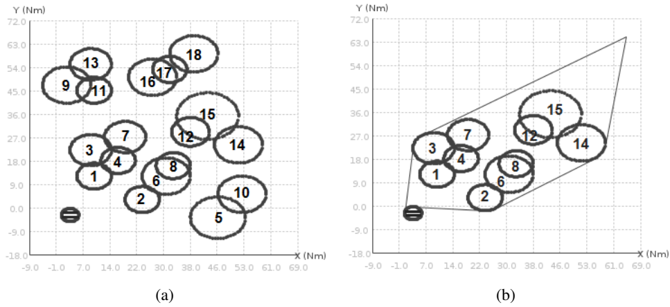
Figure 4.18: Test 3, obstacles illustration. (a) Buffer obstacle (striped) and 18 input obstacles. (b) 10 remaining obstacles after using CVH-filter.
