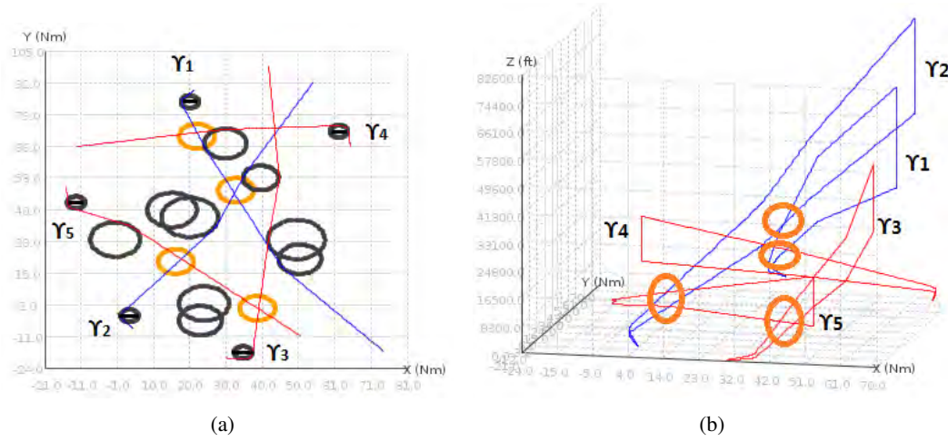
Figure 6.5: Test 2: routes generated independently by B&B and initial conflicting areas (orange circles). (a) Illustration in 2D. (b) Illustration in 3D.
