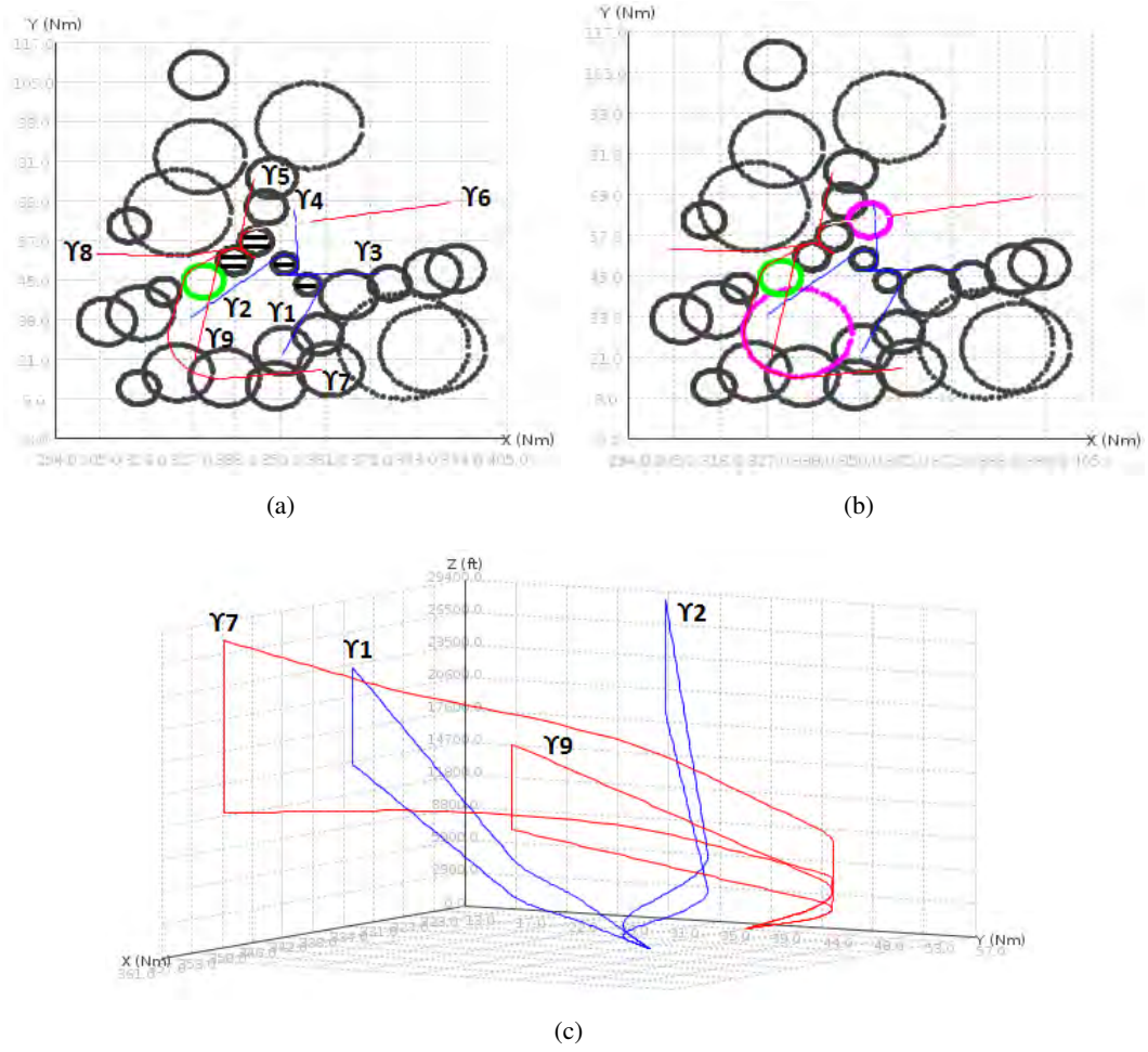
Figure 6.26: Test Zurich airport: SA method simulation results. (a) Illustration in the horizontal plane. (b) Fictitious obstacles for route deviation. (c) Illustration of \gamma_1 , \gamma_2 , \gamma_7 and \gamma_9 in 3D.
