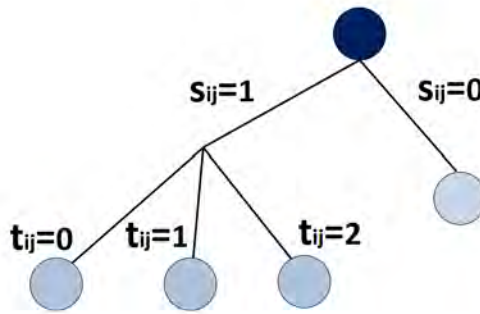
Figure 4.7: Branch and Bound branching strategy in our method.
