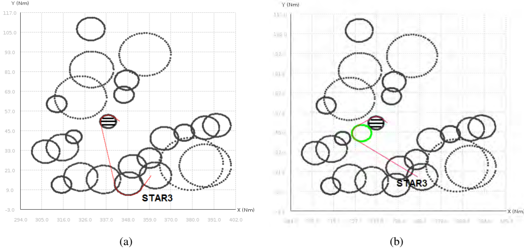
Figure 6.22: Building route \gamma (a) Simulation result of \gamma by using the B&B independently. (b) Simulation result of \gamma after adding the fictitious obstacle corresponding to the IAF (in green color).
