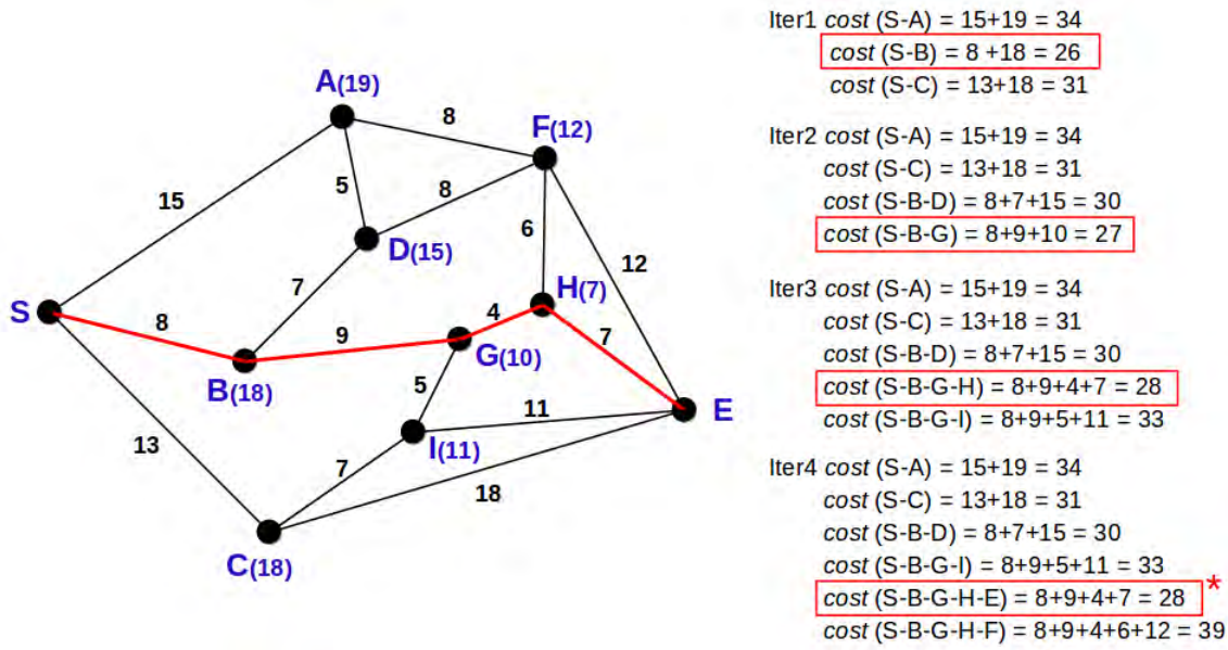
Figure 1.13: An example of the A* algorithm. The value in the brackets after each node denotes the heuristic cost of that node.
