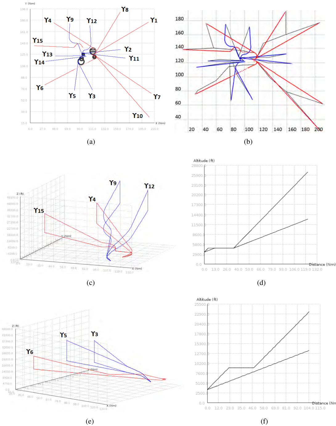
Figure 6.12: Test Paris CDG airport: B&B-based method simulation results. (a) Illustration in the horizontal plane. (b) Comparison with standard routes. (c) Illustration of \gamma_4, \gamma_9, \gamma_{12} and \gamma_{15} . (d) Illustration of \gamma_{15} in the vertical plane. (e) Illustration of \gamma_3, \gamma_5 and \gamma_6 . (f) Illustration of \gamma_6 in the vertical plane.
