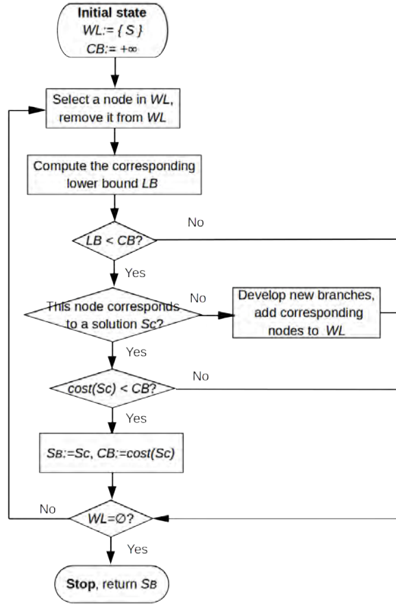
Figure 1.12: B&B flow chart.
