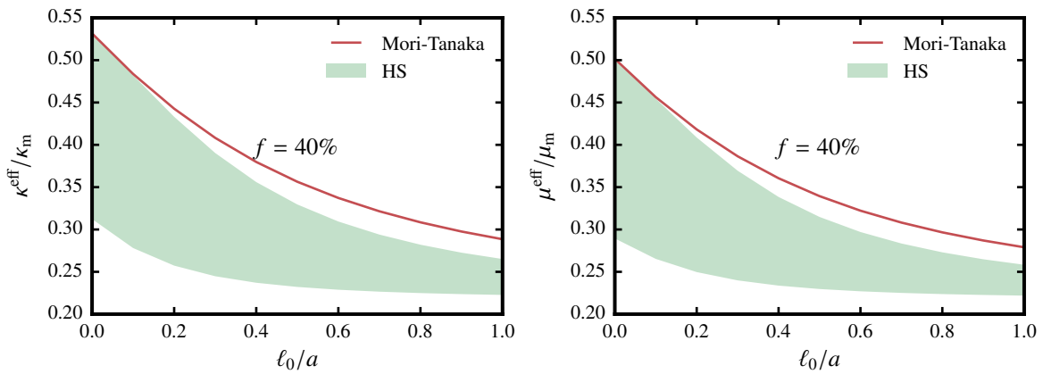
Figure 8.5. Soft inhomogeneity case: Hashin-Shtrikman bounds derived by using the Verlet-Weiss model on the effective bulk (left) and shear (right) moduli. \mu_i = 0.1\mu_m, \nu_i = \nu_m = 0.125 . The volume fraction is fixed at 40%.
