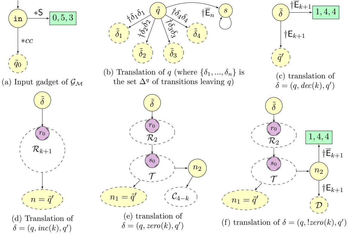
Figure 4.9 – Description of the encoding \mathcal{G}_M . Modules are \mathcal{R}_k and \mathcal{T} are copied several times. n = \tilde{q} means the terminal state n of a module is replaced by further encoded state \tilde{q} .
