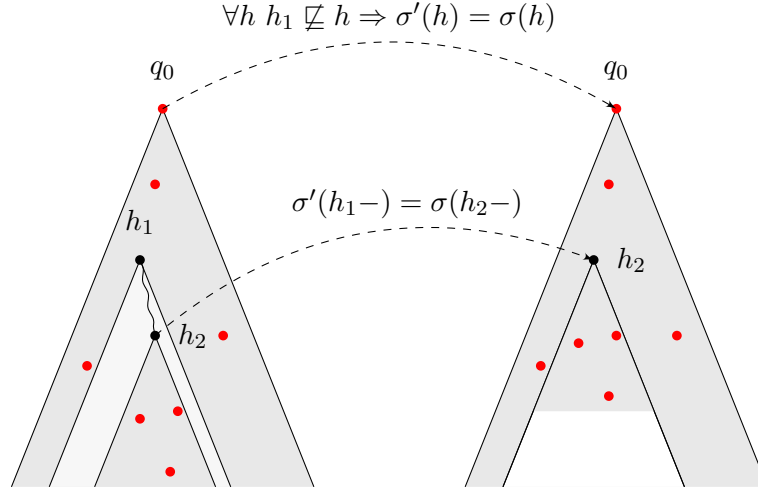
Figure 11.2 – Illustration of the proof of Theorem 11.13, when h_1 \subseteq h_2 , first(h_1) = first(h_2) and subtrees rooted in h_1 and h_2 contain the same set of important nodes (in red). Since, h_1 and h_2 have the same final state, we can replace strategy from subtree rooted in h_1 by the one rooted in h_2 (same allowed actions). This is possible since all the important nodes are in the subtree rooted in h_2 or outside the subtree rooted in h_1 , therefore all removed nodes and transitions can be generated from somewhere else.
