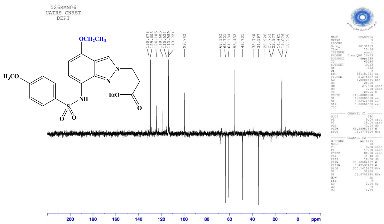
Figure 4: Spectre RMN 1 H (CDCl 3 ) du composé 34b
