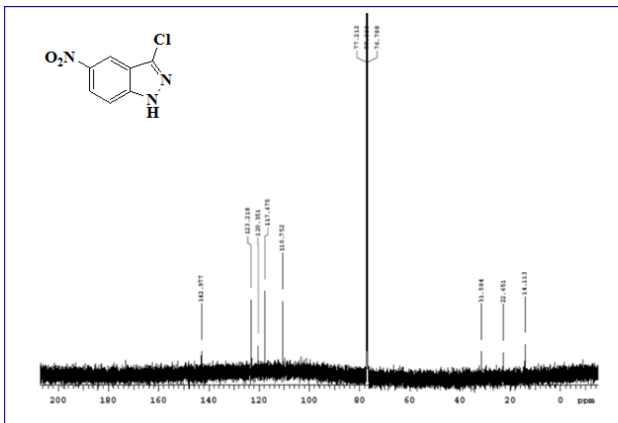
Figure 6 : Spectres RMN 1 H et RMN 13 C (CDCl 3 ) du 3-chloro-5-nitroindazole 6
