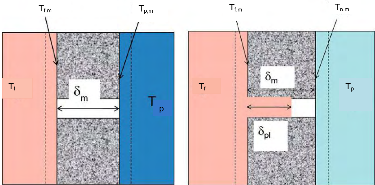
Figure 7.3: Schematic of dry and wet pore in MD (left and right respectively)
