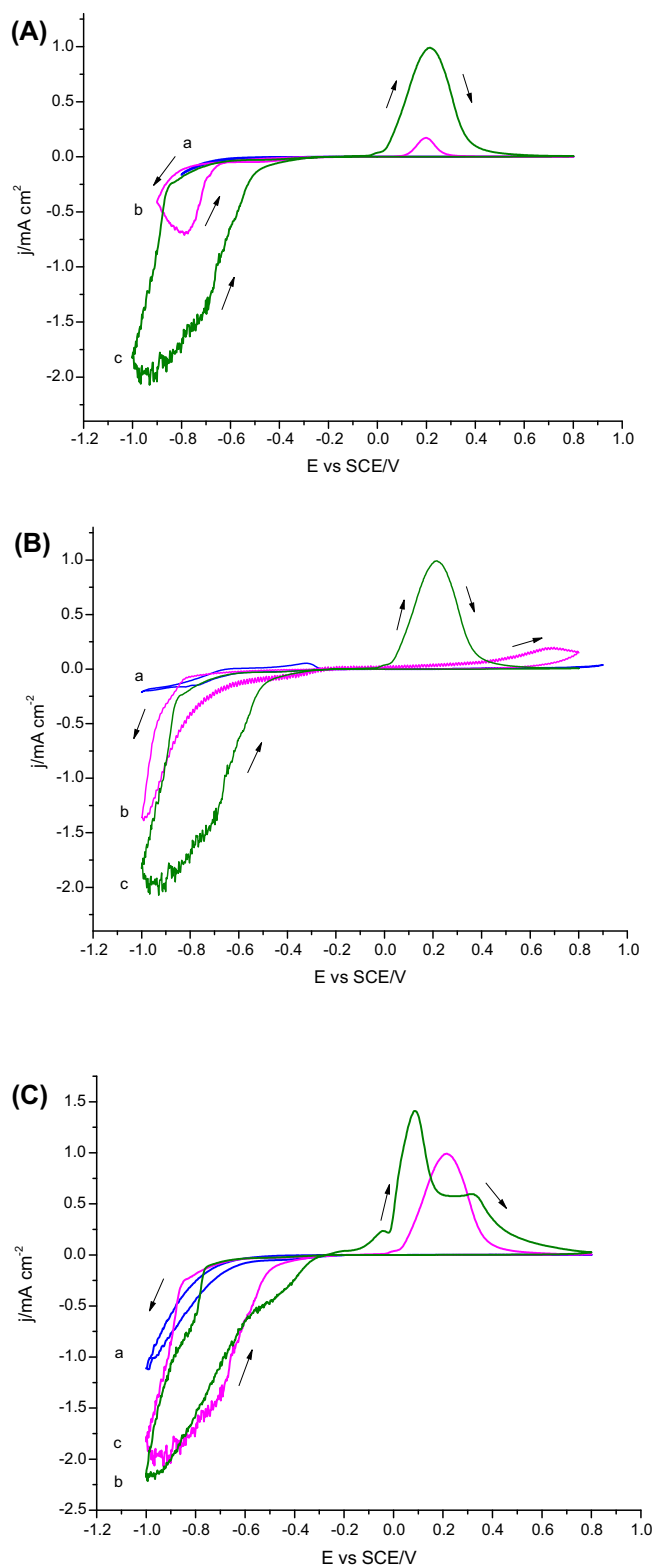
Fig. 1. Cyclic Voltammograms measured at 10 \text{ mV.s}^{-1} scan rate. (A) 0.2 \text{ M Ni(NO}_3)_2 in DMSO electrolytic solution in equilibrium with air (salt dissolved under argon). Effect of the negative potential limit: (a) -0.80 \text{ V} , (b) -0.90 \text{ V} and (c) -1.00 \text{ V} . (B) Cyclic Voltammograms of a 0.4 \text{ M KNO}_3 (curve a) and 0.2 \text{ M Ni(NO}_3)_2 in DMSO electrolyte in equilibrium with air (curve b and c). Effect of the solution conditioning upon \text{Ni(NO}_3)_2 dissolution: air (curve b) and argon (curve c). (C) Effect of gas bubbling in the 0.2 \text{ M Ni(NO}_3)_2 in DMSO bath: (a) Oxygen bubbling, (b) argon bubbling and (c) without bubbling (equilibrium with air).
