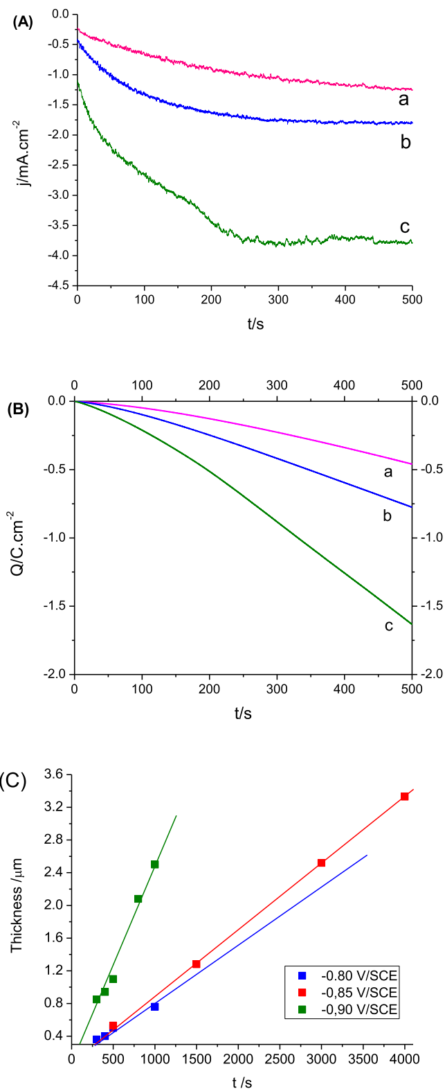
Fig. 2. (A) Deposition current curves measured in 0.2 \text{ M Ni(NO}_3)_2 -DMSO at (a) -0.80 \text{ V/SCE} , (b) -0.85 \text{ V/SCE} and (c) -0.90 \text{ V/SCE} . (B) Electrical charge density exchanged upon the experiment shown in (A). (C) Variation of the mean layer thickness with deposition time and applied potential.
