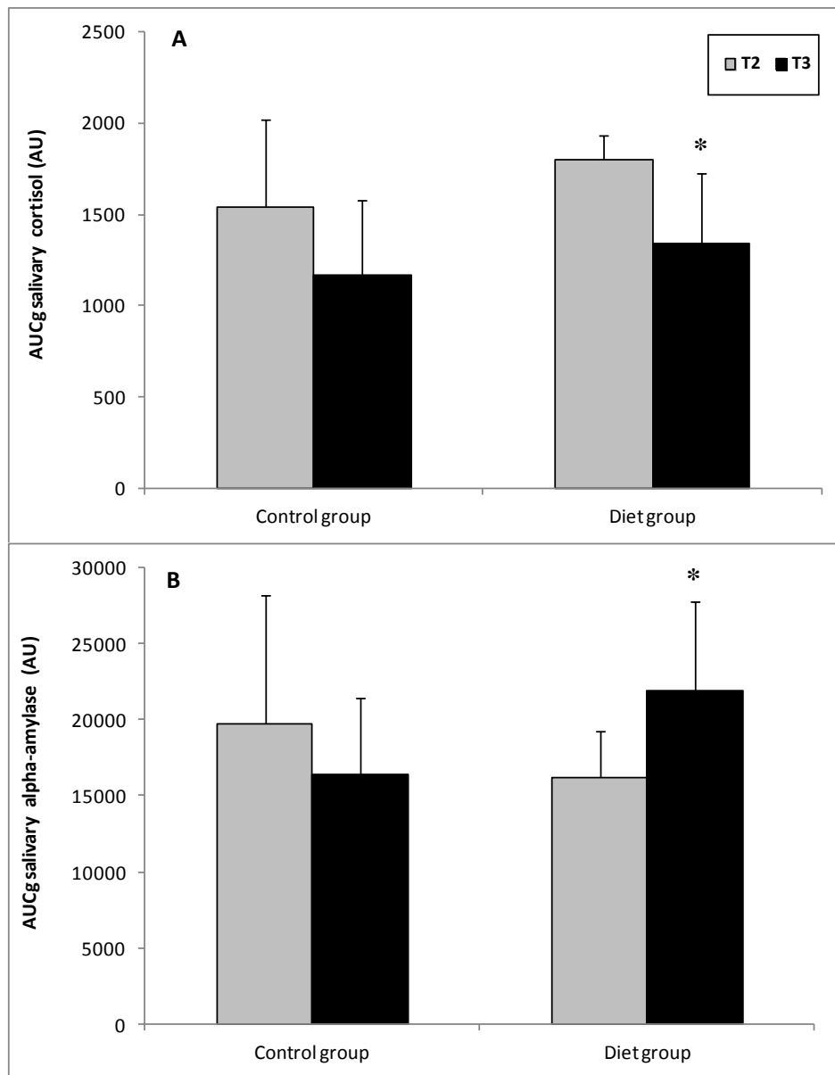
Figure 3: AUC gsC (A) and AUC gsAA (B) (mean ± SEM) during a simulated weightlifting competition held during a weight maintenance period (T 2 ) and after a six-day period of food restriction (T 3 ) for the Diet group only. * Significant difference between both periods (T 2 vs T 3 ) ( P < 0,05 ).
