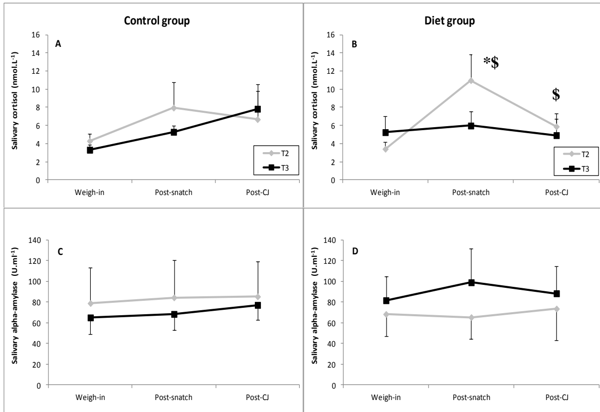
Figure 2 : Salivary cortisol concentrations and sAA activity (mean \pm SEM) for the Control group (A-C) and the Diet group (B-D) at weigh-in (Weigh-in, 02:00-02:15 PM), after the third snatch attempt (Post-snatch, 04:45-05:00 PM) and after the third CJ attempt (Post-CJ, 05:45-06:00 PM) of a simulated competition held during a weight-maintenance period (T 2 ) and after a six-day period of food restriction (T 3 ) for the Diet group only.* Significant difference between both periods (T 2 vs T 3 ) ( P < 0.05 ). $ Significant difference from the preceding point in time ( P < 0.05 ).
