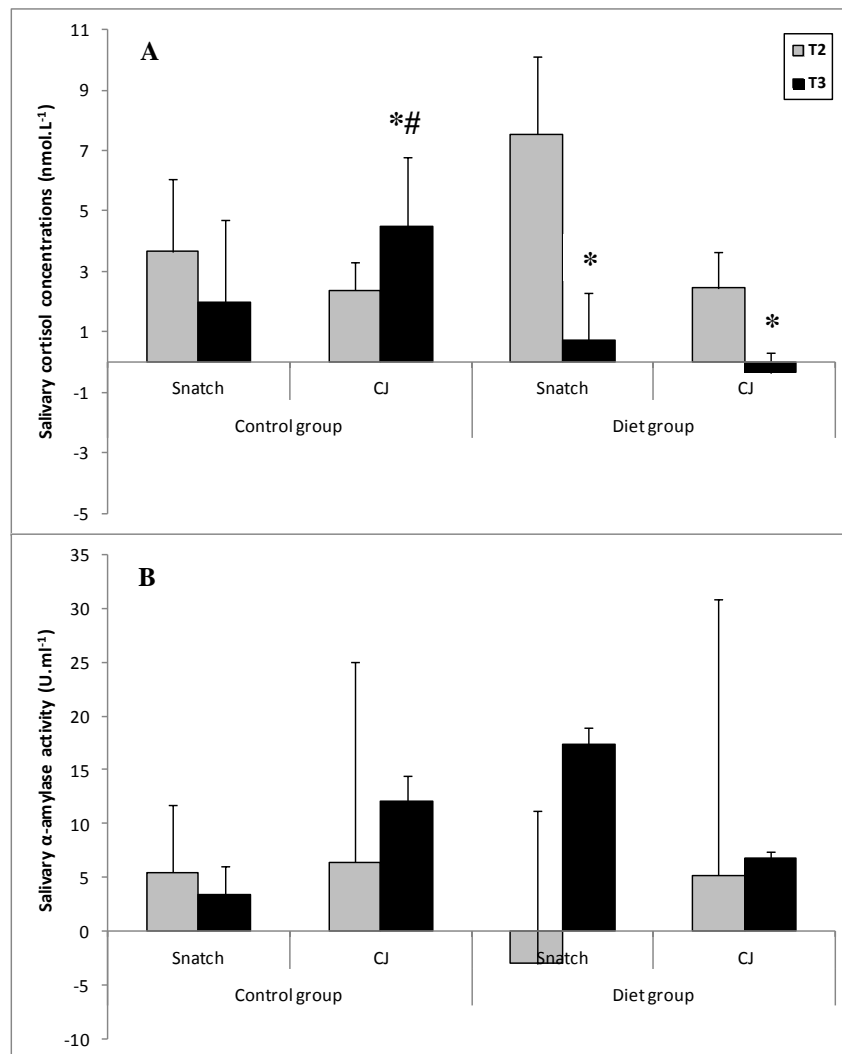
Figure 4: Post-snatch and post-CJ variation for salivary cortisol concentrations (A) and sAA activity (B) (mean ± SEM) during a simulated weightlifting competition held during a weight maintenance period (T 2 ) and after a six-day period of food restriction (T 3 ) for the Diet group only. The variation was calculated based on the difference between the weigh-in value and the post-snatch or CJ values. * Significant difference between both periods (T 2 vs T 3 ) ( P < 0.05 ). # Significant difference between groups at the same time point ( P < 0.05 ).
