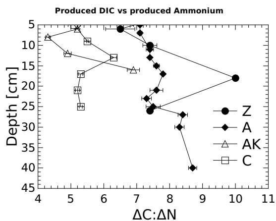
Figure 5.3 – \frac{\Delta DIC}{\Delta NH_4} porewater ratio of the investigated stations.
