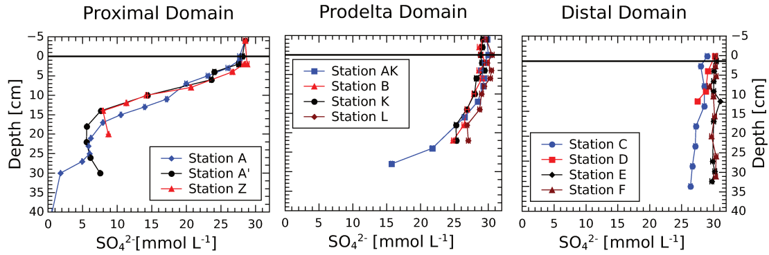
Figure 3.8 – Sulfate profiles measured in the porewaters (mmol L -1 ) of the proximal, the prodelta and in the distal domains.
