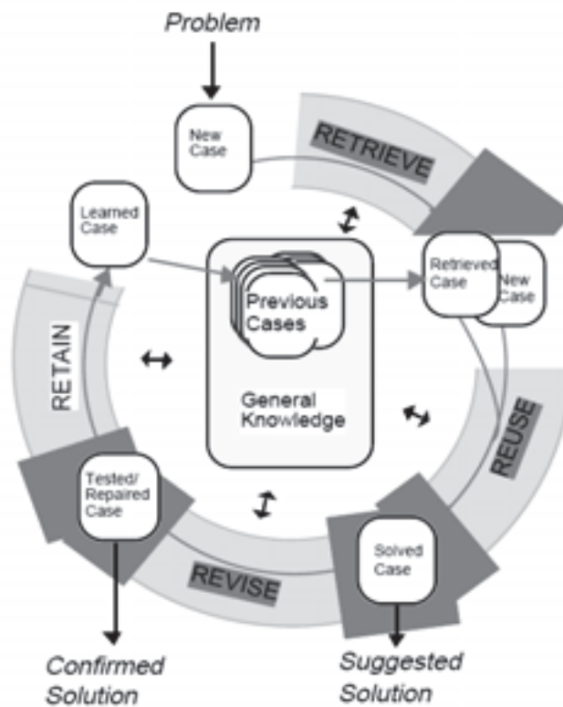
Figure 14: CBR Cycle (Aamodt & Plaza, 1994)
