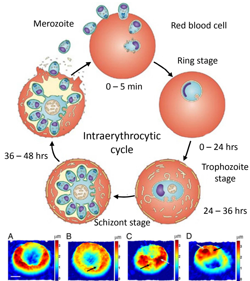
Figure 2.4 Schematic illustration of the intraerythrocytic cycle of malaria infection and its 3D phase mapping at various stages [33]: (A) healthy cell; (B) Ring stage; (C) trophozoite stage; and (D) Schizont stage; where black arrows indicate the merozoite and gray arrows indicate the hemozoin.
