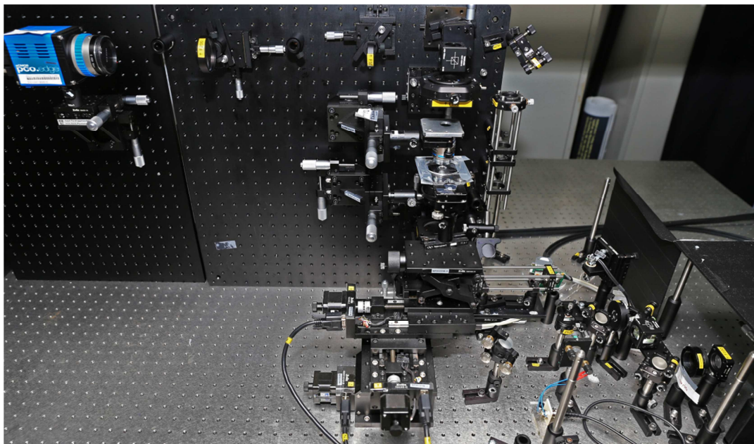
Figure 4.7 Photograph of the optical setup of the ODT system
