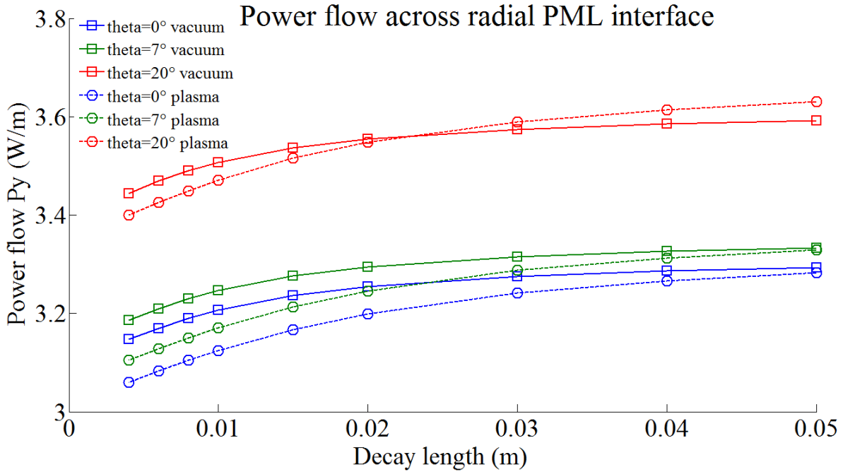
Figure 3.22. Radial power flow w.r.t decay length, case 1
