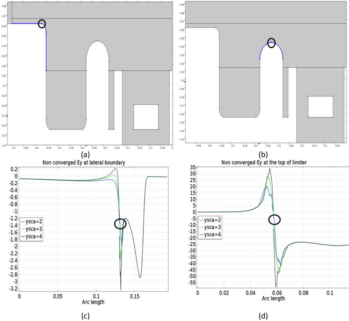
Figure 4.9. (a)-(b) Blue curve Indicates the target boundary while the black circle shows the transition point; (c) Comparison of E_y with three mesh sizes at the boundary in (a). Black circle indicates the transition point; (d) Comparison of E_y with three mesh sizes at the boundary in (b)
