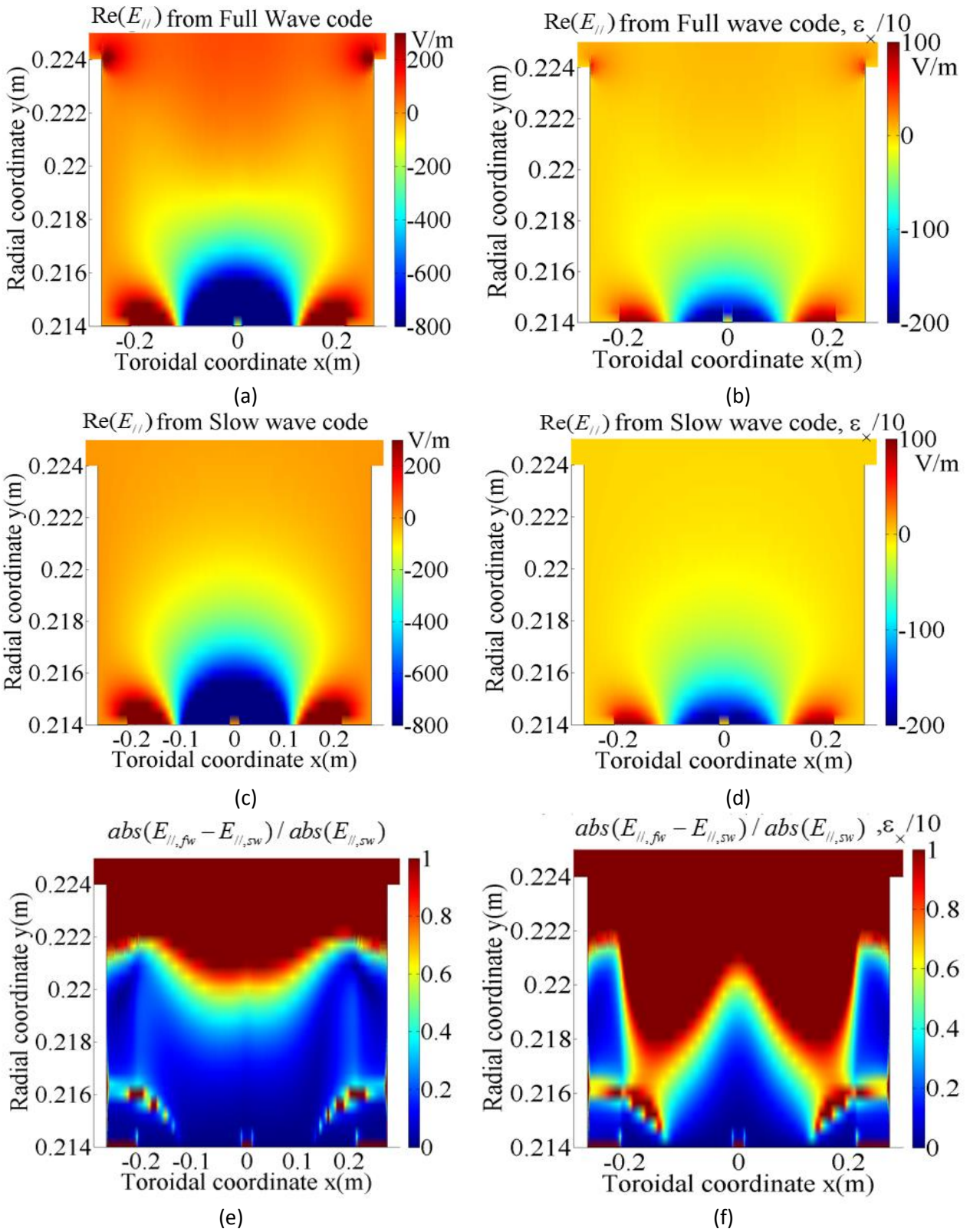
Figure 5.4. Comparison of E_{||} . Left: normal parameters Right: \epsilon_x/10
