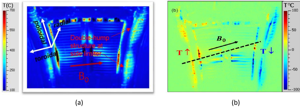
Figure 5.12 (a): infrared picture of active ToreSupra ICRF antenna [Corre 2012] shows a double-hump structure at the side limiters (b) differential IR image from subtraction of two RF pulses, where the RF generator power balance is changed from (50% / 50%) to (63% / 37%)[Colas 2013]
