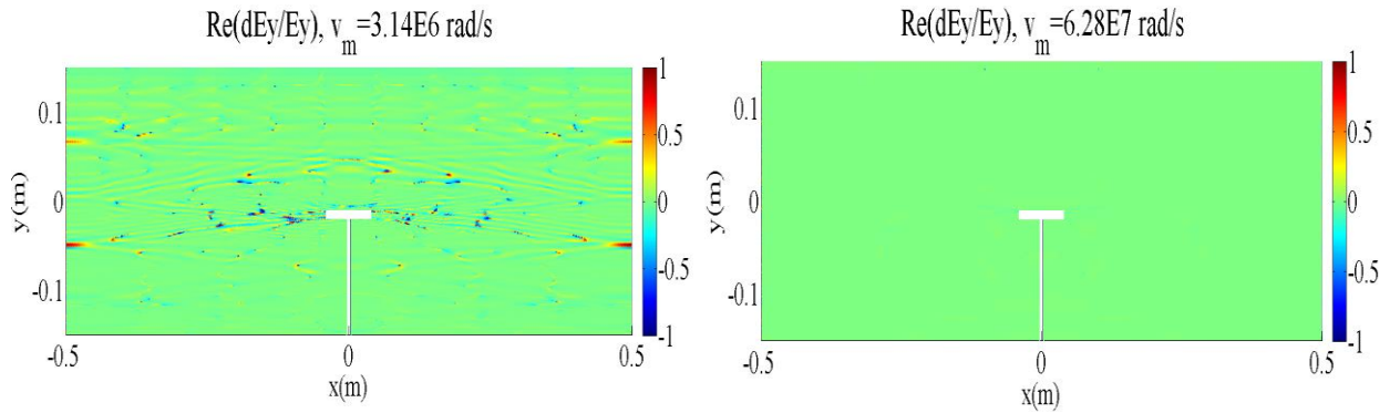
Figure 5.25. Relative variations of E_y of the Helicon wave with different dissipation; dE_y/E_y = (E_y(1mm) - E_y(2mm))/E_y(2mm) ; Left: collision frequency \nu_m = 3.14 \times 10^6 rad/s; Right \nu_m = 6.28 \times 10^7 rad/s
