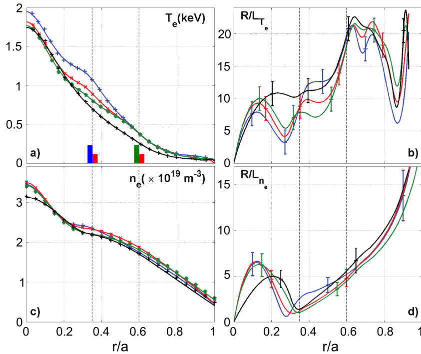
Figure 5.7: Profiles of the electron (a) temperature and (c) density, normalized (b) temperature and (d) density gradients for the discharges shown in table 5.3. These data are computed with CRONOS [Artaud 2010]. In black an Ohmic reference shot is shown.
