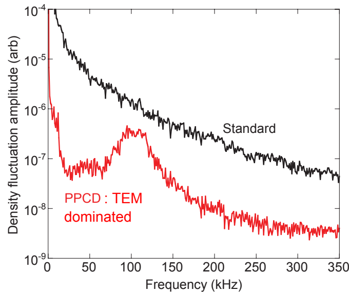
Figure 7.2: measurement made in the reversed field pinch MST in standard plasmas (black) and PPCD plasma dominated by TEM. Reproduced from [Sarff 2015].
