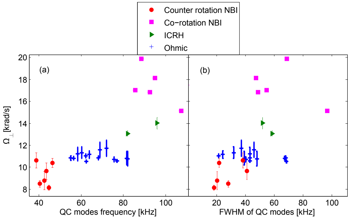
Figure 4.1: TEXTOR measurements of the perpendicular velocity \Omega_{\perp} made at the LFS during the discharges #116494, #116495, #107985-7, #108012, #108824, 116518. (a) shows \Omega_{\perp} as a function of the QC mode frequency and (b) shows \Omega_{\perp} as a function of the frequency width of the QC mode peak.
