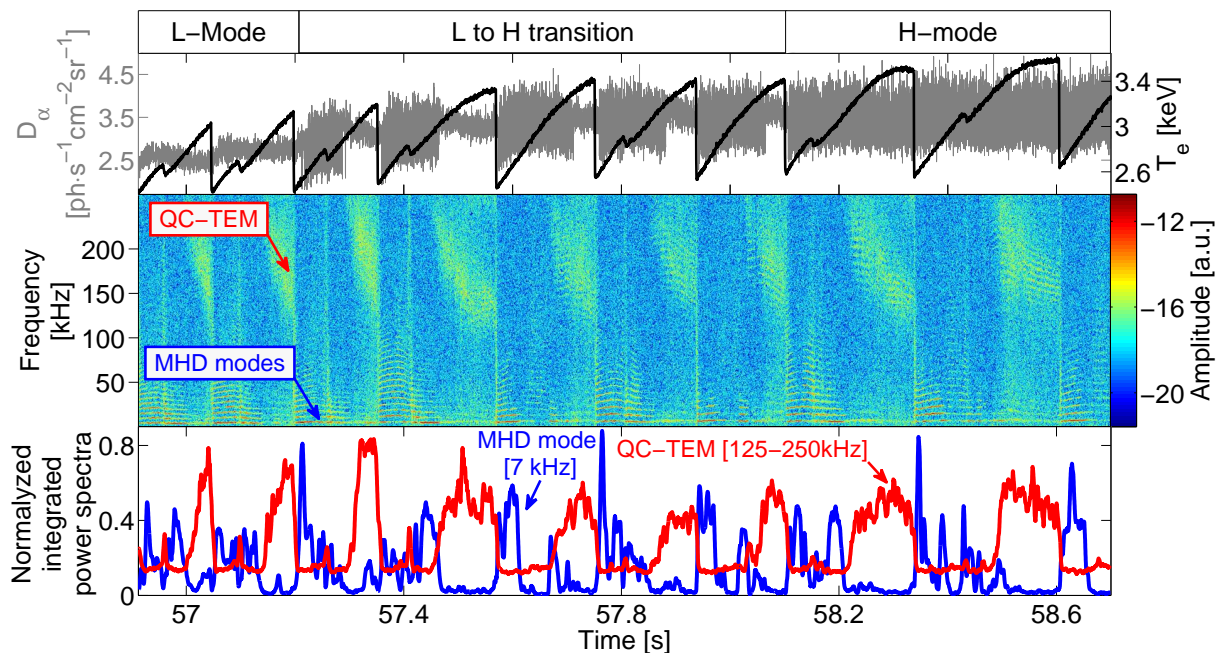
Figure 6.11: JET data showing (a) the electron temperature and the D_\alpha signals, (b) the reflectometry spectrogram and (c) the normalized integrated power spectra.
