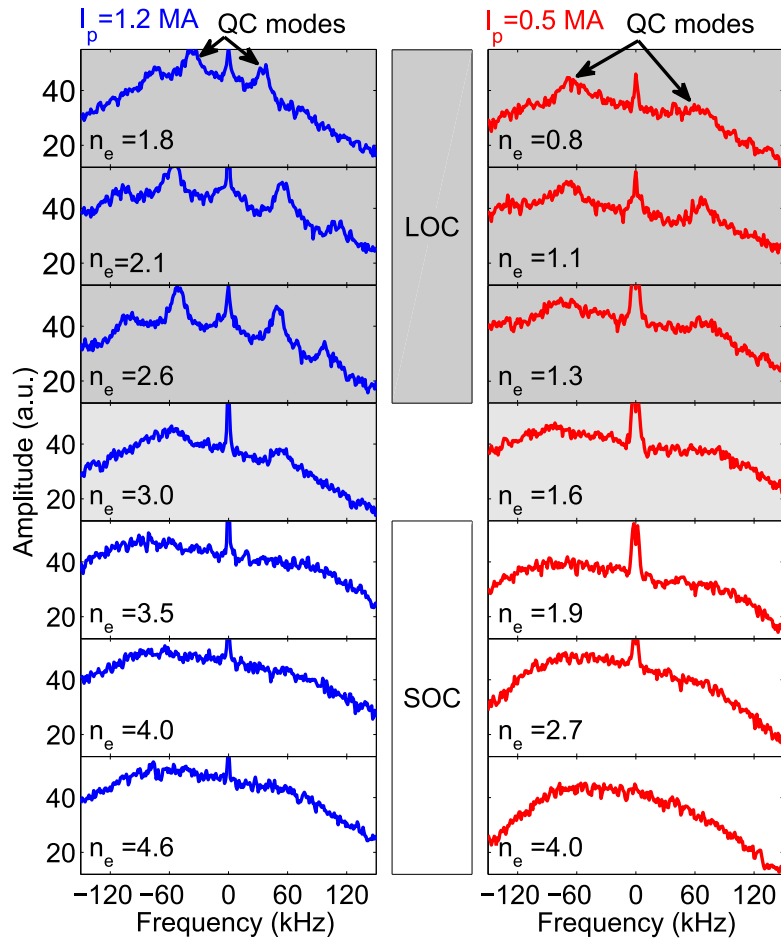
Figure 4.5: Tore Supra reflectometry spectra during the LOC-SOC transitions shown in figure 4.4. The measurements are performed at r/a \approx 0.2 for I_p = 0.5 MA and at r/a \approx 0.3 for I_p \approx 1.2 MA. The spectra correspond to the filled points shown in figure 4.4.
