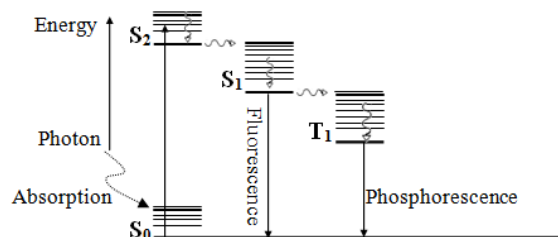
Fig. 13 Jablonski diagram showing fluorescence and phosphorescence.
