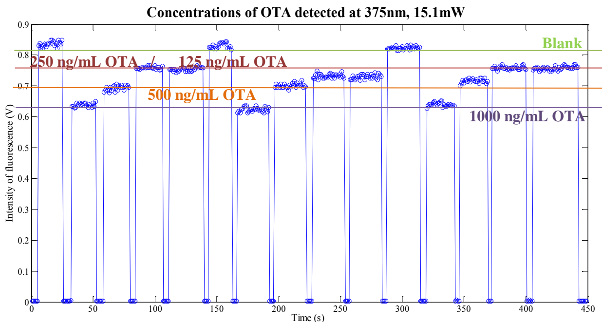
Fig. 53 Concentration of OTA versus the intensity of fluorescence in voltage value.
