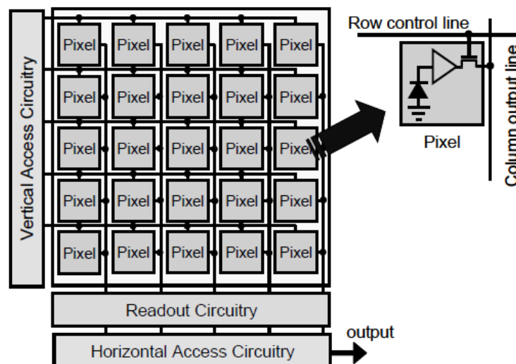
Fig. 14 Architecture of a CMOS image sensor.
