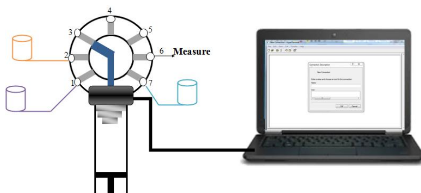
Fig. 34 Representation of a SIA system.
