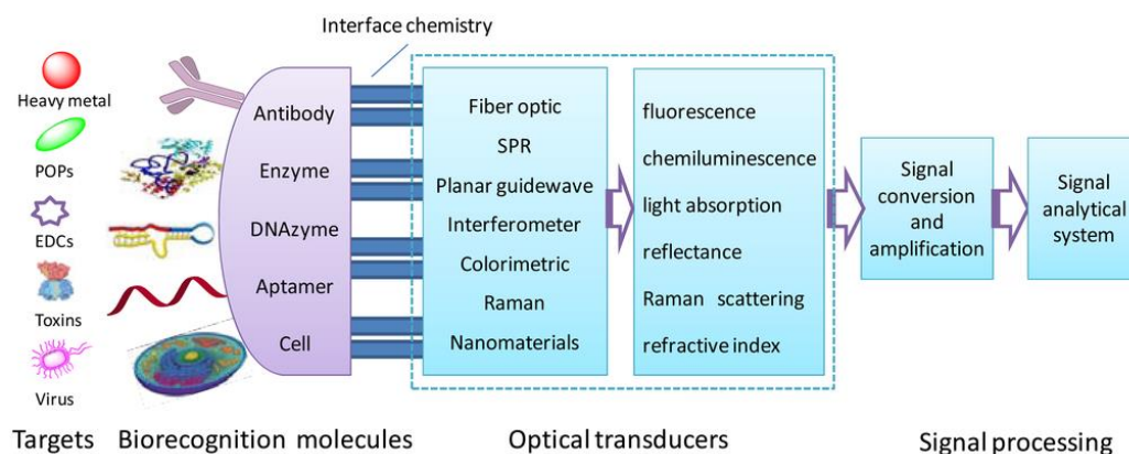
Fig. 11 Schematic of an optical biosensor [99].
