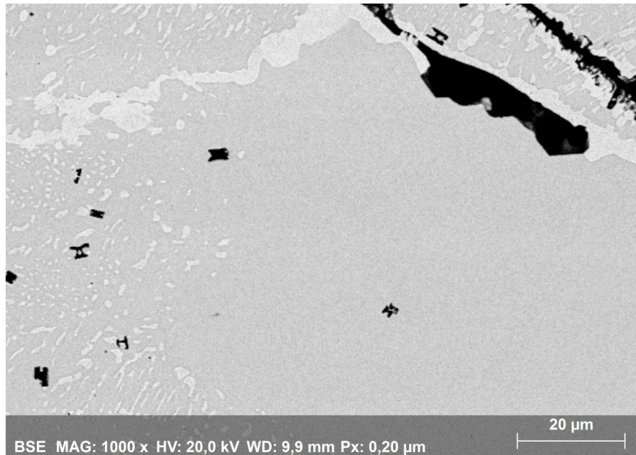
FIGURE 3.13: SEM image of the sample n°34 obtained in BSE mode. The light gray phase (minority) corresponds to the AlIr compound, the darker gray phase (majority) is the new Al 2.4 Ir compound and the black regions are holes.
