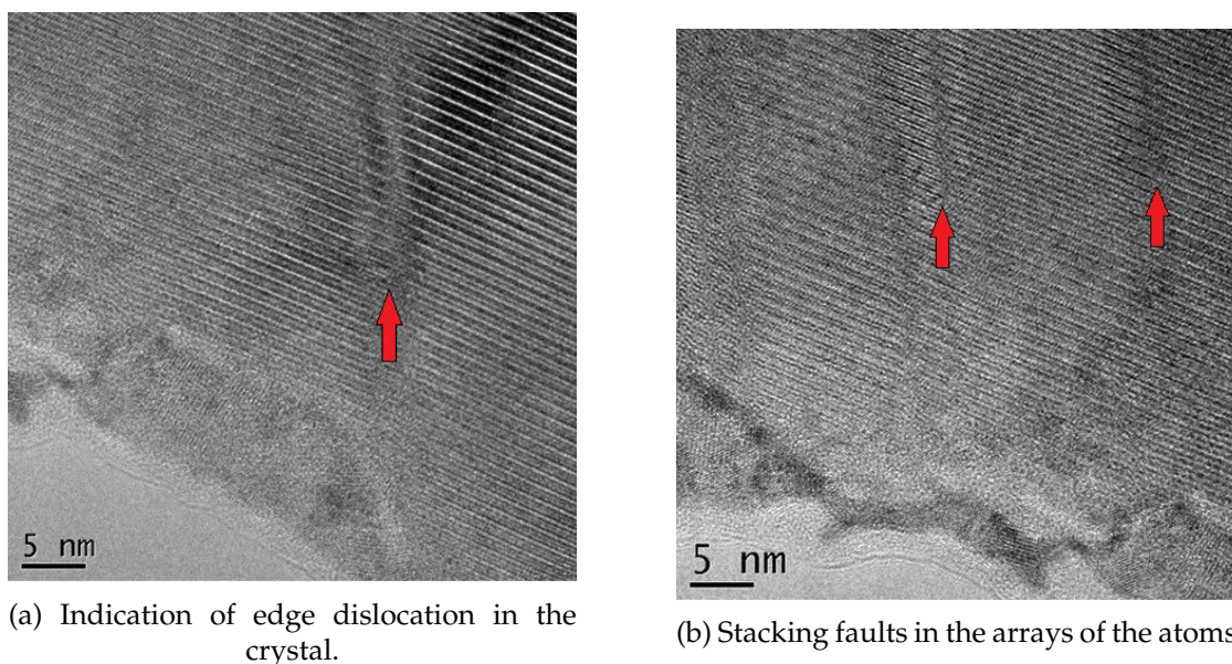
FIGURE 3.15: Typical TEM images of the sample n°34.
