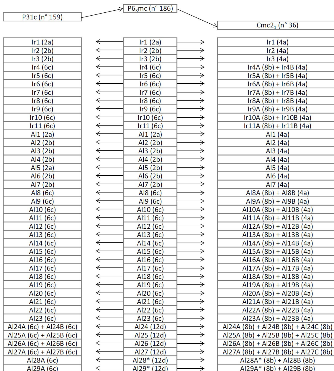
FIGURE 3.20: Atomic and Wyckoff positions generated after splitting the P6_3mc space group into the P31c and Cmc2_1 space groups. The positions marked by a star (*) are half occupied.
