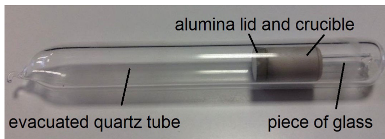
FIGURE 2.2: A sample inside an alumina crucible sealed in an evacuated quartz tube.
