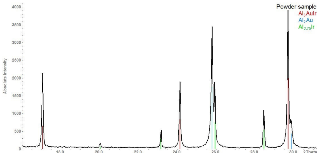
FIGURE 2.8: One section of a PXRD pattern of an Al-Au-Ir alloy, indexed with the three identified phases.
